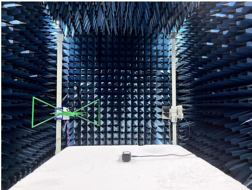
Radiated Test Above 1GHz Lab A
