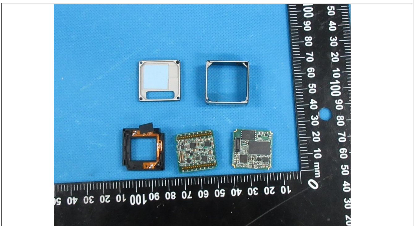
Details of: Internal view 23
