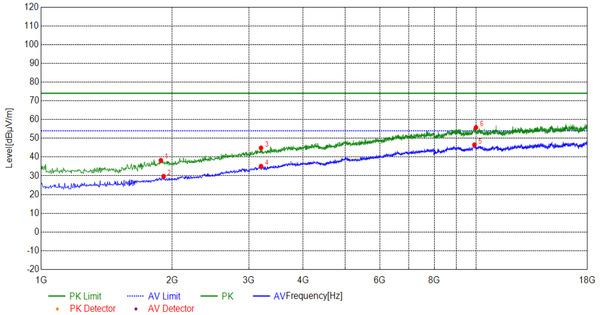
(Plot N: Test Antenna Vertical 1G – 18G)
