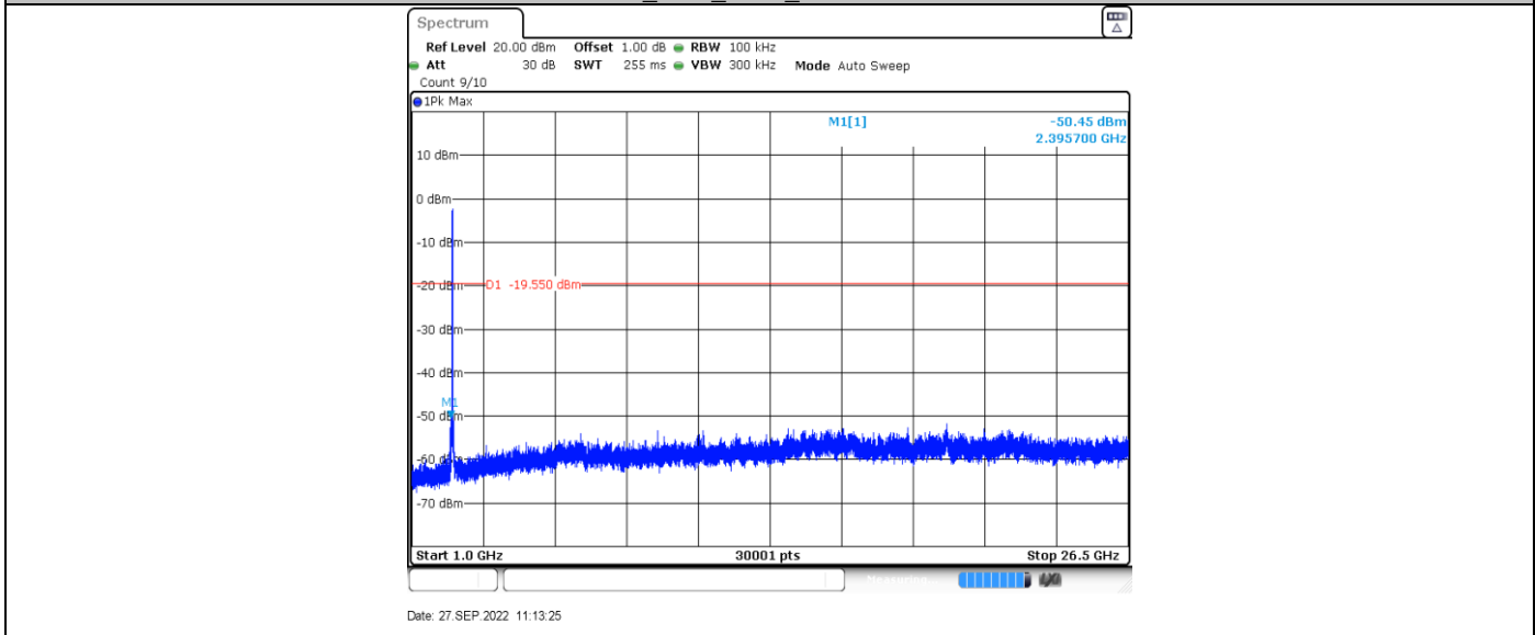
11G_Ant1_2462_0~Reference
