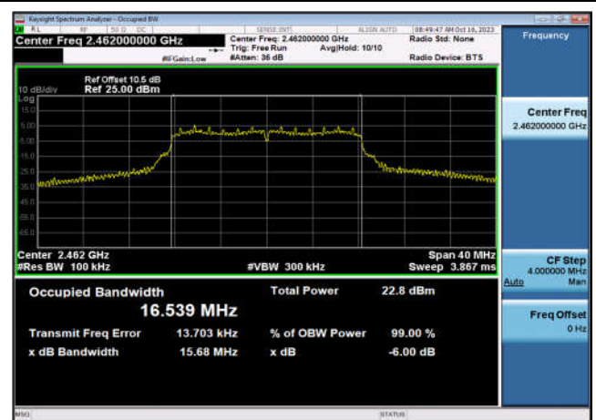
6dB Bandwidth-802.11g,2462MHz,Ant0
