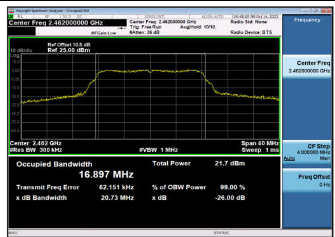
99% Bandwidth-802.11g,2462MHz,Ant0
