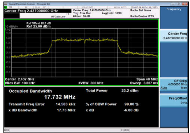
6dB Bandwidth-802.11n(HT20),2437MHz ,Ant0
