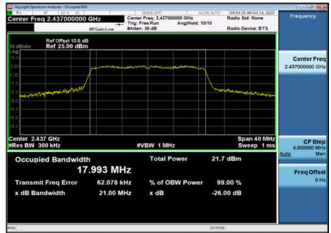
99% Bandwidth-802.11n(HT20),2437MHz ,Ant0
