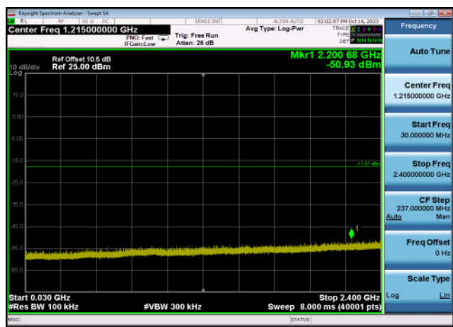
Conducted Emission: GFSK,2441,DH5 ,30MHz~2400MHz
