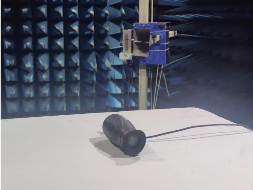
Radiated emissions spurious (Above 1GHz)
