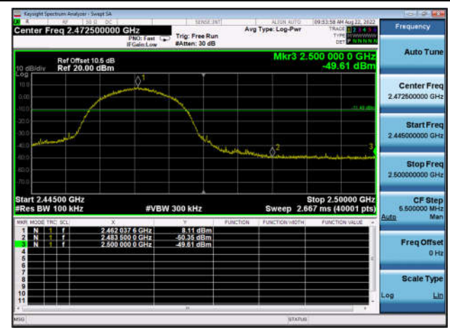
,Plot 2,Band Edge-802.11b,2462MHz ,Ant0
