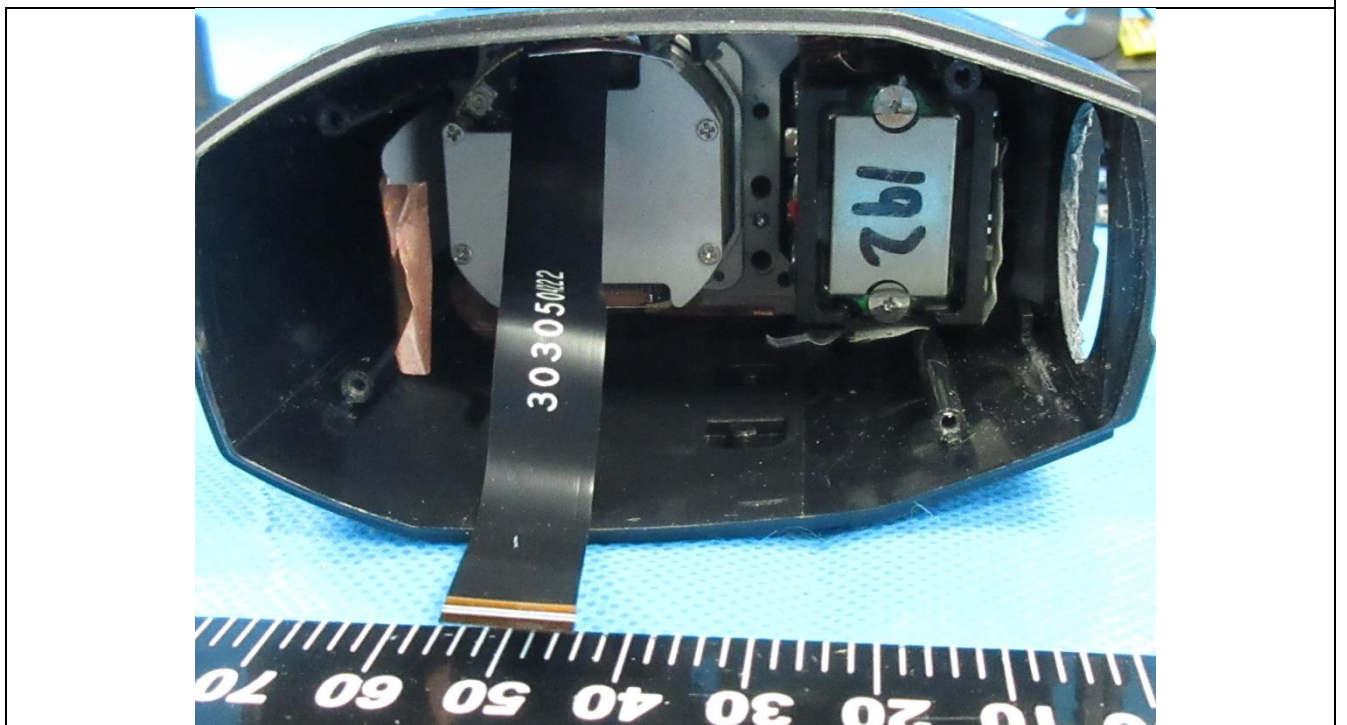
Details of: Internal view 6 of main unit
