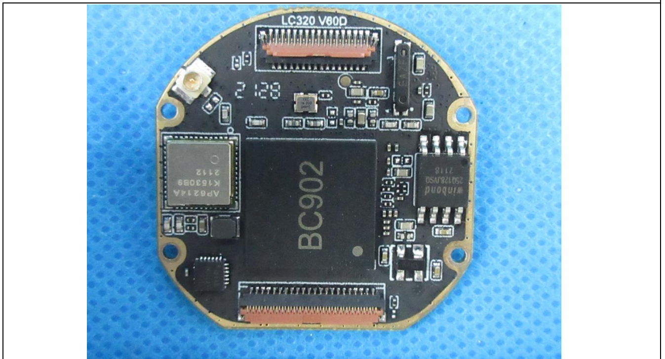
Details of: PCB view 9 of main unit
