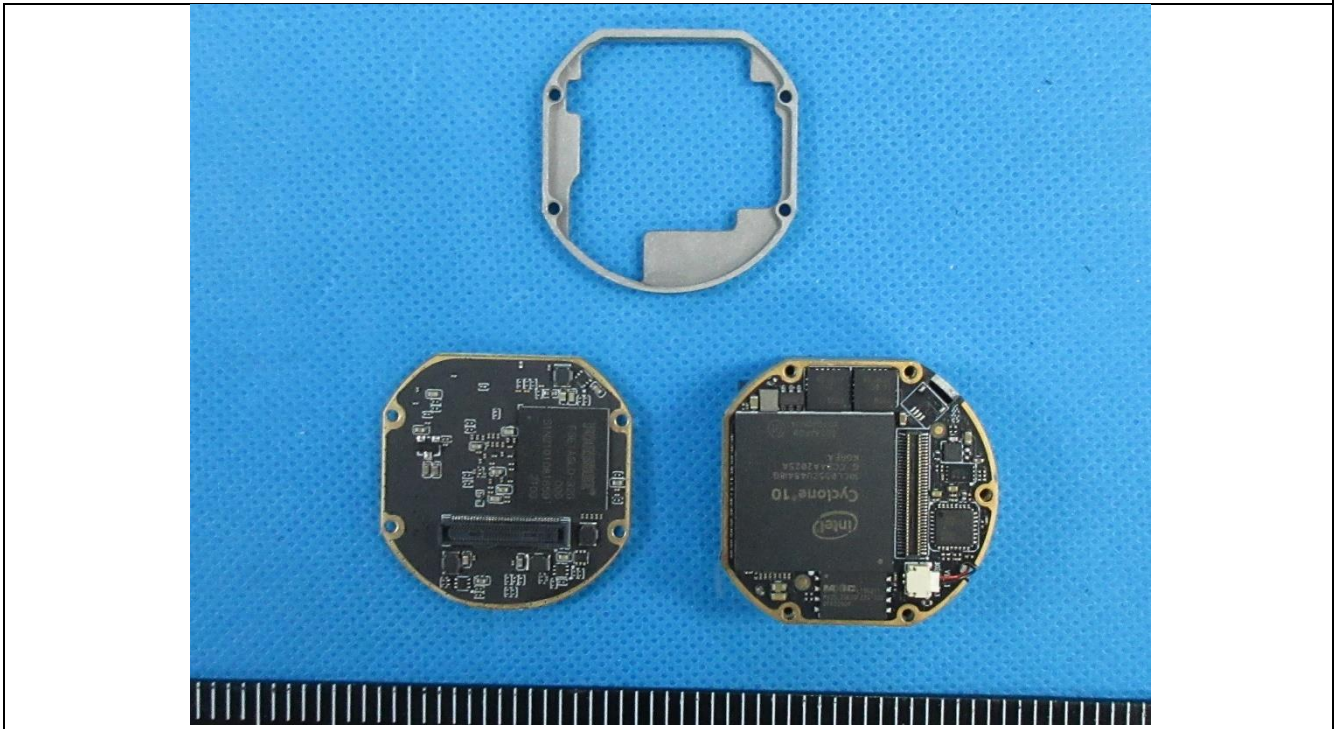
Details of: PCB view 7 of main unit
