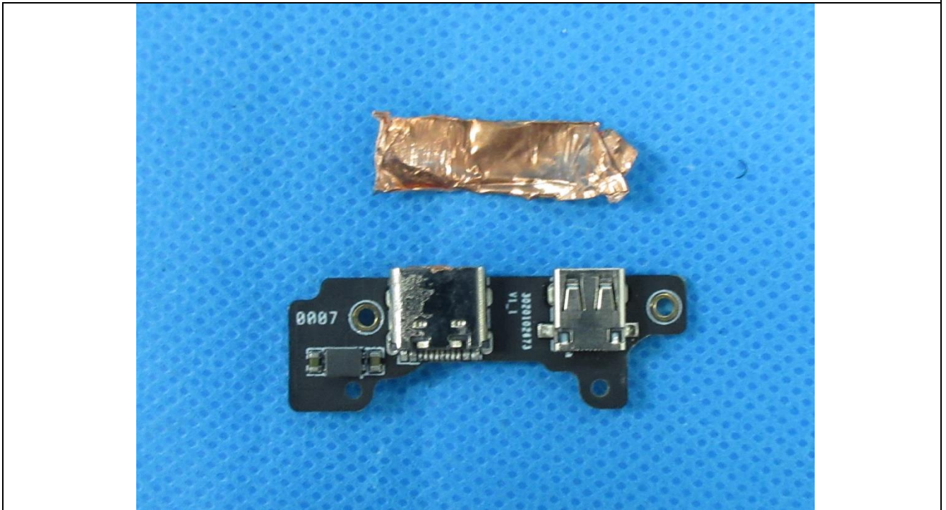
Details of: PCB view 4 of main unit
