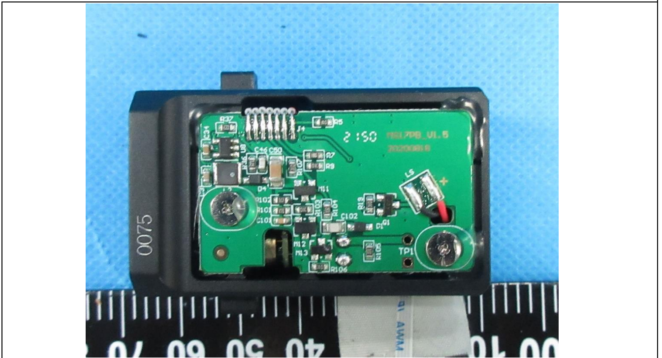
Details of: PCB view 14 of main unit
