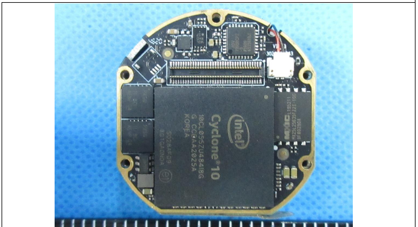
Details of: PCB view 10 of main unit
