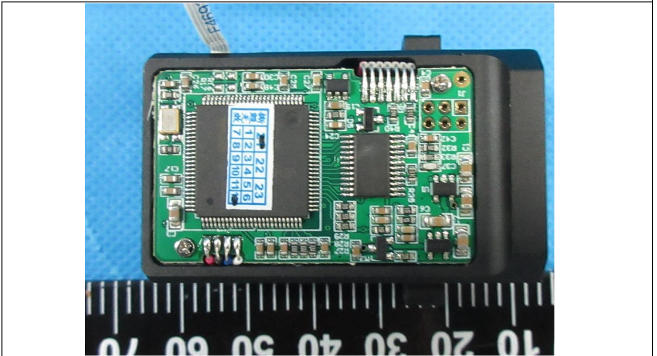
Details of: PCB view 16 of main unit
