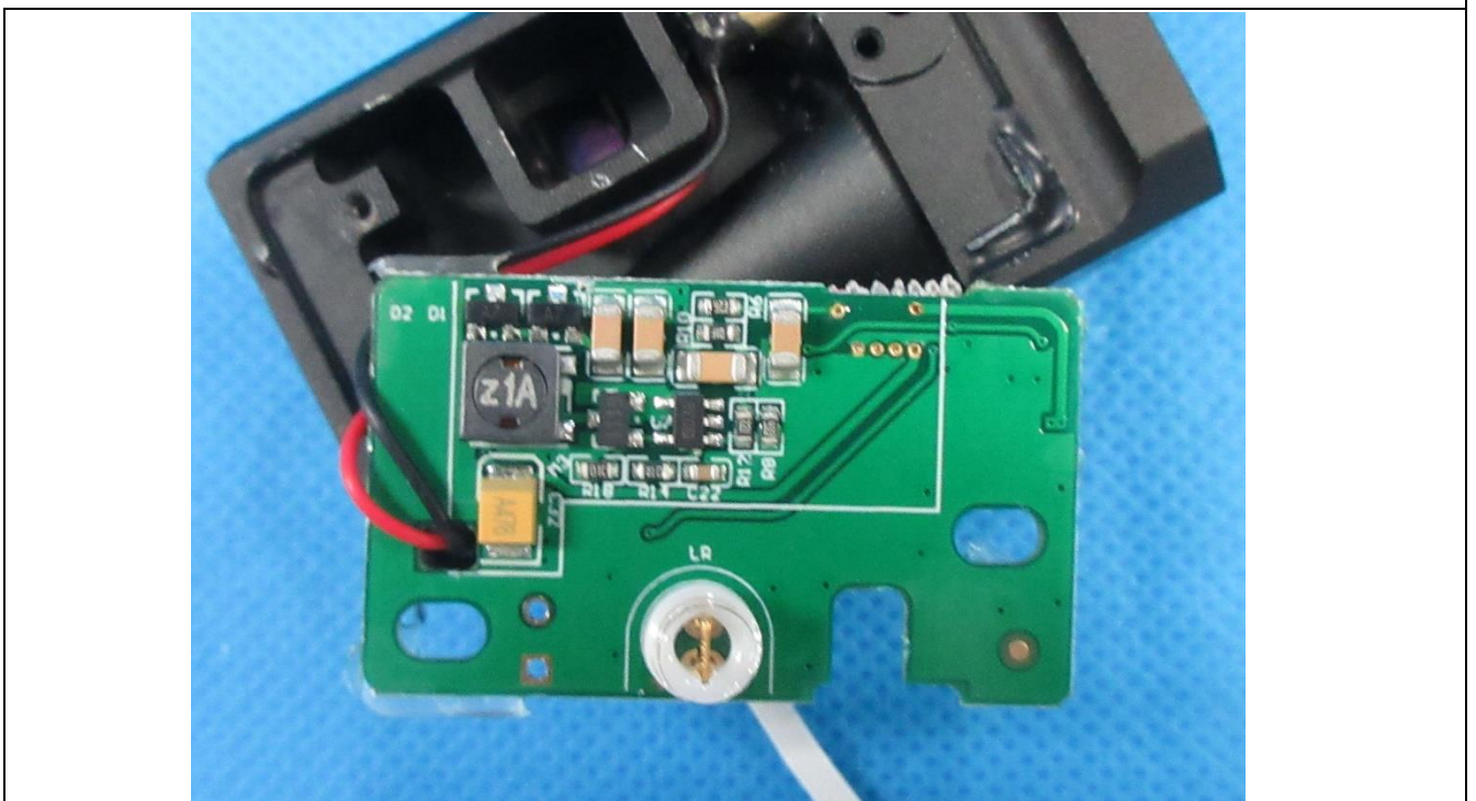
Details of: PCB view 15 of main unit
