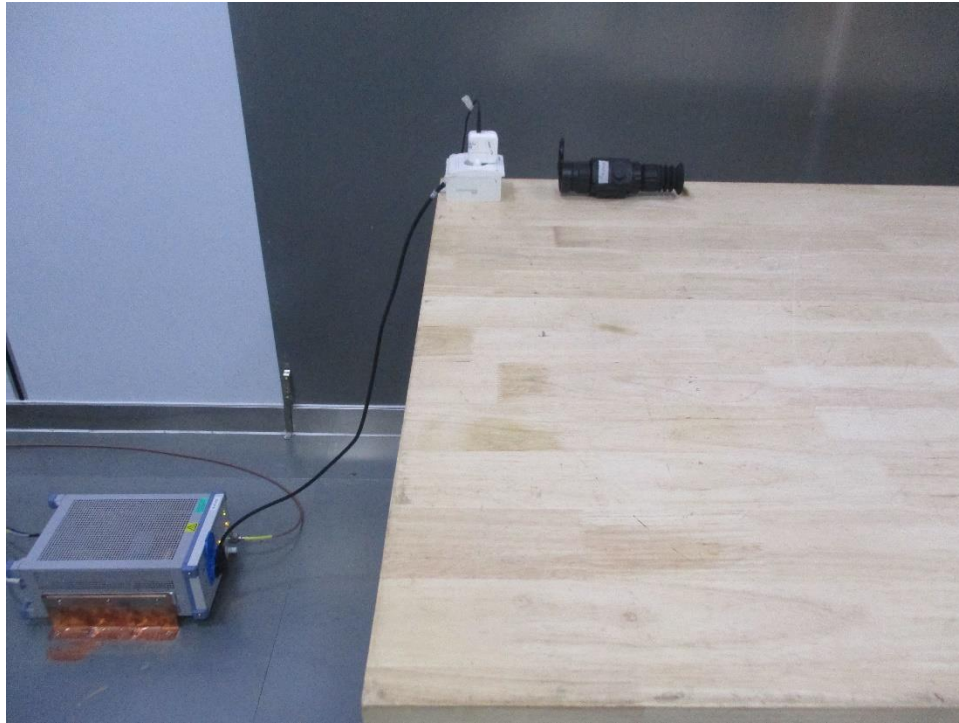
Conducted Disturbance Emissions on AC main
