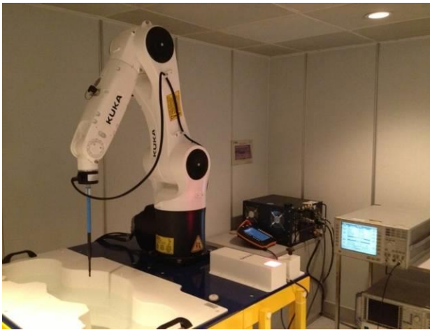
Photo 1: Measurement System SATIMO
