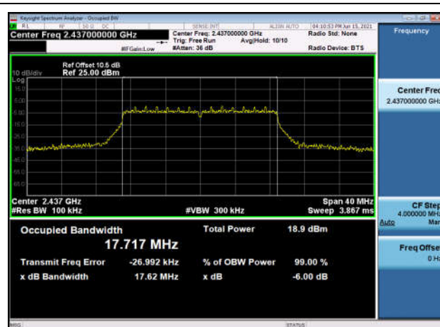
6dB Bandwidth-802.11n(HT20),2437MHz
