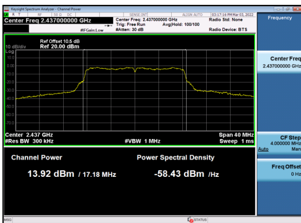
Output Power-802.11g,2437MHz,Ant0
