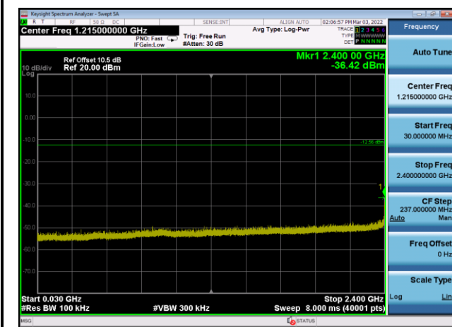
Plot 3,30MHz~2400MHz-802.11b,2462MHz
