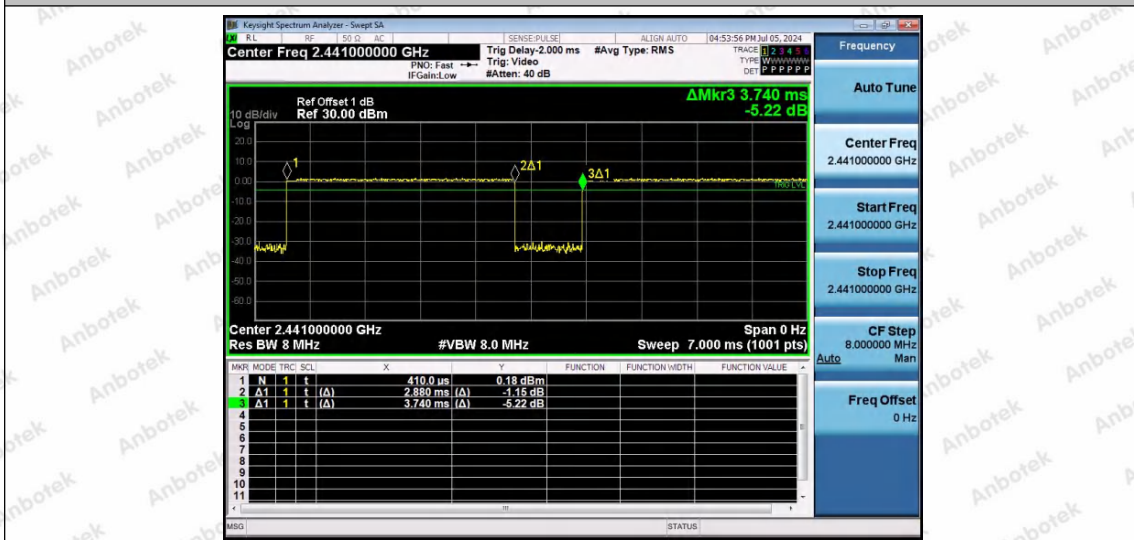
NTNV-3DH5-Ant1-2441
