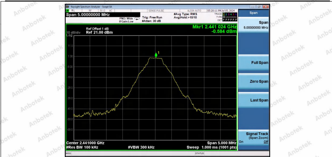
DH5-Ant1-2441-0~Reference-PASS
