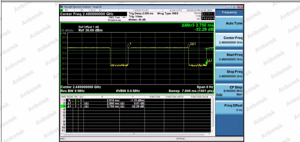
NTNV-3DH5-Ant1-2480
