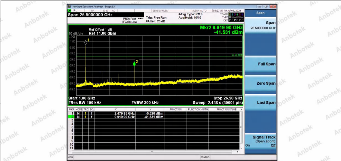
3DH5-Ant1-2480-1000~26500-PASS
