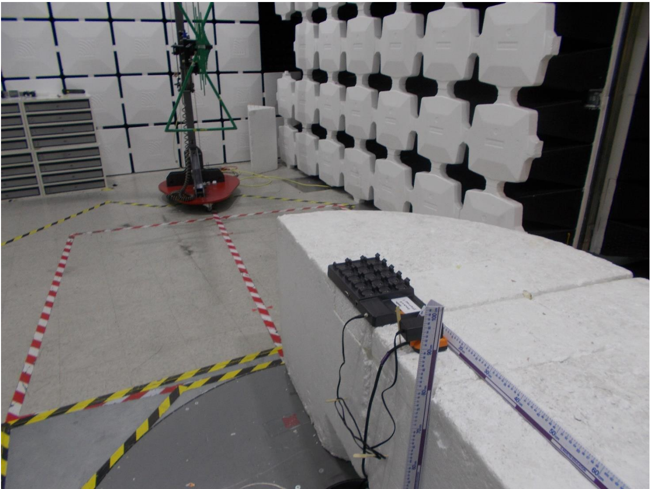
Radiated emissions 30MHz to 1GHz
