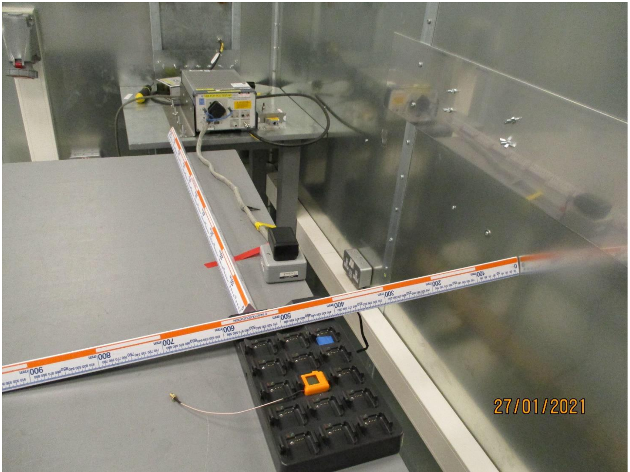
Mains conducted emissions
