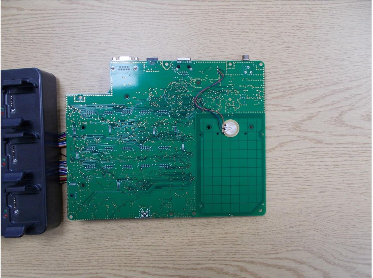
Track Side
