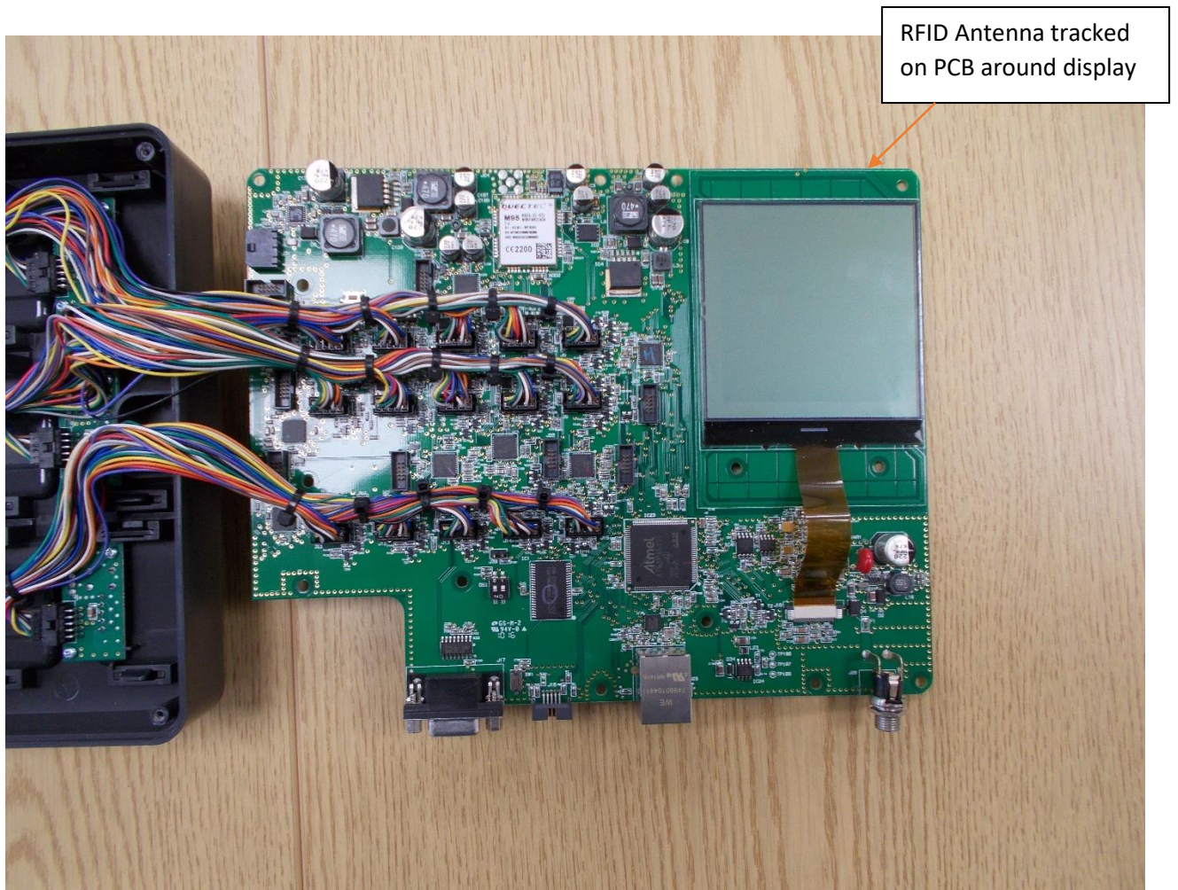
Component side
