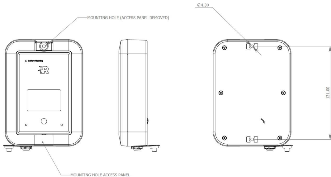
Figure 6 - R-LINKBeacon
