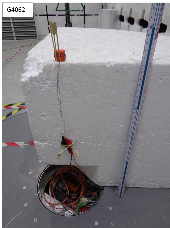
EUT Setup – Radiated emissions 30MHz to 1GHz
