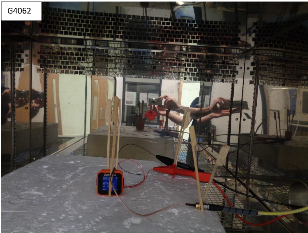
EUT Setup – Stability over temperature 13.56MHz
