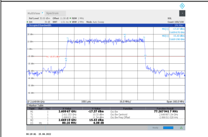
1-N41-PC2-30-80-H-5-DFT-PI/2BPSK-Outer_Full-216@0-Ant1-77.268-80.160-≤80-PASS
