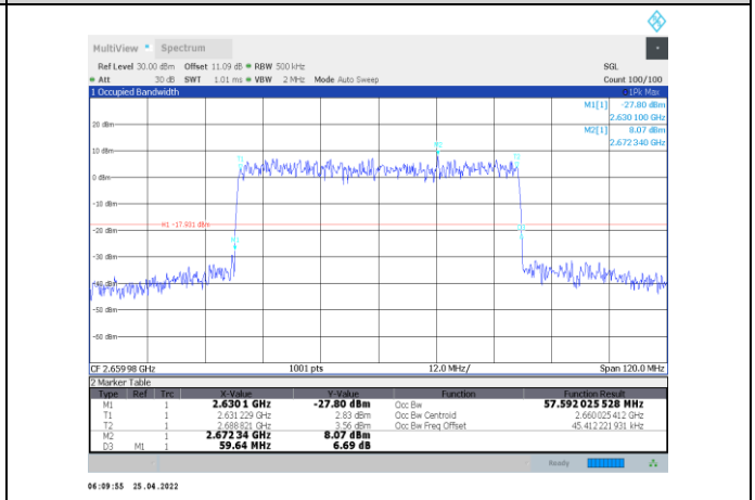
1-N41-PC2-30-60-H-4-CP-256QAM-Outer_Full-162@0-Ant 1-57.592-59.640-≤60-PASS
