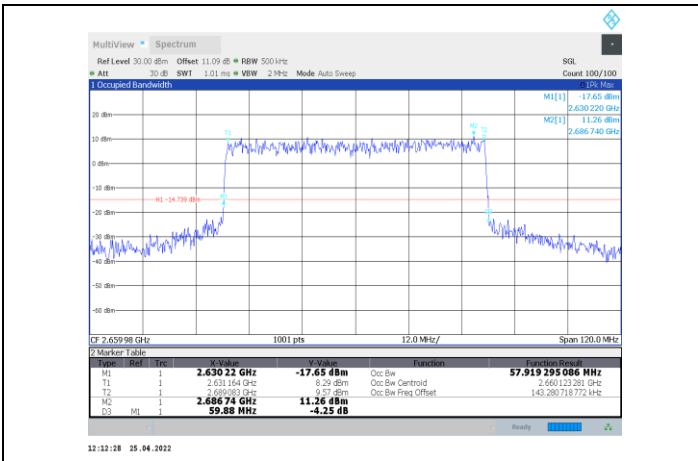
1-N41-PC2-30-60-H-1-CP-QPSK-Outer_Full-162@0-Ant 1-57.919-59.880-≤60-PASS
