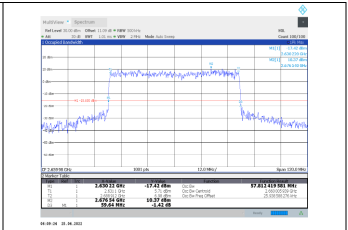
1-N41-PC2-30-60-H-2-CP-16QAM-Outer_Full-162@0-Ant 1-57.812-59.640-≤60-PASS
