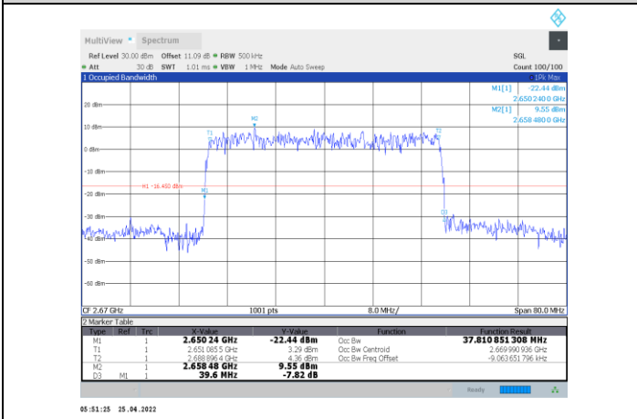
1-N41-PC2-30-40-H-3-CP-64QAM-Outer_Full-106@0-Ant1 nt1-37.811-39.600-≤40-PASS
