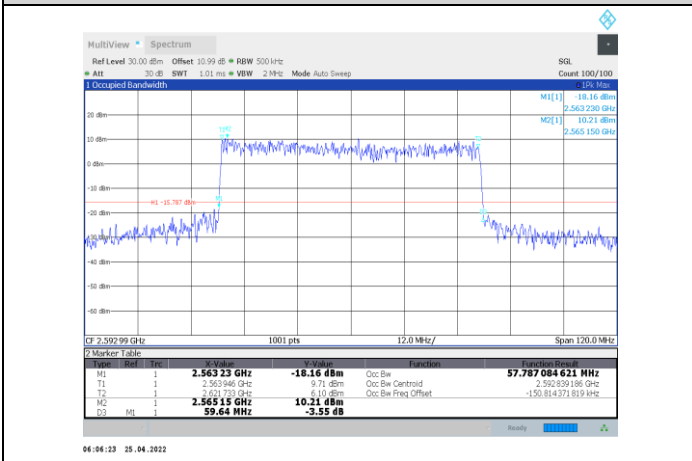
1-N41-PC2-30-60-M-2-CP-16QAM-Outer_Full-162@0-A nt1-57.787-59.640-≤60-PASS
