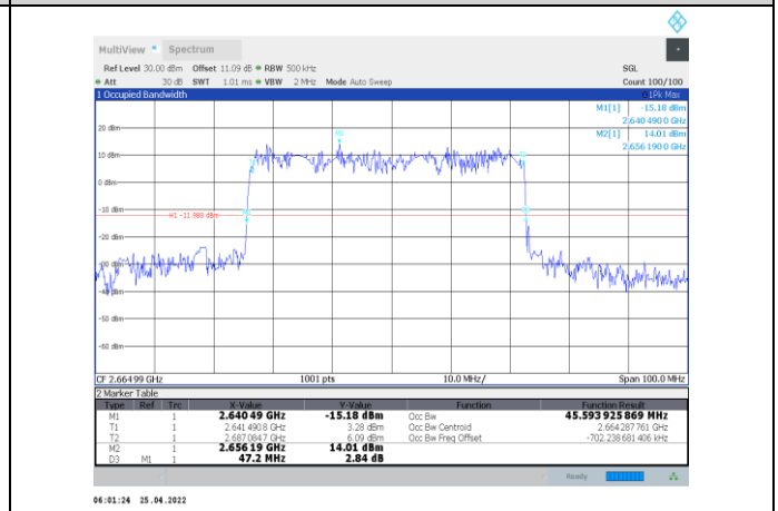
1-N41-PC2-30-50-H-6-DFT-QPSK-Outer_Full-128@0-Ant 1-45.594-47.200-≤50-PASS
