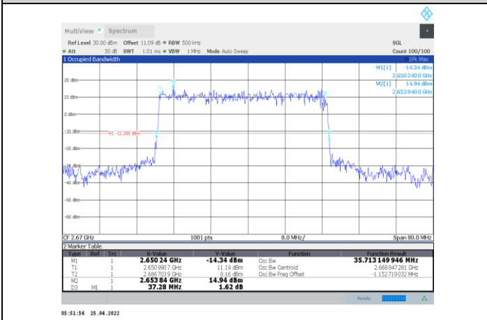
1-N41-PC2-30-40-H-5-DFT-PI/2BPSK-Outer_Full-100@0-Ant1 0-Ant1-35.713-37.280-≤40-PASS
