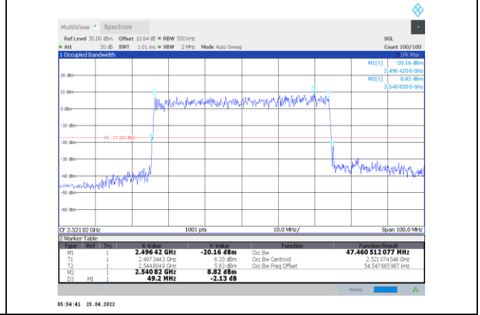
1-N41-PC2-30-50-L-4-CP-256QAM-Outer_Full-133@0- Ant1-47.461-49.200-≤50-PASS
