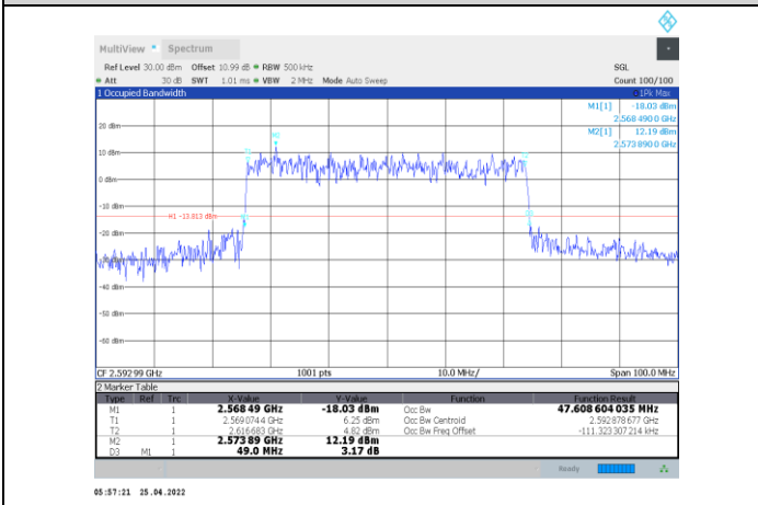
1-N41-PC2-30-50-M-2-CP-16QAM-Outer_Full-133@0-Ant1-47.609-49.000-≤50-PASS
