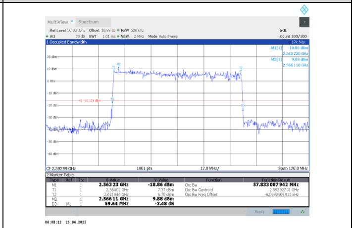
1-N41-PC2-30-60-M-9-DFT-256QAM-Outer_Full-162@0-Ant1-57.833-59.640-≤60-PASS
