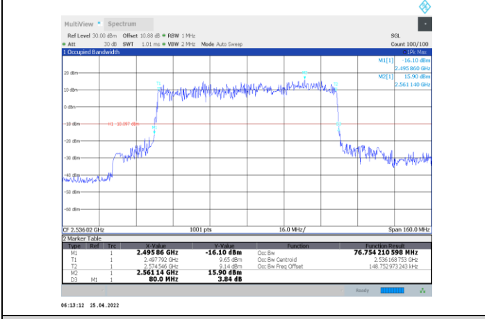
1-N41-PC2-30-80-L-5-DFT-PI/2BPSK-Outer_Full-216@0 -Ant1-76.754-80.000-≤80-PASS
