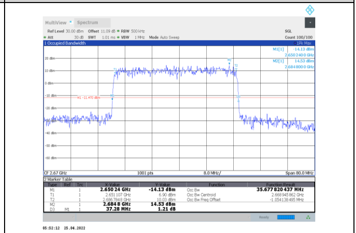
1-N41-PC2-30-40-H-6-DFT-QPSK-Outer_Full-100@0-Ant1 Ant1-35.678-37.280-≤40-PASS
