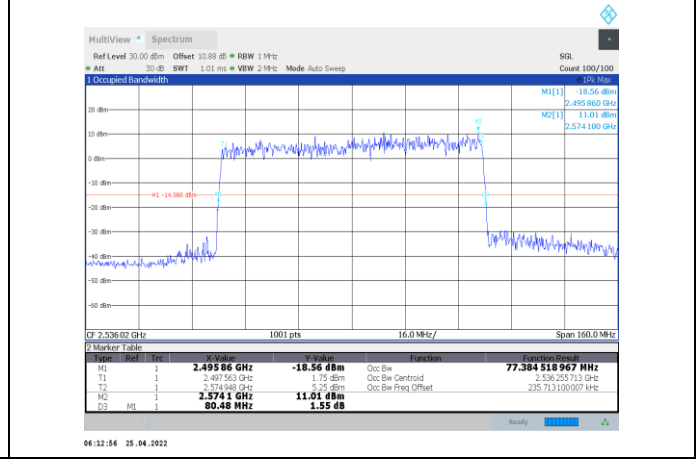
1-N41-PC2-30-80-L-4-CP-256QAM-Outer_Full-217@0- Ant1-77.385-80.480-≤80-PASS
