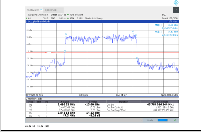
1-N41-PC2-30-50-L-5-DFT-PI/2BPSK-Outer_Full-128@0 -Ant1-45.784-47.300-≤50-PASS
