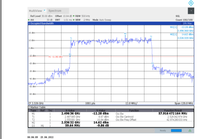
1-N41-PC2-30-60-L-5-DFT-PI/2BPSK-Outer_Full-162@0 -Ant1-57.916-59.640-≤60-PASS
