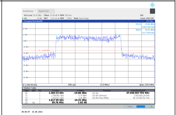
1-N41-PC2-30-60-M-1-CP-QPSK-Outer_Full-162@0-An t1-57.951-59.760-≤60-PASS
