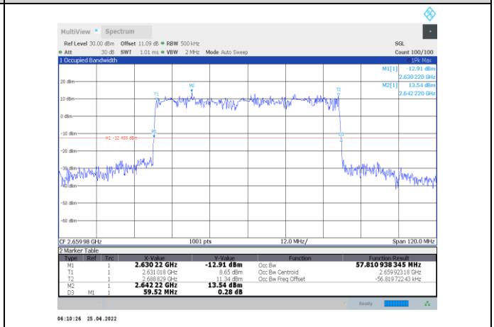
1-N41-PC2-30-60-H-6-DFT-QPSK-Outer_Full-162@0-Ant 1-57.811-59.520-≤60-PASS
