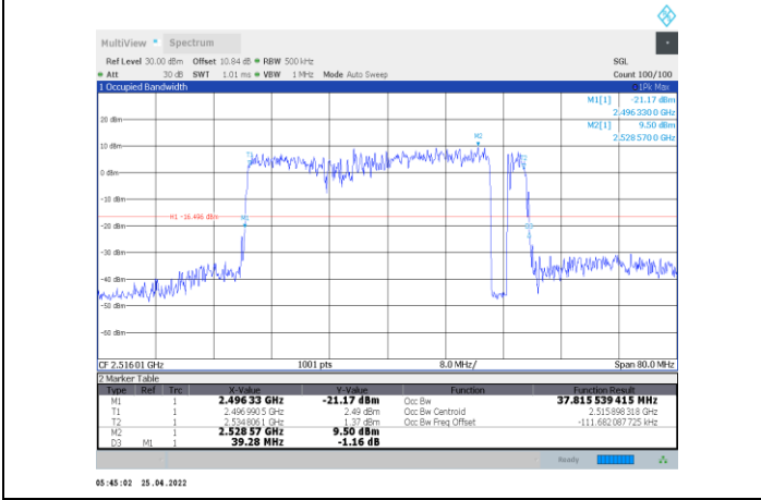
1-N41-PC2-30-40-L-3-CP-64QAM-Outer_Full-106@0-An t1-37.816-39.280-≤40-PASS
