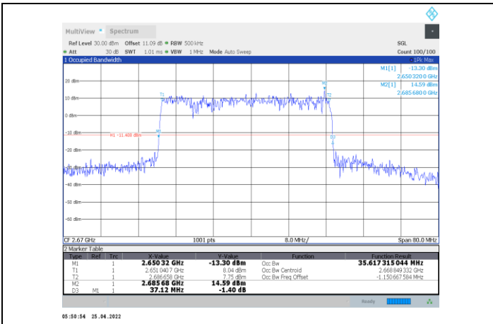
1-N41-PC2-30-40-H-1-CP-QPSK-Outer_Full-106@0-Ant 1-35.617-37.120-≤40-PASS
