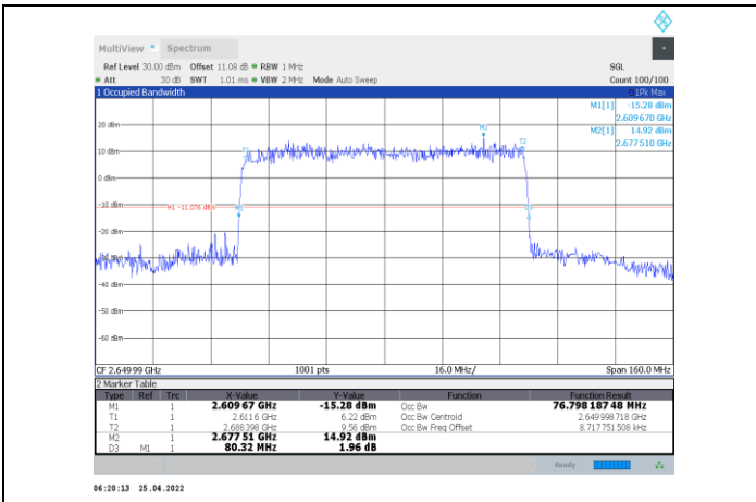
1-N41-PC2-30-80-H-7-DFT-16QAM-Outer_Full-216@0-Ant1-76.798-80.320-≤80-PASS
