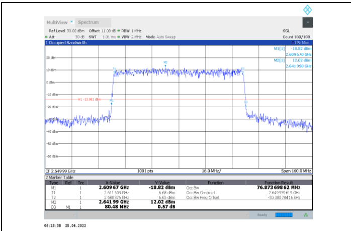
1-N41-PC2-30-80-H-1-CP-QPSK-Outer_Full-217@0-Ant 1-76.874-80.480-≤80-PASS
