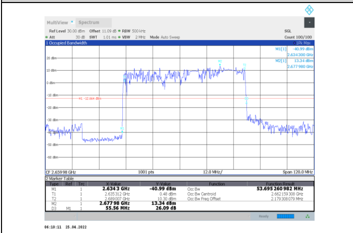
1-N41-PC2-30-60-H-5-DFT-PI/2BPSK-Outer_Full-162@0-Ant 1-53.695-55.560-≤60-PASS
