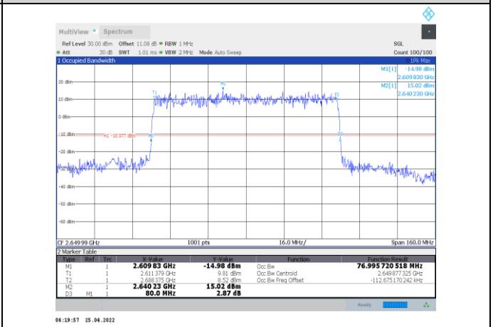
1-N41-PC2-30-80-H-6-DFT-QPSK-Outer_Full-216@0-Ant1-76.996-80.000-≤80-PASS
