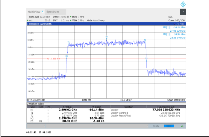
1-N41-PC2-30-80-L-3-CP-64QAM-Outer_Full-217@0-An t1-77.038-80.320-≤80-PASS
