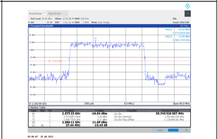
1-N41-PC2-30-40-M-9-DFT-256QAM-Outer_Full-100@0-Ant1-35.746-37.440-≤40-PASS
