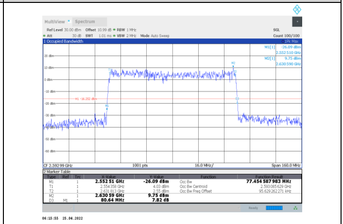
1-N41-PC2-30-80-M-3-CP-64QAM-Outer_Full-217@0-A nt1-77.455-80.640-≤80-PASS
