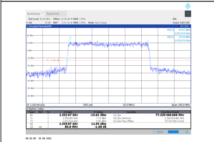
1-N41-PC2-30-80-M-2-CP-16QAM-Outer_Full-217@0-A nt1-77.339-80.800-≤80-PASS
