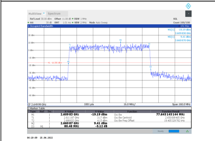
1-N41-PC2-30-80-H-3-CP-64QAM-Outer_Full-217@0-Ant1-77.645-80.480-≤80-PASS
