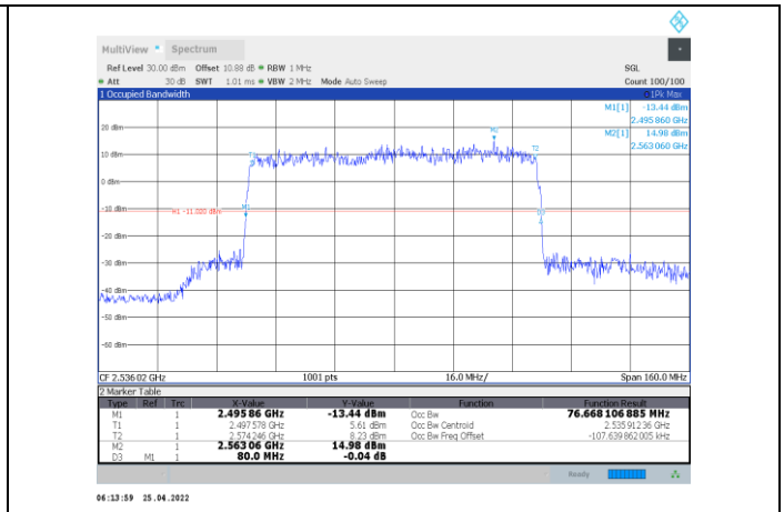
1-N41-PC2-30-80-L-8-DFT-64QAM-Outer_Full-216@0-Ant1-76.668-80.000-≤80-PASS
