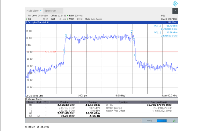
1-N41-PC2-30-40-L-5-DFT-PI/2BPSK-Outer_Full-100@0 -Ant1-35.766-37.280-≤40-PASS
