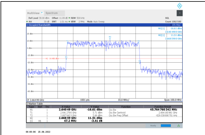
1-N41-PC2-30-50-H-1-CP-QPSK-Outer_Full-133@0-Ant 1-45.765-47.200-≤50-PASS
