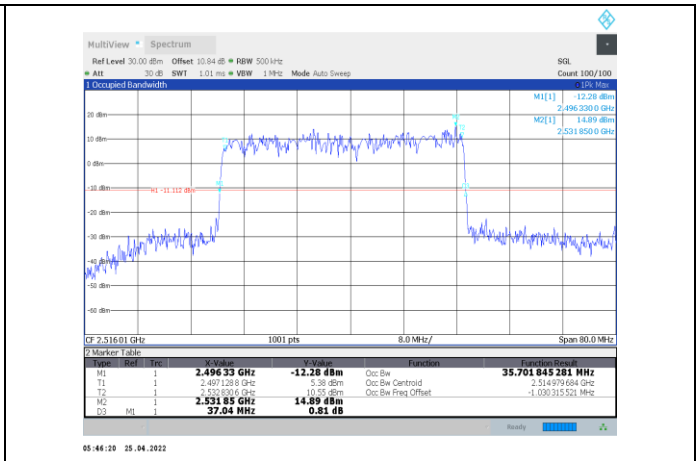
1-N41-PC2-30-40-L-8-DFT-64QAM-Outer_Full-100@0-Ant1-35.702-37.040-≤40-PASS
