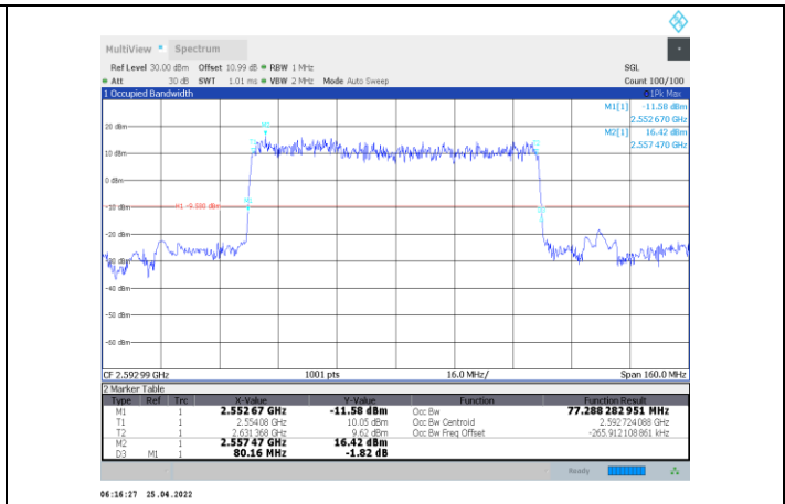
1-N41-PC2-30-80-M-5-DFT-PI/2BPSK-Outer_Full-216@0-Ant1-77.288-80.160-≤80-PASS
