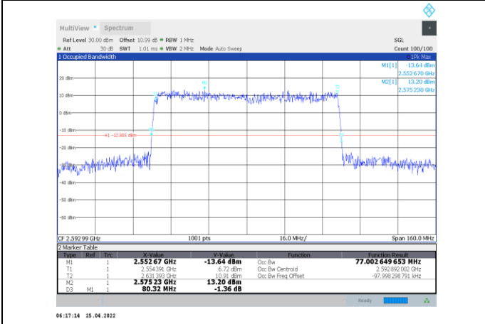
1-N41-PC2-30-80-M-8-DFT-64QAM-Outer_Full-216@0-Ant1-77.003-80.320-≤80-PASS
