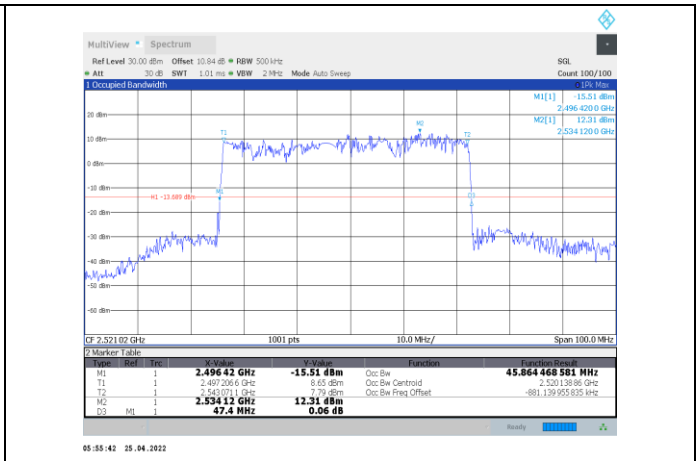
1-N41-PC2-30-50-L-8-DFT-64QAM-Outer_Full-128@0-Ant1-45.864-47.400-≤50-PASS
