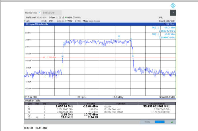
1-N41-PC2-30-40-H-9-DFT-256QAM-Outer_Full-100@0-Ant1-35.46-37.200-≤40-PASS
