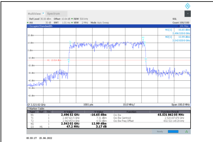
1-N41-PC2-30-50-L-7-DFT-16QAM-Outer_Full-128@0-Ant1-45.532-47.200-≤50-PASS
