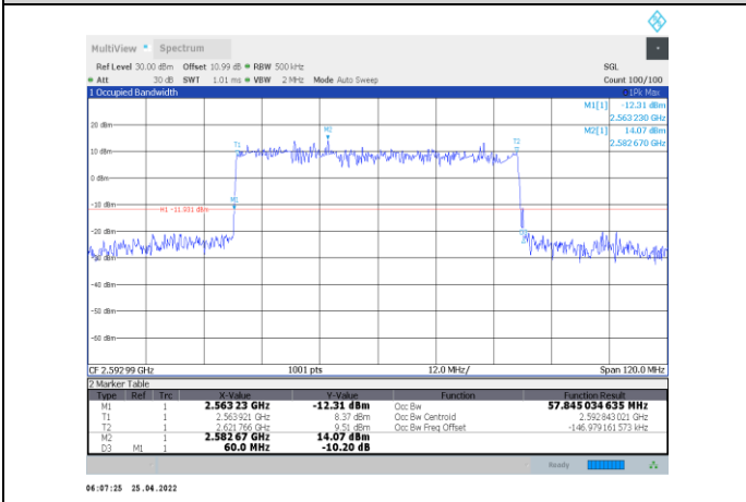
1-N41-PC2-30-60-M-6-DFT-QPSK-Outer_Full-162@0-Ant1-57.845-60.000-≤60-PASS
