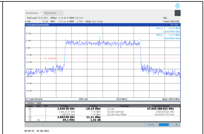
1-N41-PC2-30-50-H-2-CP-16QAM-Outer_Full-133@0-Ant 1-47.64-49.200-≤50-PASS
