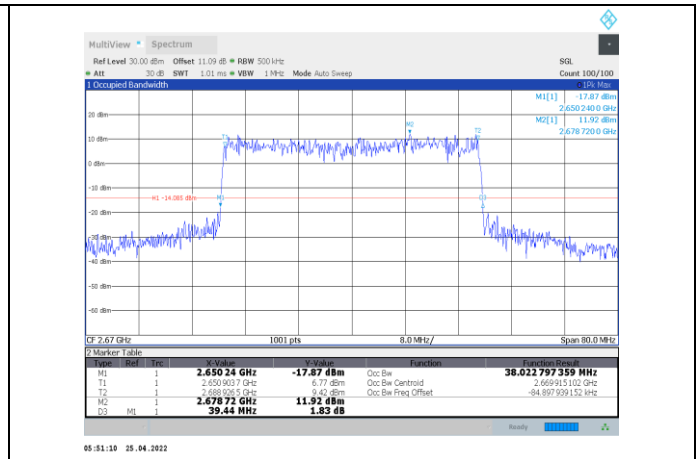
1-N41-PC2-30-40-H-2-CP-16QAM-Outer_Full-106@0-Ant1 -Ant1-38.023-39.440-≤40-PASS
