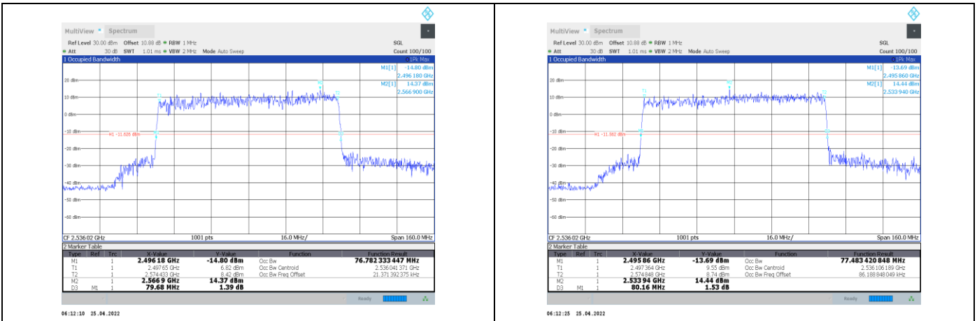
1-N41-PC2-30-80-L-1-CP-QPSK-Outer_Full-217@0-Ant 1-76.782-79.680-≤80-PASS
