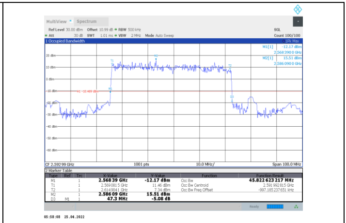
1-N41-PC2-30-50-M-5-DFT-PI/2BPSK-Outer_Full-128@0-Ant1-45.823-47.300-≤50-PASS
