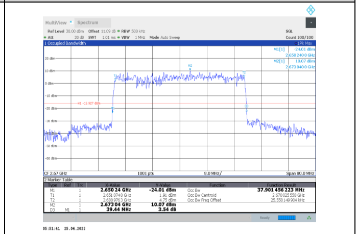
1-N41-PC2-30-40-H-4-CP-256QAM-Outer_Full-106@0-Ant1 -Ant1-37.901-39.440-≤40-PASS
