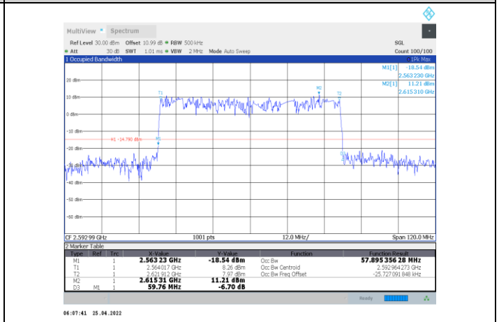
1-N41-PC2-30-60-M-7-DFT-16QAM-Outer_Full-162@0-Ant1-57.895-59.760-≤60-PASS
