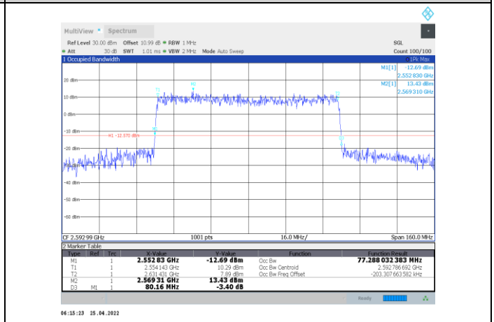
1-N41-PC2-30-80-M-1-CP-QPSK-Outer_Full-217@0-An t1-77.288-80.160-≤80-PASS
