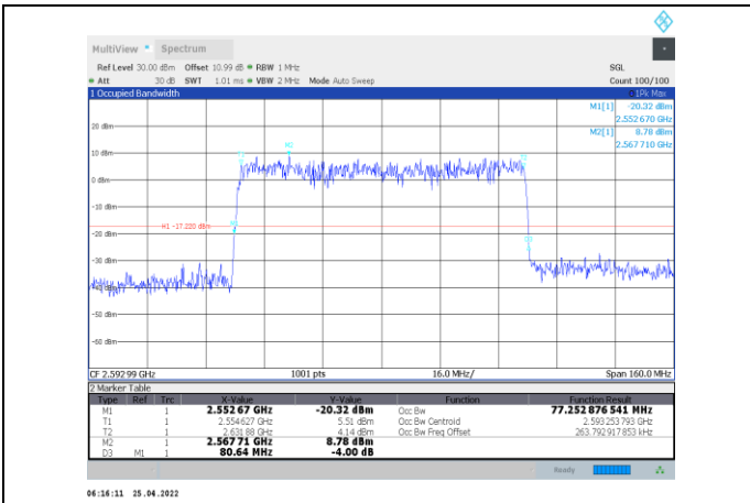
1-N41-PC2-30-80-M-4-CP-256QAM-Outer_Full-217@0-Ant1-77.253-80.640-≤80-PASS
