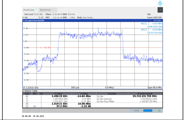
1-N41-PC2-30-40-L-6-DFT-QPSK-Outer_Full-100@0-A nt1-35.742-37.200-≤40-PASS
