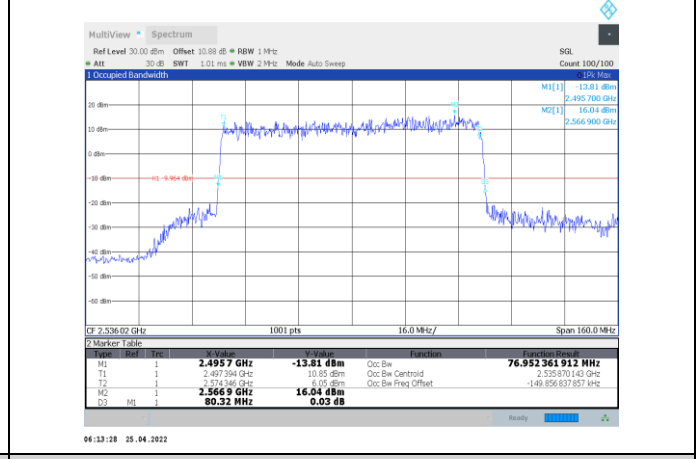
1-N41-PC2-30-80-L-6-DFT-QPSK-Outer_Full-216@0-A nt1-76.952-80.320-≤80-PASS
