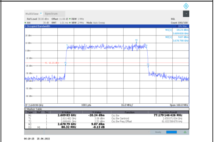
1-N41-PC2-30-80-H-4-CP-256QAM-Outer_Full-217@0-Ant1-77.179-80.320-≤80-PASS
