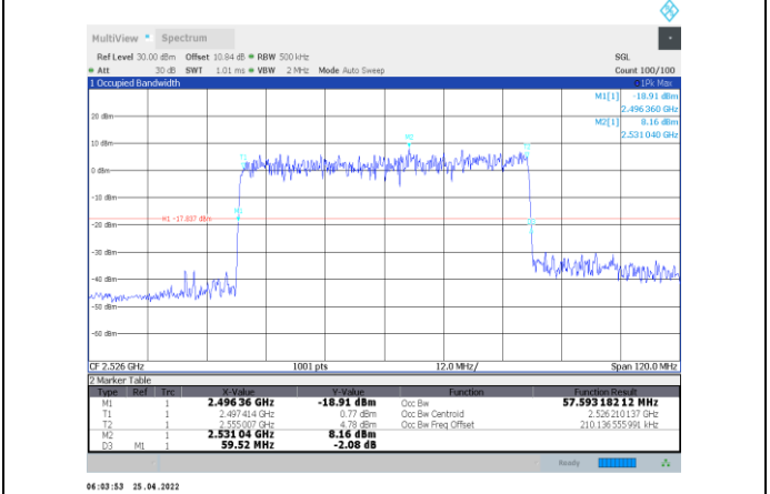
1-N41-PC2-30-60-L-4-CP-256QAM-Outer_Full-162@0- Ant1-57.593-59.520-≤60-PASS
