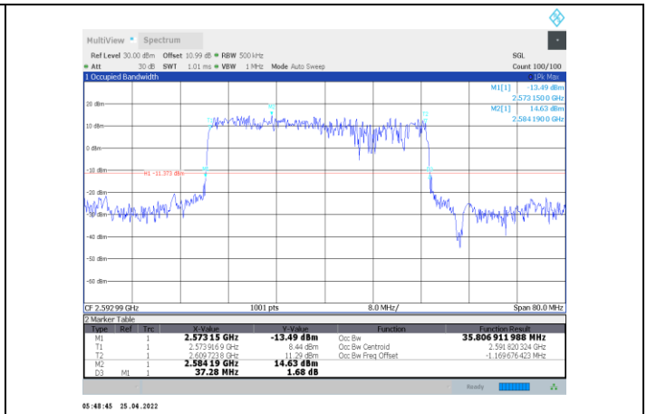
1-N41-PC2-30-40-M-5-DFT-PI/2BPSK-Outer_Full-100@0-Ant1-35.807-37.280-≤40-PASS
