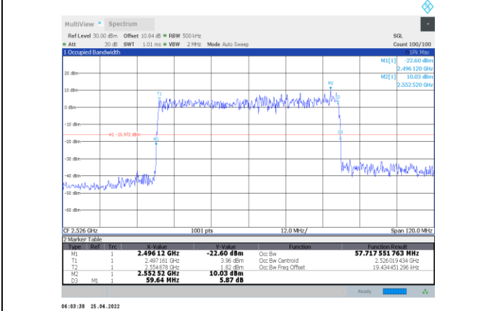
1-N41-PC2-30-60-L-3-CP-64QAM-Outer_Full-162@0-An t1-57.718-59.640-≤60-PASS
