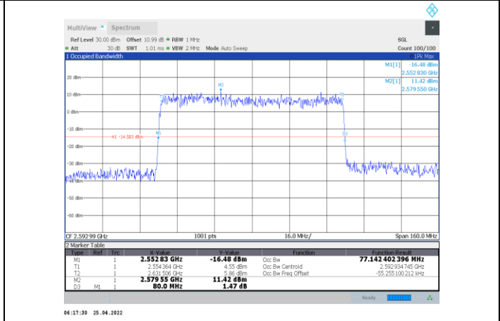
1-N41-PC2-30-80-M-9-DFT-256QAM-Outer_Full-216@0-Ant1-77.142-80.000-≤80-PASS
