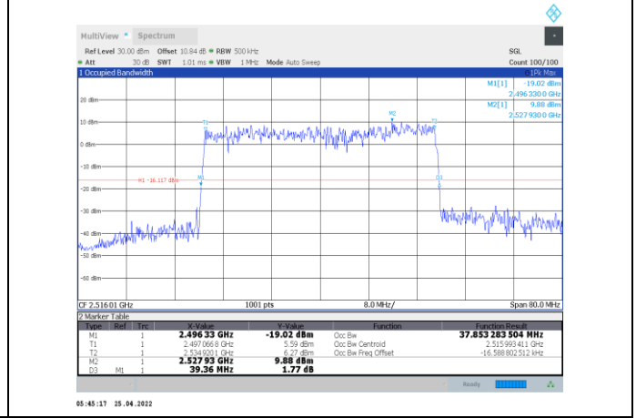
1-N41-PC2-30-40-L-4-CP-256QAM-Outer_Full-106@0- Ant1-37.853-39.360-≤40-PASS
