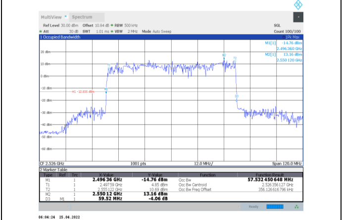
1-N41-PC2-30-60-L-6-DFT-QPSK-Outer_Full-162@0-A nt1-57.532-59.520-≤60-PASS
