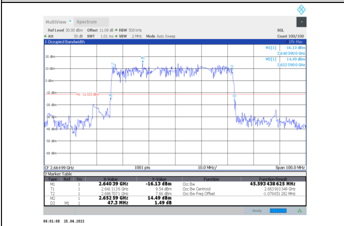
1-N41-PC2-30-50-H-5-DFT-PI/2BPSK-Outer_Full-128@0-Ant 1-45.593-47.300-≤50-PASS
