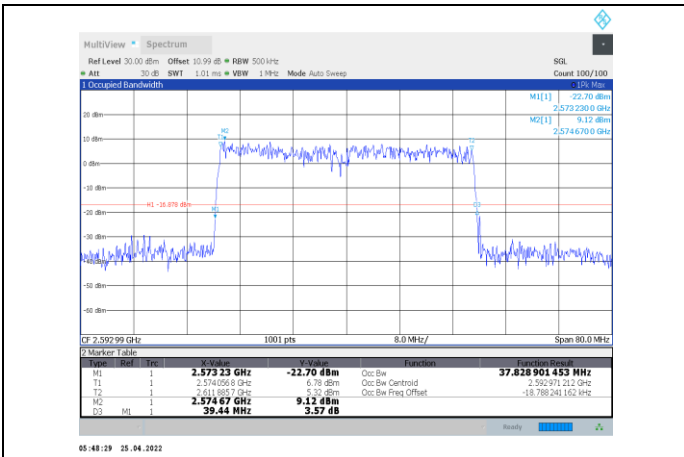
1-N41-PC2-30-40-M-4-CP-256QAM-Outer_Full-106@0-Ant1-37.829-39.440-≤40-PASS
