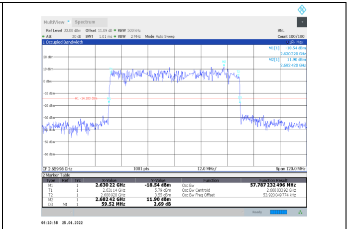
1-N41-PC2-30-60-H-8-DFT-64QAM-Outer_Full-162@0-Ant1-57.787-59.520-≤60-PASS
