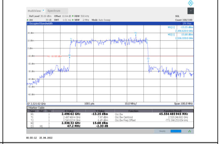
1-N41-PC2-30-50-L-6-DFT-QPSK-Outer_Full-128@0-A nt1-45.554-47.200-≤50-PASS
