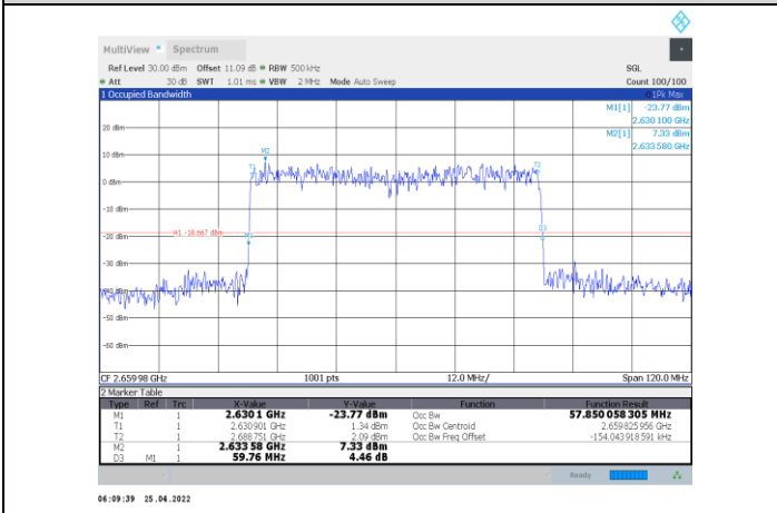
1-N41-PC2-30-60-H-3-CP-64QAM-Outer_Full-162@0-Ant 1-57.85-59.760-≤60-PASS
