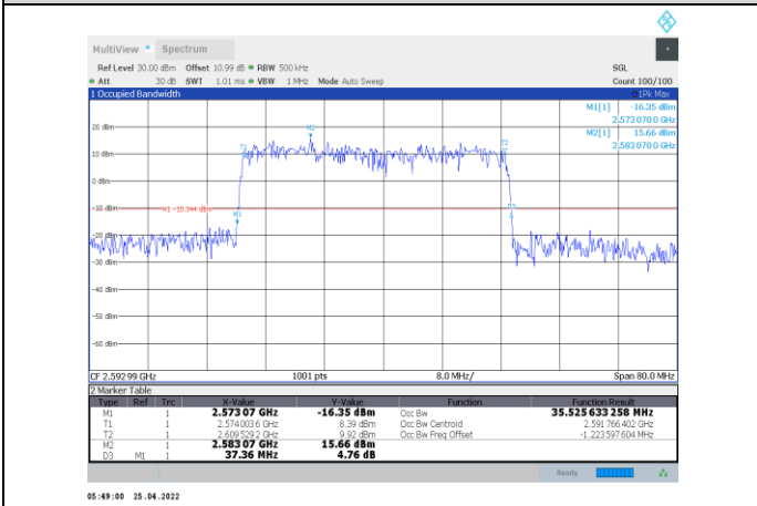
1-N41-PC2-30-40-M-6-DFT-QPSK-Outer_Full-100@0-Ant1-35.526-37.360-≤40-PASS
