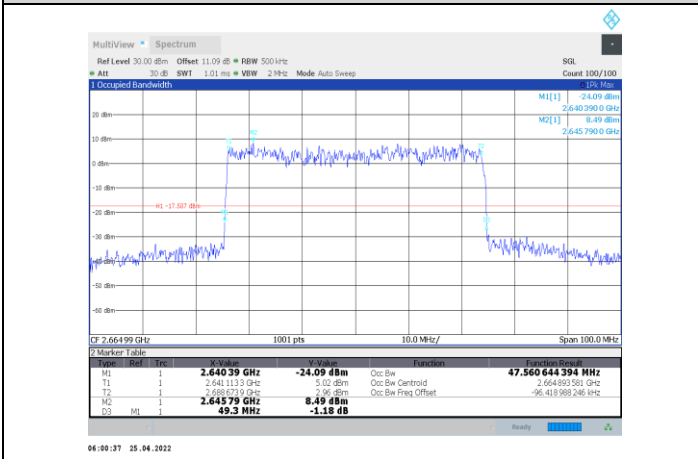
1-N41-PC2-30-50-H-3-CP-64QAM-Outer_Full-133@0-Ant 1-47.561-49.300-≤50-PASS
