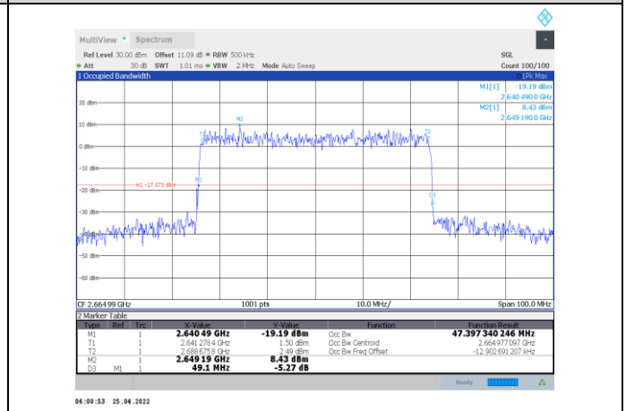
1-N41-PC2-30-50-H-4-CP-256QAM-Outer_Full-133@0-Ant 1-47.397-49.100-≤50-PASS
