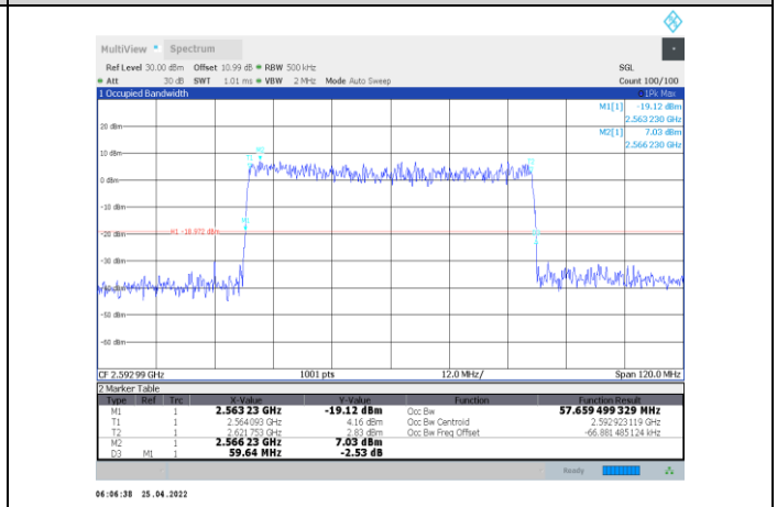
1-N41-PC2-30-60-M-3-CP-64QAM-Outer_Full-162@0-A nt1-57.659-59.640-≤60-PASS
