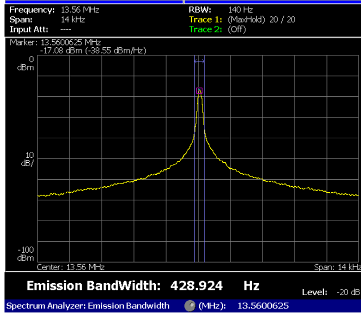
Figure B-9: Measurement results for 20dB Bandwidth
