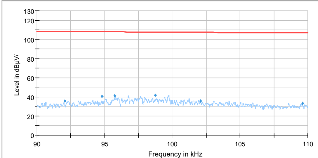
Radiates Emission from 90kHz to 110kHz
