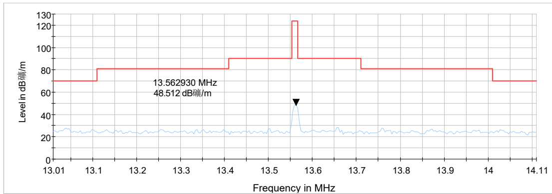
Radiates Emission from 13.01MHz to 14.11MHz
