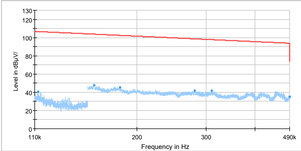
Radiates Emission from 110kHz to 490kHz
