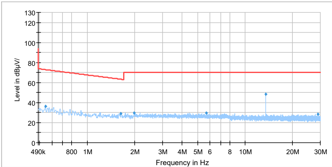
Radiates Emission from 490kHz to 30MHz
