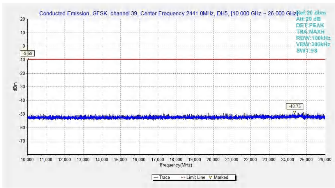
Fig.38. Conducted spurious emission: GFSK, Channel 39, 10GHz – 26GHz
