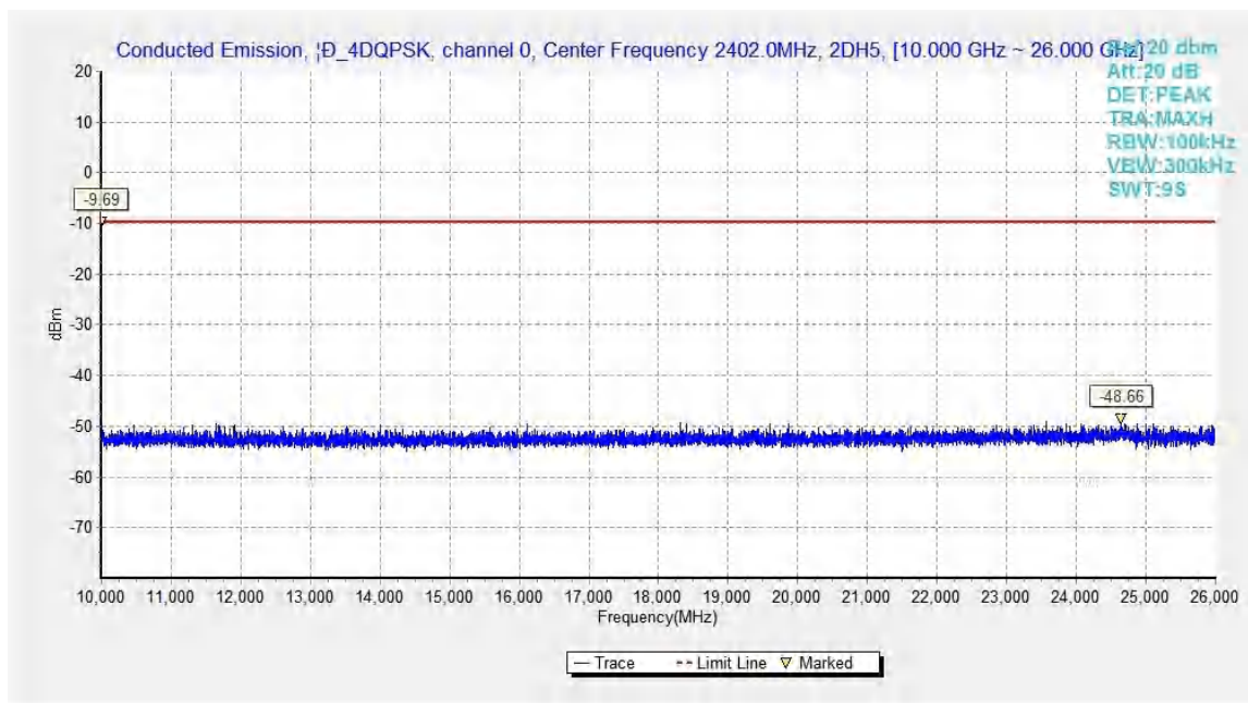
Fig.48. Conducted spurious emission: \pi/4 DQPSK, Channel 0, 10GHz - 26GHz
