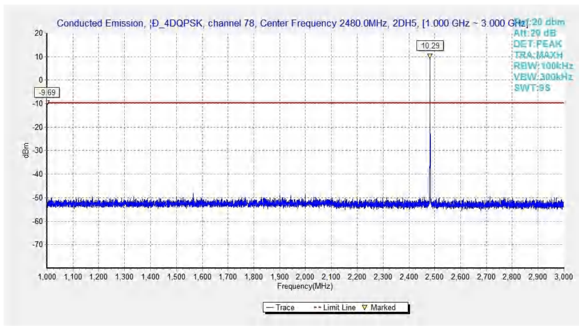
Fig.56. Conducted spurious emission: \pi/4 DQPSK, Channel 78, 1GHz - 3GHz
