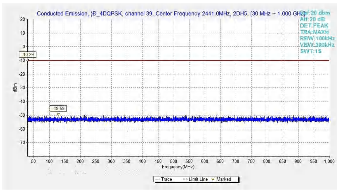
Fig.50. Conducted spurious emission: \pi/4 DQPSK, Channel 39, 30MHz - 1GHz
