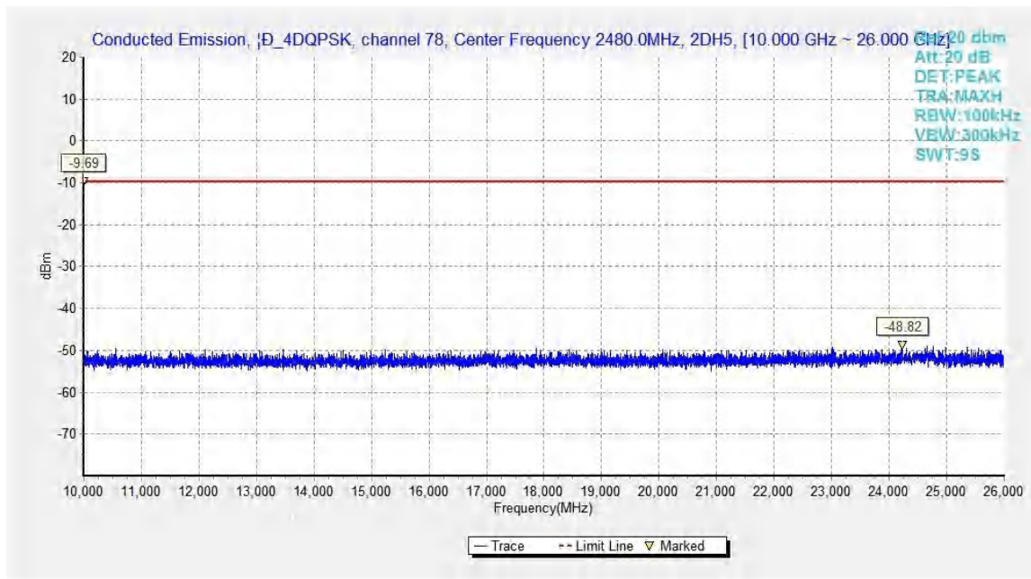
Fig.58. Conducted spurious emission: \pi/4 DQPSK, Channel 78, 10GHz - 26GHz
