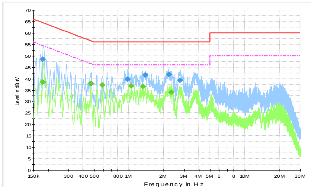
Fig.B.11.1 AC Powerline Conducted Emission-blutetooth(Set.1, (UT18a + AE13 + AE2 + AE17 + AE19)
