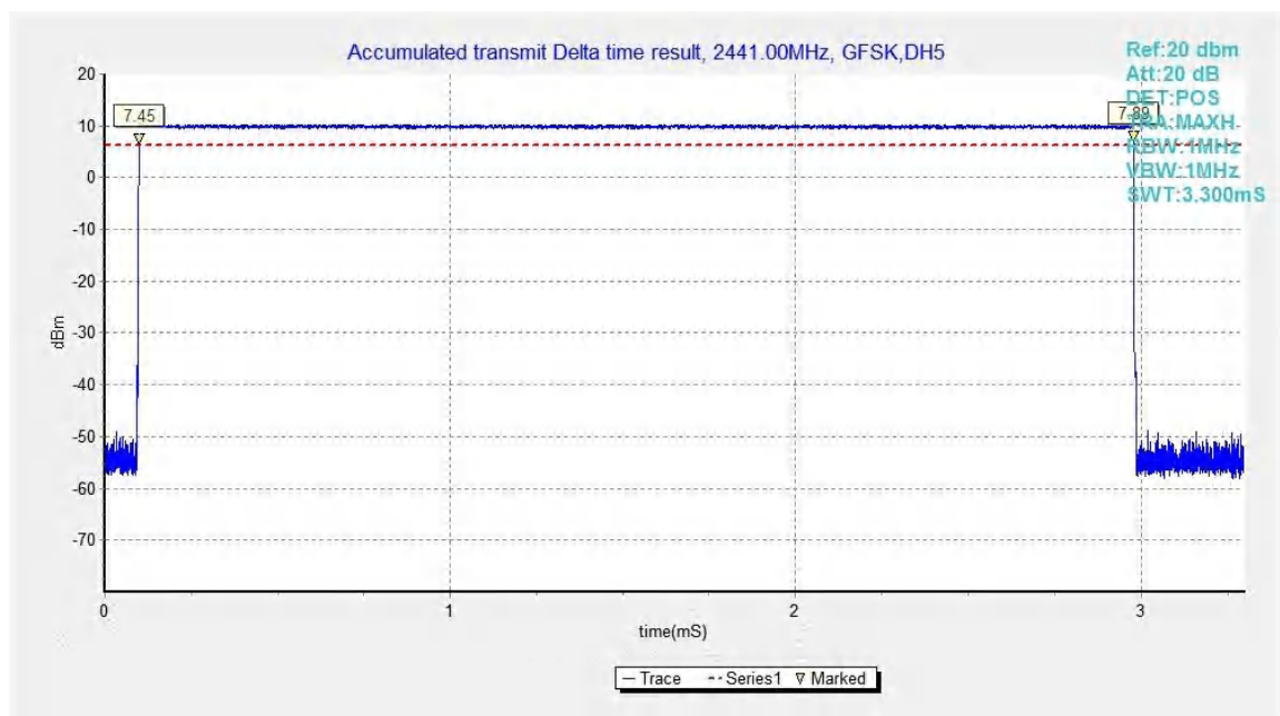
Fig.78. Time of occupancy (Dwell Time): Channel 39, Packet DH5
