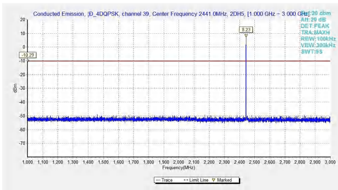
Fig.51. Conducted spurious emission: \pi/4 DQPSK, Channel 39, 1GHz - 3GHz
