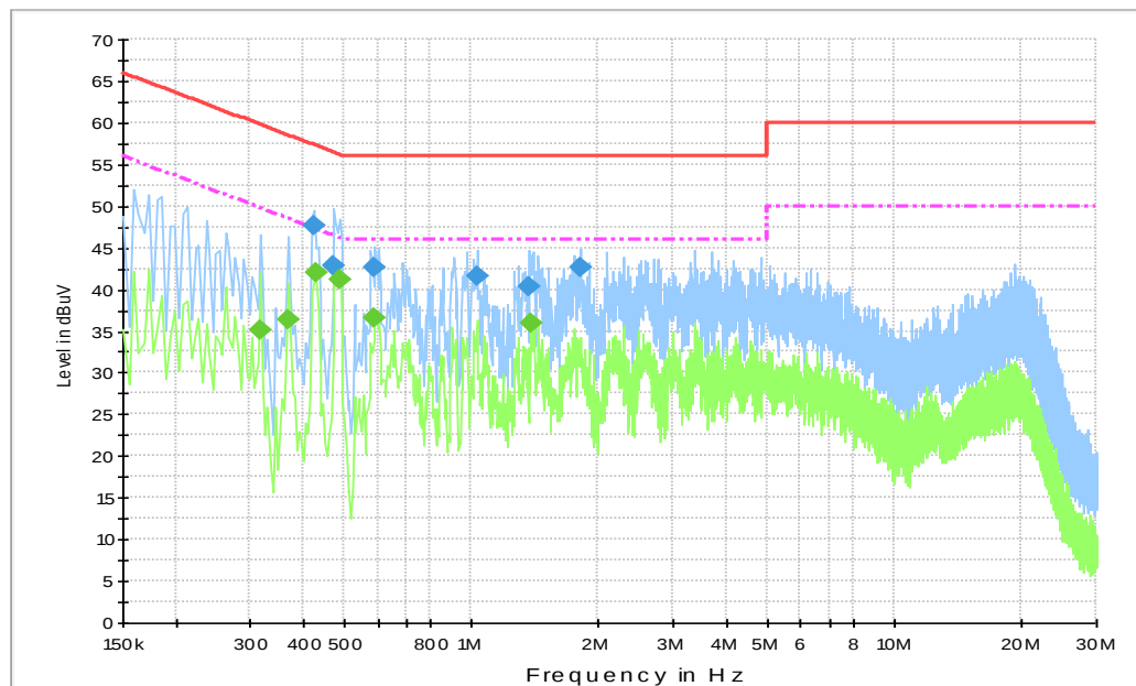
Fig.B.11.3 AC Powerline Conducted Emission-blue tooth(Set.2, UT25a + AE14 + AE4 + AE18 +AE19)
