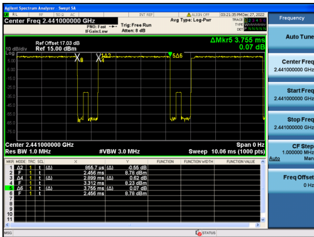
Bluetooth-8-DPSK
