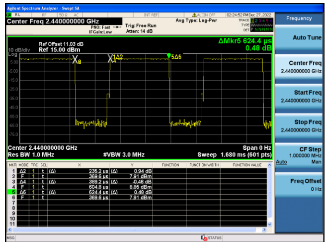
Bluetooth-BLE-1Mbps
