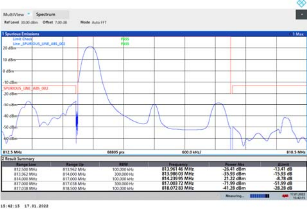
LTE Band 26 QPSK 3MHz CH-Low 1RB
