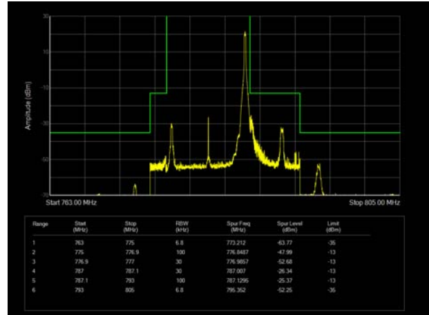
LTE Band 13 QPSK 10MHz CH-High, 100%RB
