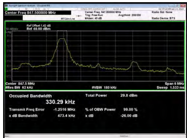
LTE Band 26 QPSK 3MHz CH-High
