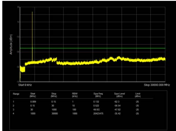
LTE Band 7 10MHz CH- Middle 9kHz~30GHz
