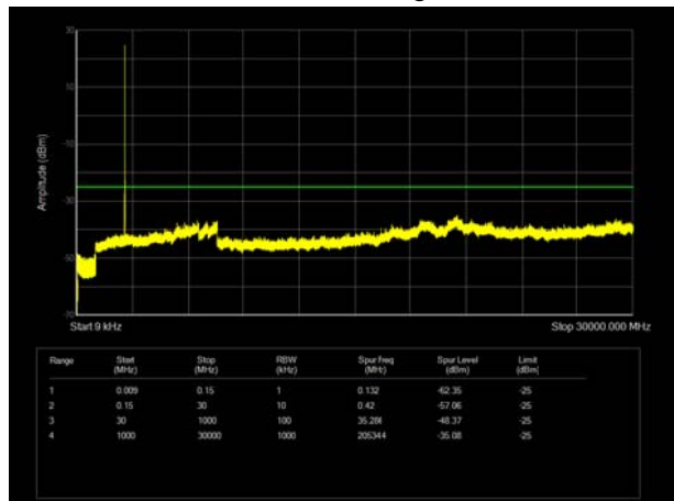
LTE Band 7 10MHz CH- High 9kHz~30GHz
