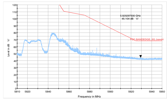
802.11a-Channel 165: Peak
