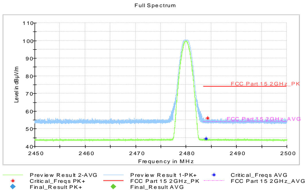
Fig.10. Frequency Band Edges: GFSK, 2480 MHz, Hopping Off, 2.45 GHz - 2.50GHz
