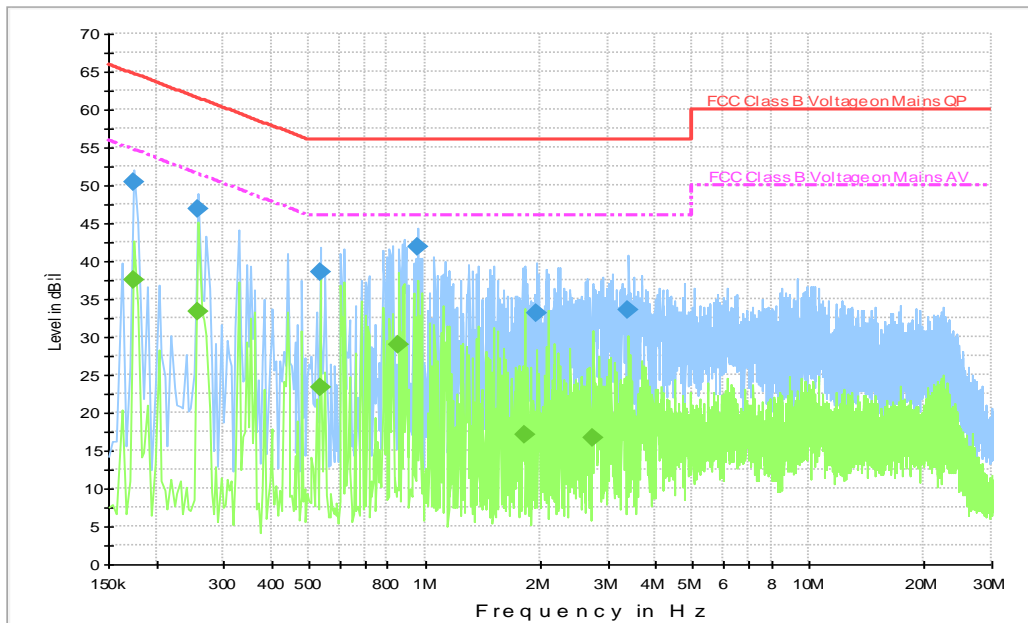
Fig.B.9.3 AC Powerline Conducted Emission-Idle(EUT5 + AE2-3 + AE1-3)
