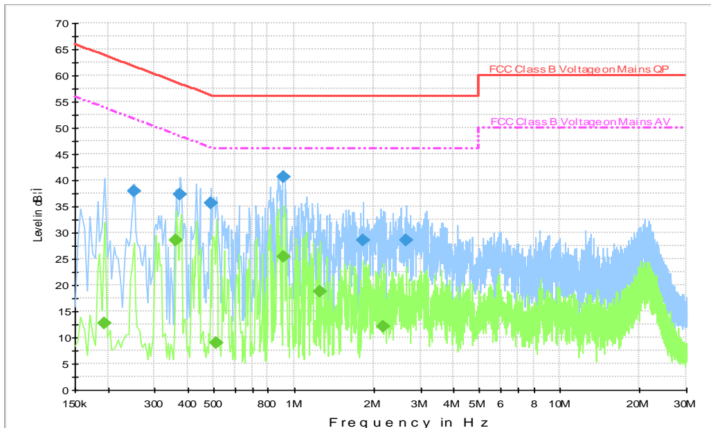
Fig.B.9.1 AC Powerline Conducted Emission-Idle(EUT3 + AE2-1 + AE1-3)
