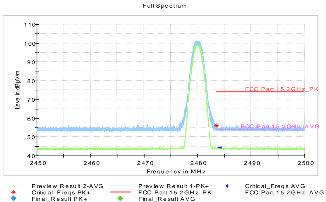
Fig.8. Frequency Band Edges: GFSK, 2480 MHz, Hopping Off , 2.45 GHz - 2.50GHz
