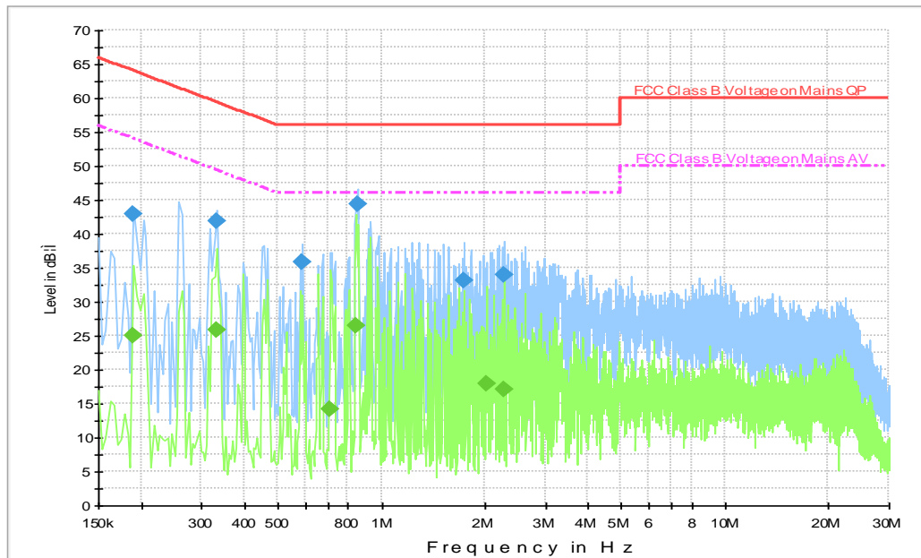
Fig.B.9.5 AC Powerline Conducted Emission-Idle(EUT4 + AE2-5 + AE1-3)
