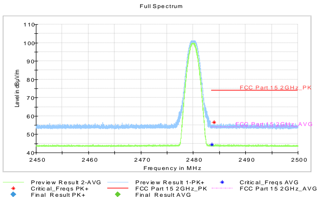
Fig.6. Frequency Band Edges: GFSK, 2480 MHz, Hopping Off, 2.45 GHz - 2.50GHz
