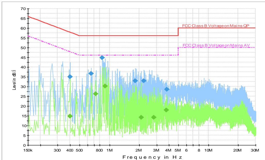
Fig.B.9.2 AC Powerline Conducted Emission-Idle(EUT4 + AE2-2 + AE1-3)
