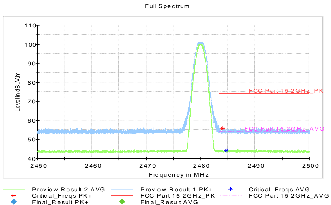
Fig.12. Frequency Band Edges: GFSK, 2480 MHz, Hopping Off, 2.45 GHz - 2.50GHz
