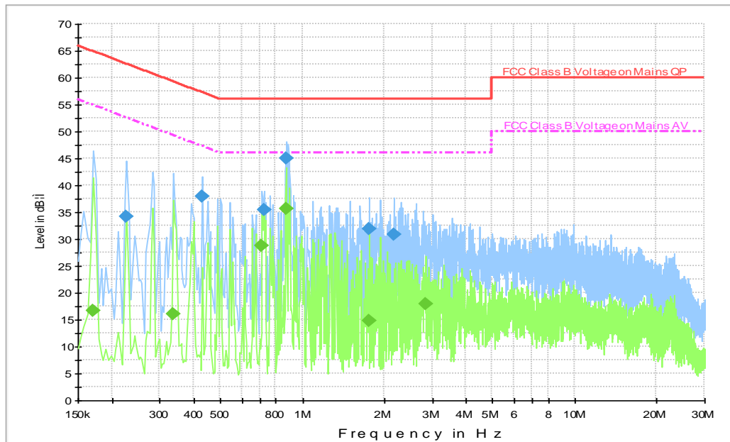
Fig.B.9.4 AC Powerline Conducted Emission-Idle(EUT3 + AE2-4 + AE1-3)
