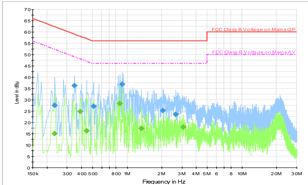
Fig.A.7.5 AC Powerline Conducted Emission-802.11b(UT22a + AE2-4 + AE1-3)
