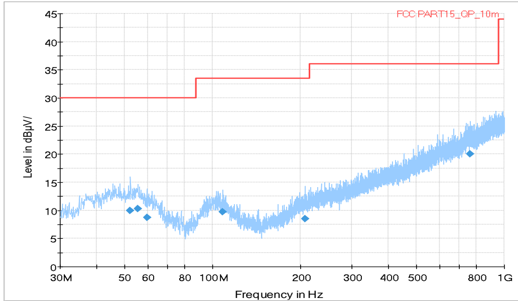
RE FCC_30MHz-1GHz_10m_Direct_testina_FP5b
