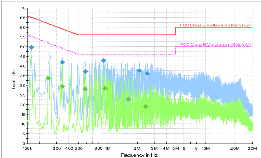
Fig.A.7.4 AC Powerline Conducted Emission-802.11b(UT26a + AE2-3 + AE1-3)
