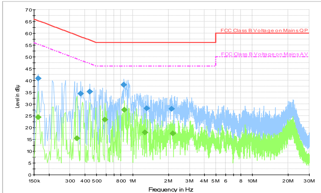
Fig.A.7.1 AC Powerline Conducted Emission-802.11b(UT22a + AE2-1 + AE1-3)
