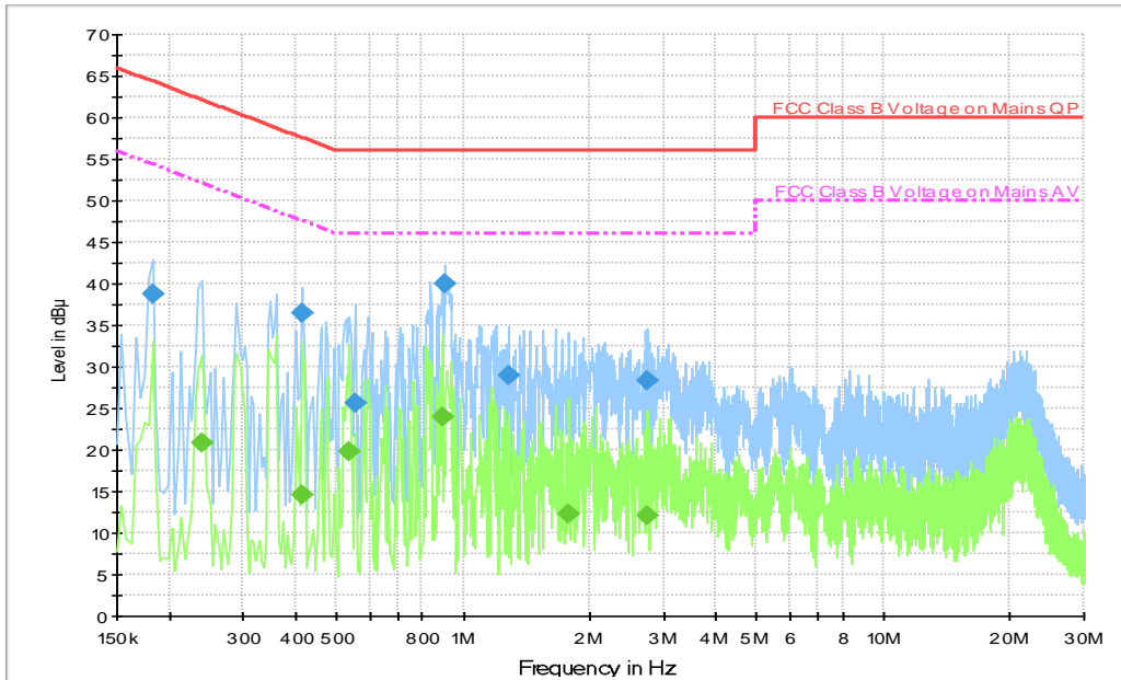
Fig.A.7.3 AC Powerline Conducted Emission-802.11b (UT25a + AE2-2 + AE1-3)
