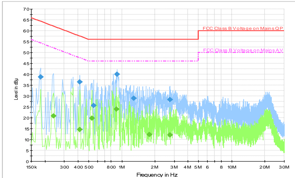
Fig.A.7.2 AC Powerline Conducted Emission-Idle(UT22a + AE2-1 + AE1-3)
