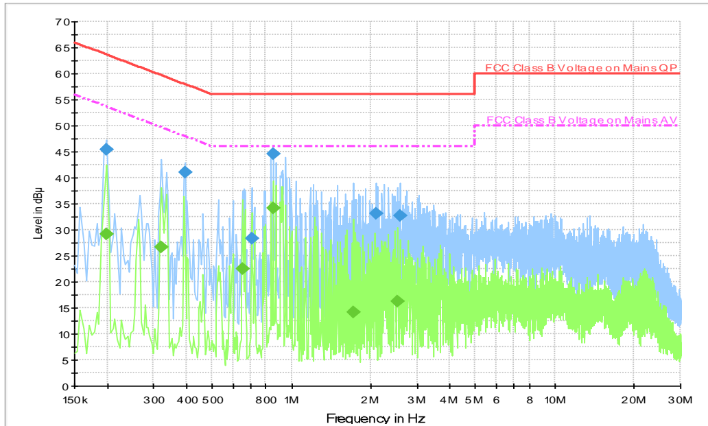
Fig.A.7.6 AC Powerline Conducted Emission-802.11b (UT25a + AE2-5 + AE1-3)
