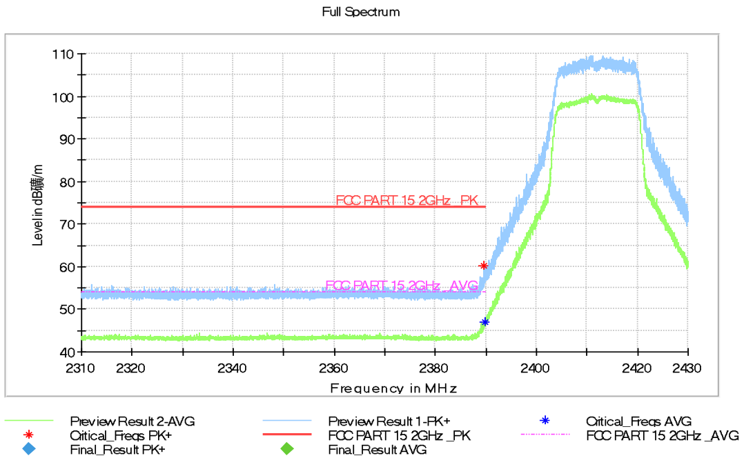
Fig.A.5.11 Band Edges (802.11g, Ch 1, 2.31GHz – 2.43GHz)
