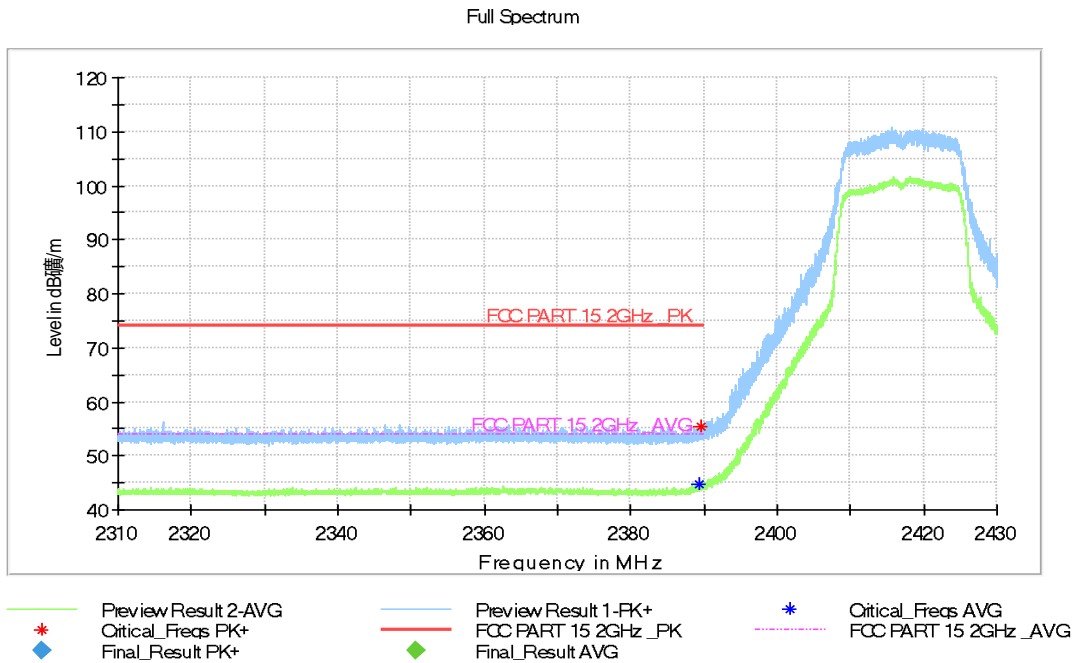
Fig.A.5.12 Band Edges (802.11g, Ch 2, 2.31 GHz – 2.43GHz)
