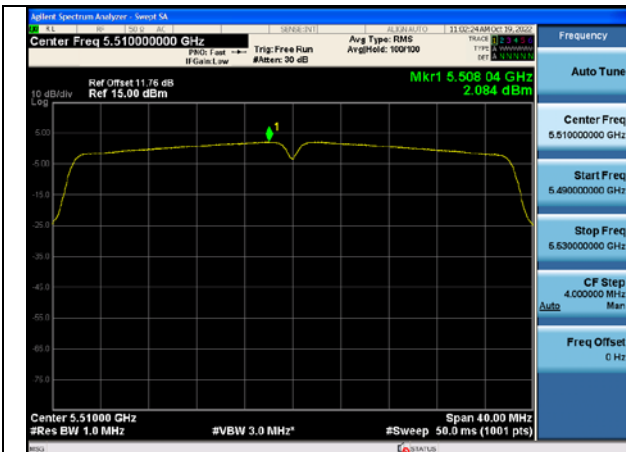
Test Mode:802.11n HT40 5510MHz Chain0
