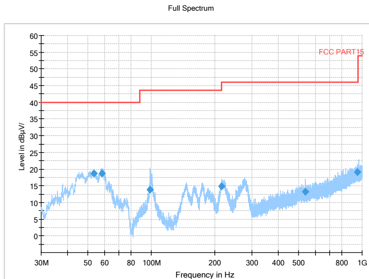
Frequency Range: 30MHz-1000 MHz Detector: QP mode Modulation type: GFSK (LE)
