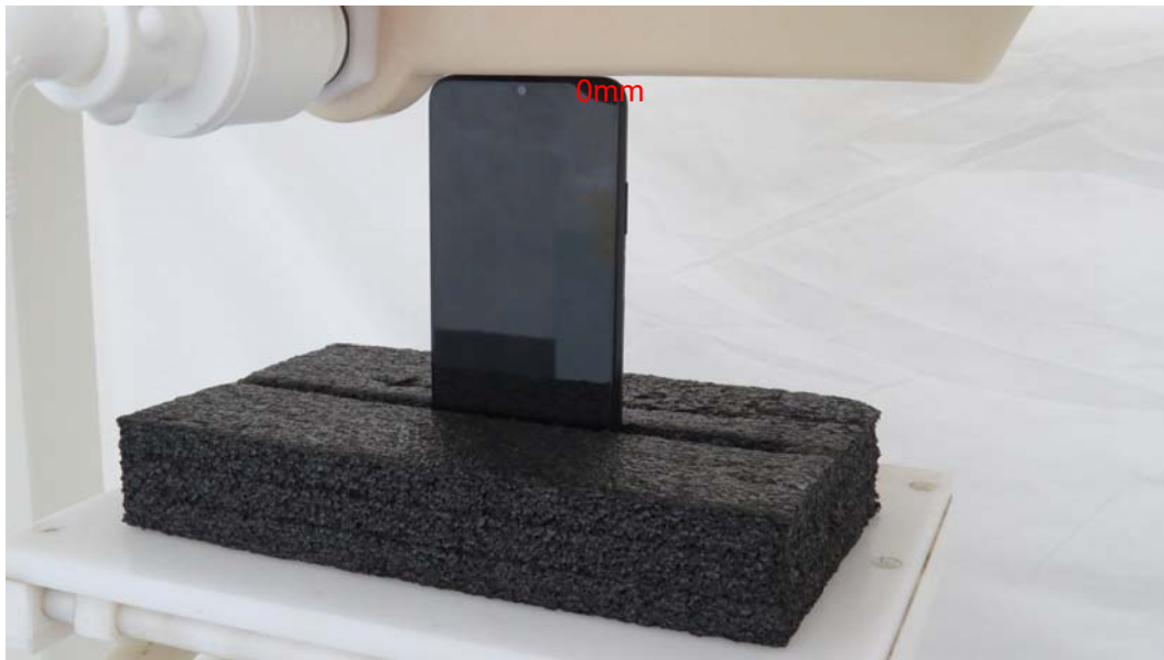
Picture 17: Top Edge, the distance from handset to the bottom of the Phantom is 0mm
