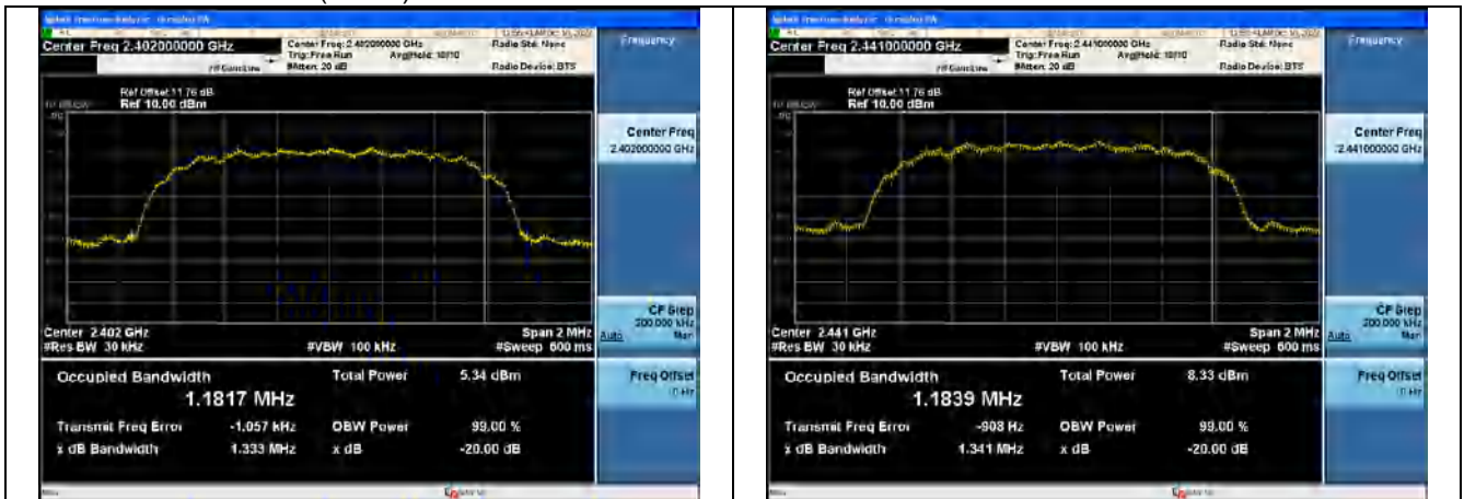
Test Mode: \pi/4 DQPSK(2DH5) 2402MHz
