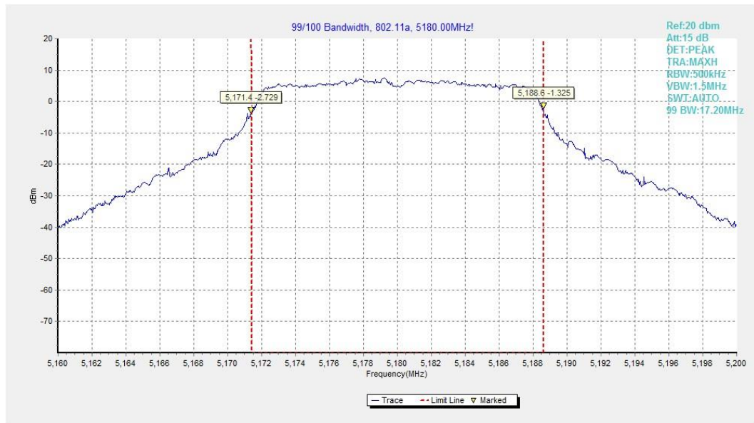
Fig.34 99% Occupied bandwidth (802.11a, 5180MHz)
