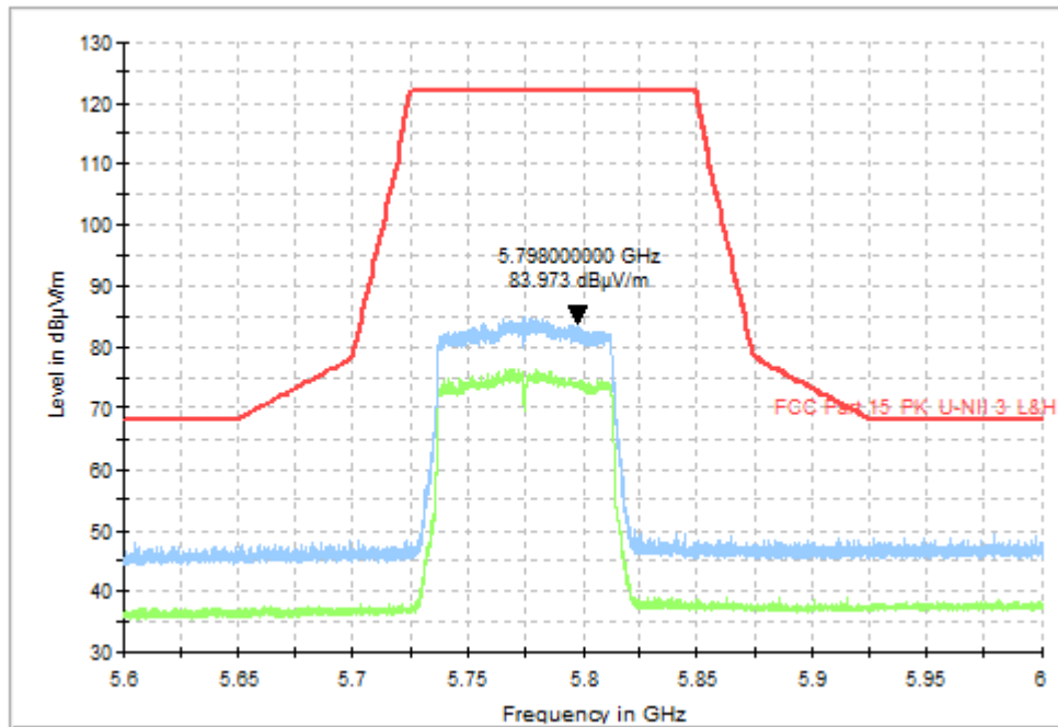
Fig. 17 Band Edges (802.11ac-VHT80, CH155 5775MHz)
