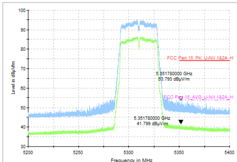
Fig. 8 Band Edges (802.11ac-VHT40, CH62 5310MHz)
