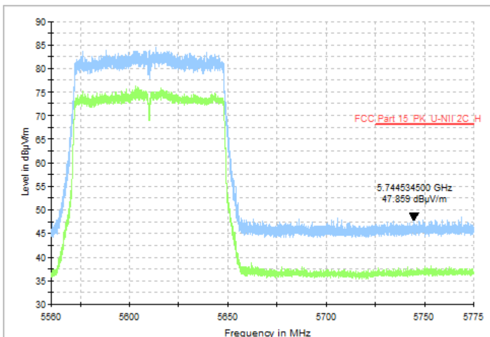
Fig. 16 Band Edges (802.11ac-VHT80, CH122 5610MHz)
