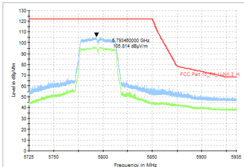
Fig. 12 Band Edges (802.11ac-VHT40, CH159 5795MHz)
