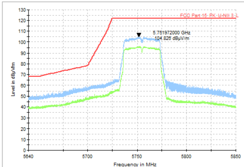
Fig. 11 Band Edges (802.11ac-VHT40, CH151 5755MHz)
