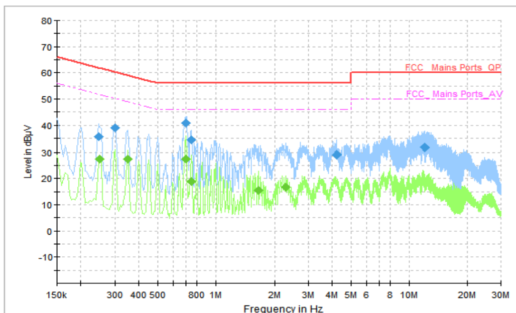
Fig. 49 AC Power line Conducted Emission (Idle)
