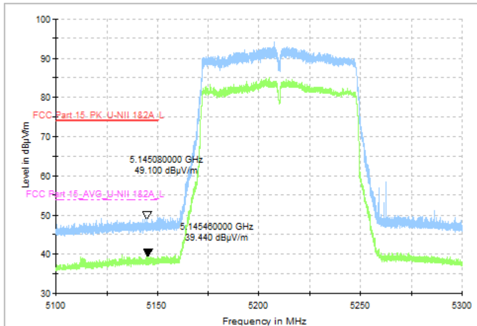
Fig. 13 Band Edges (802.11ac-VHT80, CH42 5210MHz)
