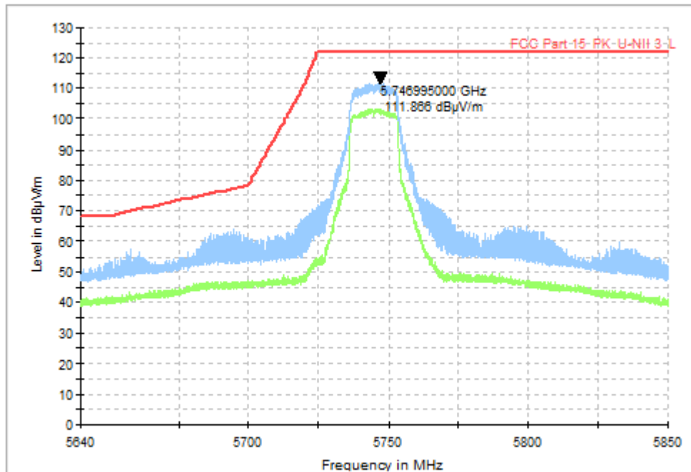
Fig. 5 Band Edges (802.11a, CH149 5745MHz)
