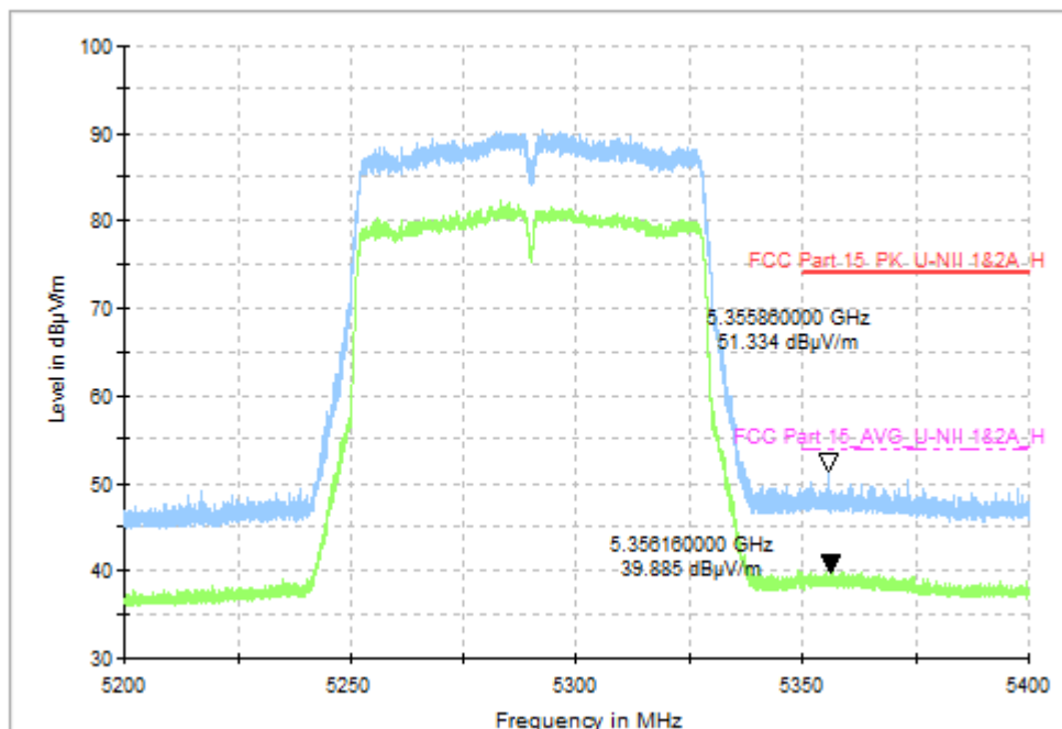
Fig. 14 Band Edges (802.11ac-VHT80, CH58 5290MHz)
