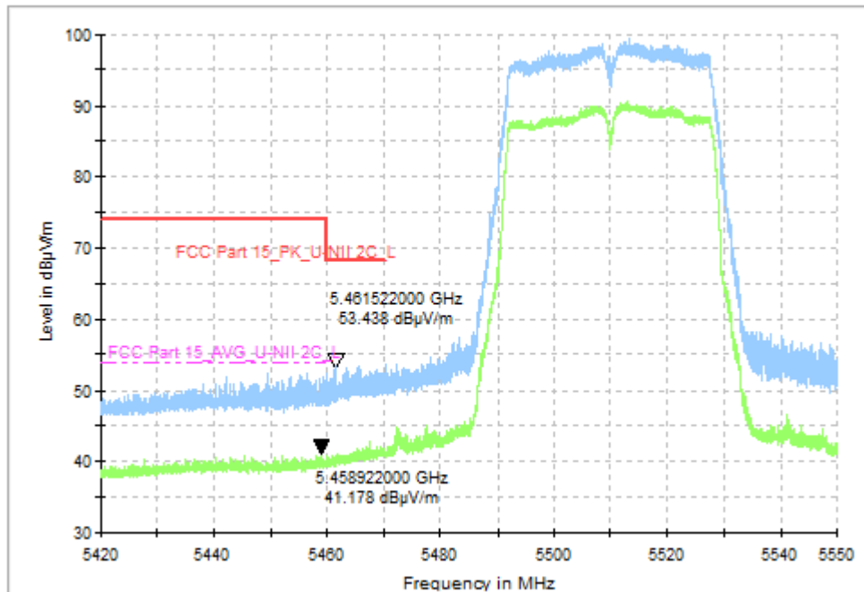
Fig. 9 Band Edges (802.11ac-VHT40, CH102 5510MHz)
