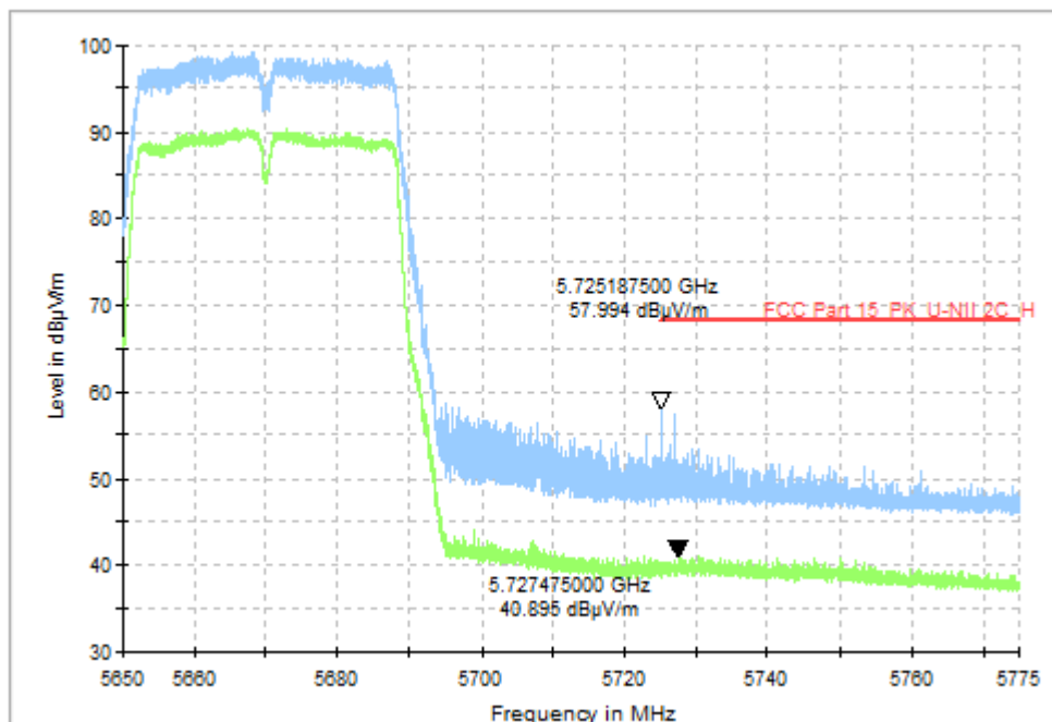
Fig. 10 Band Edges (802.11ac-VHT40, CH134 5670MHz)
