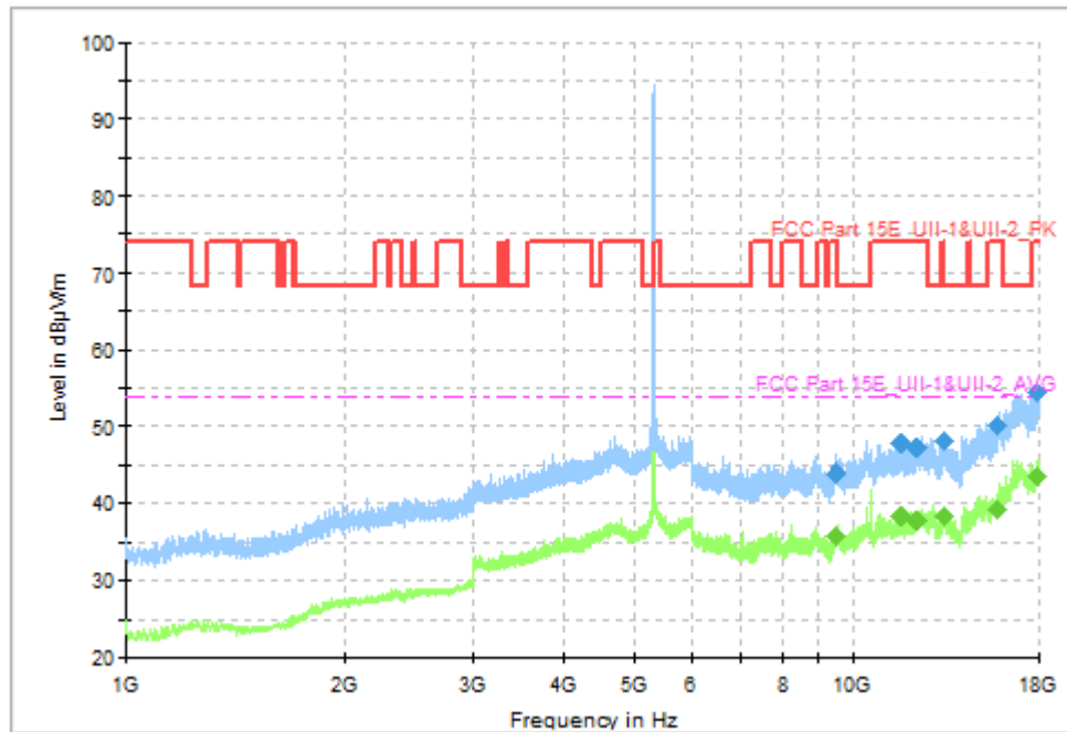
Fig. 33 Transmitter Spurious Emission (802.11ac-VHT40, CH62 5310MHz, 1GHz-18GHz)
