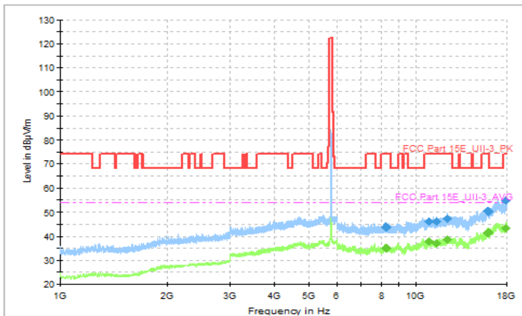
Fig. 43 Transmitter Spurious Emission (802.11ac-VHT80, CH155 5775MHz, 1GHz-18GHz)
