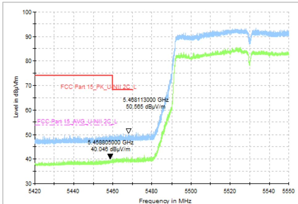
Fig. 15 Band Edges (802.11ac-VHT80, CH106 5530MHz)
