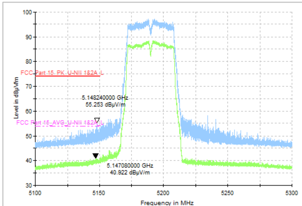
Fig. 7 Band Edges (802.11ac-VHT40, CH38 5190MHz)
