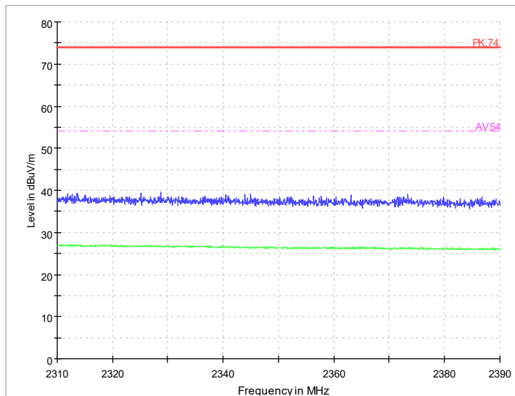
Radiated Emission Band Edge Channel No.:0 Test Mode: GFSK (LE) Polarization: H
