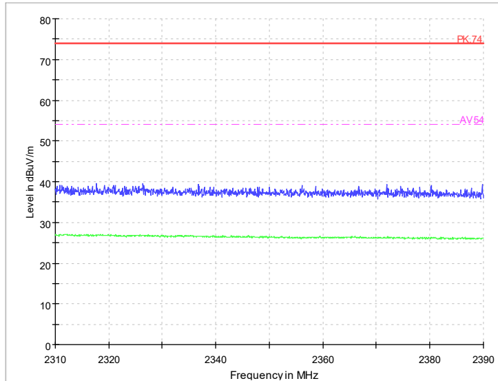
Radiated Emission Band Edge Channel No.:0 Test Mode: GFSK (LE) Polarization: V
