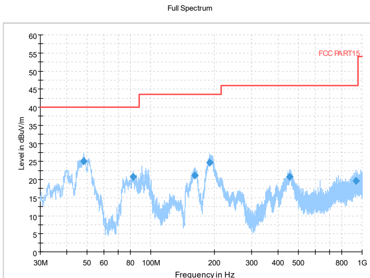
Frequency Range: 30MHz-1000MHz Detector: QP mode
