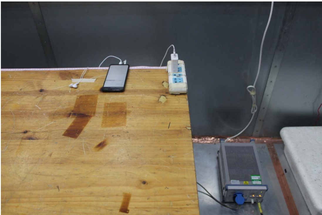
Picture 2 Conducted Emission Test Setup
