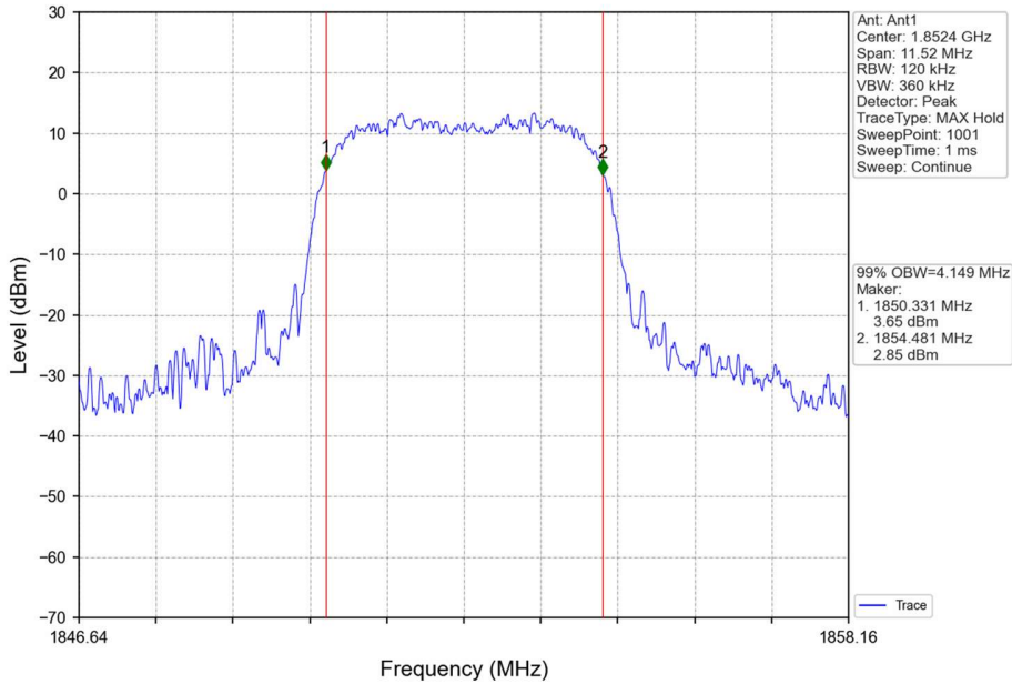
Band2_HSUPA_LCH_1852.4MHz_Subtest 1_NTNV
