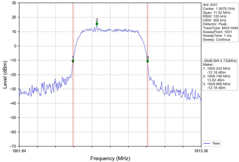
Band2_HSDPA_HCH_1907.6MHz_Subtest 1_NTNV
