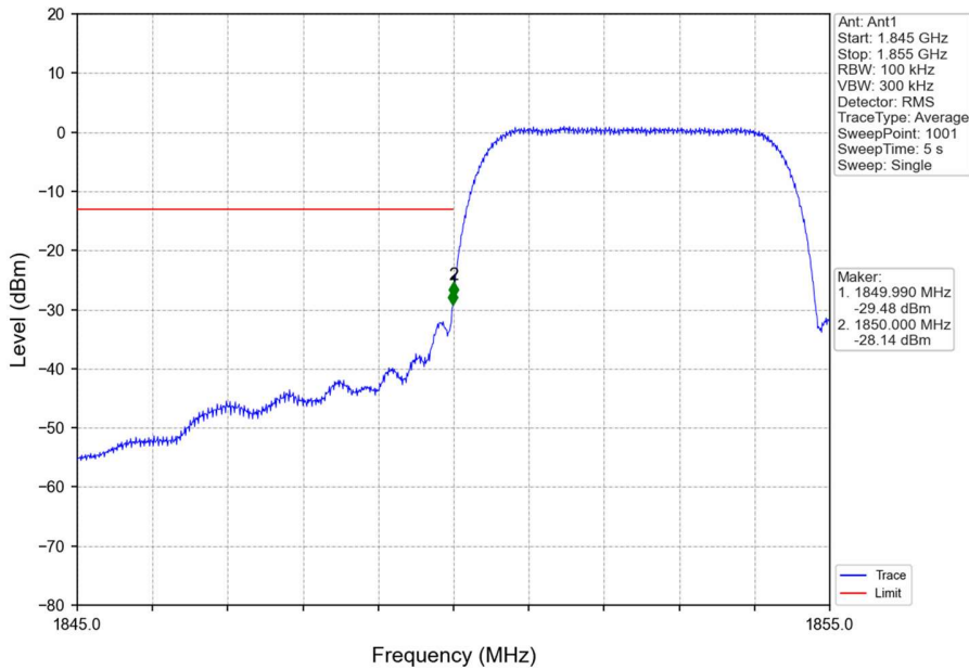
Band2_HSDPA_LCH_1852.4MHz_Subtest 1_NTNV
