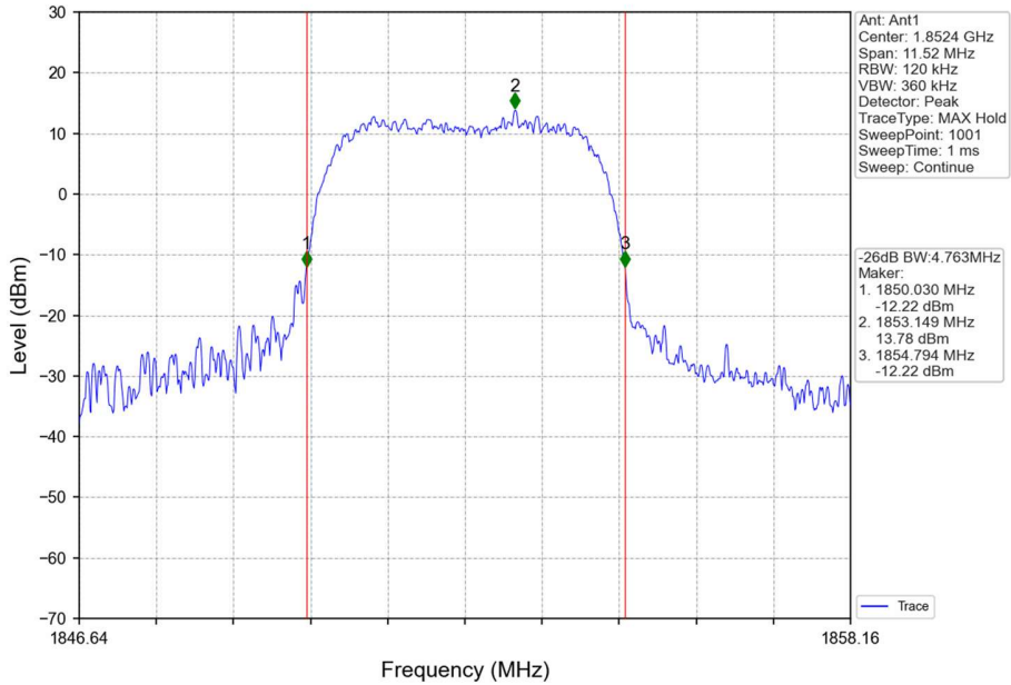
Band2_HSDPA_LCH_1852.4MHz_Subtest 1_NTNV
