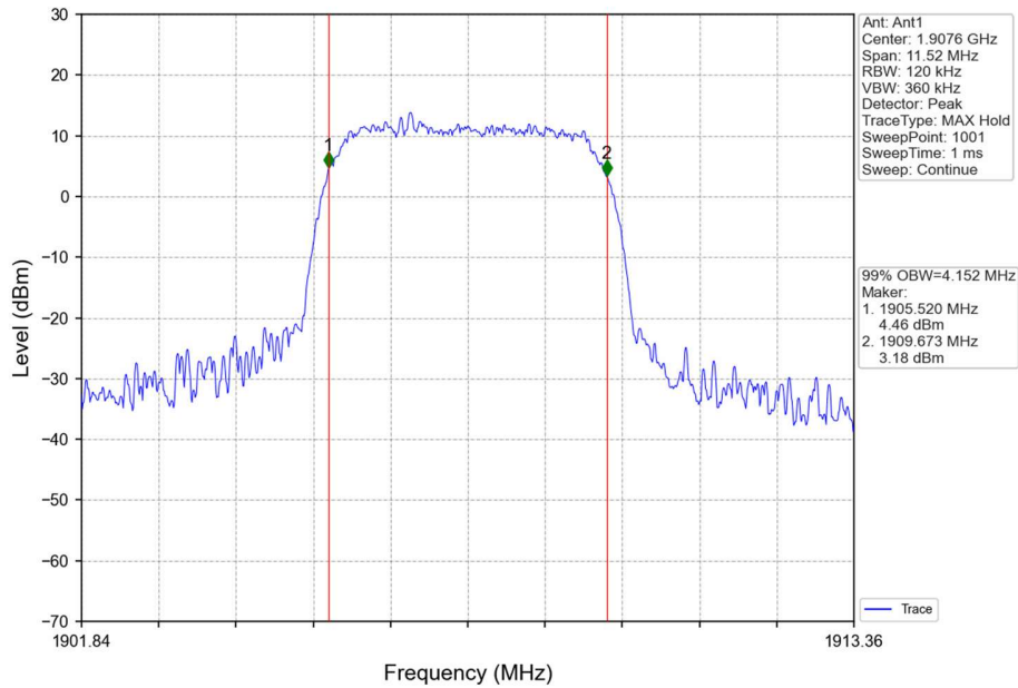
Band2_HSDPA_HCH_1907.6MHz_Subtest 1_NTNV
