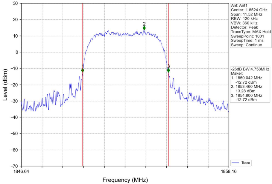
Band2_HSUPA_LCH_1852.4MHz_Subtest 1_NTNV
