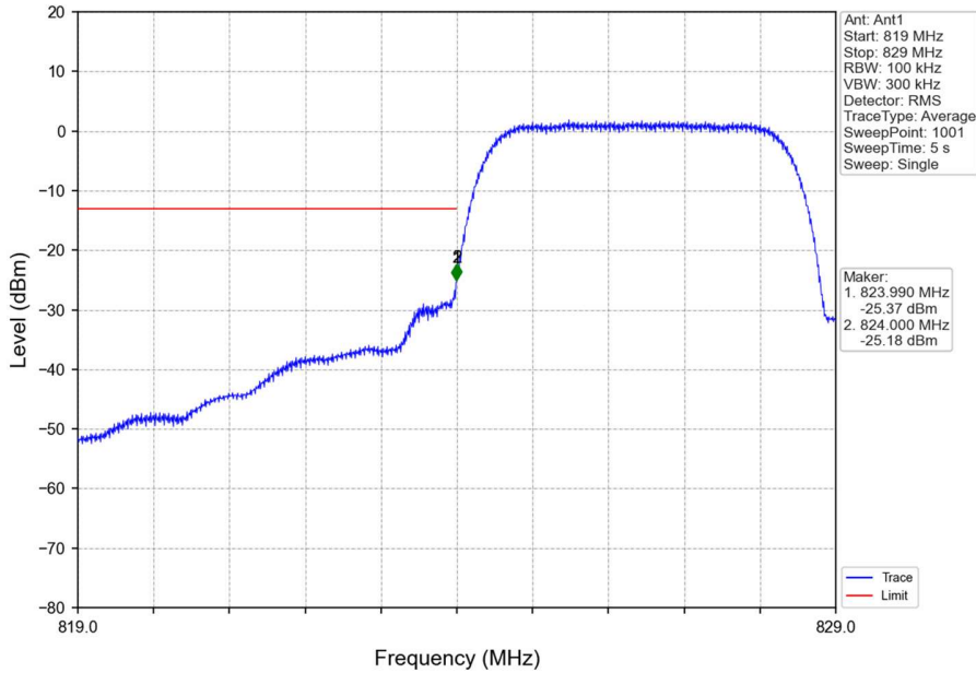
Band5_HSDPA_LCH_826.4MHz_Subtest 1_NTNV
