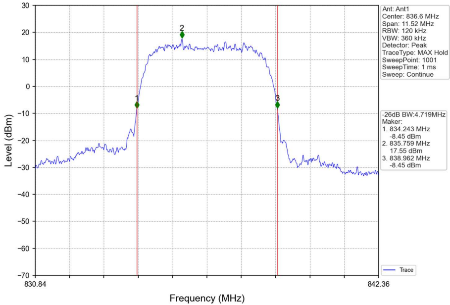
Band5_RMC_MCH_836.6MHz_12.2kbps RMC_NTNV
