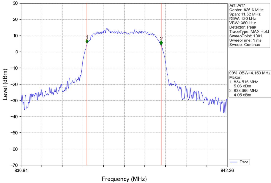
Band5_HSDPA_MCH_836.6MHz_Subtest 1_NTNV
