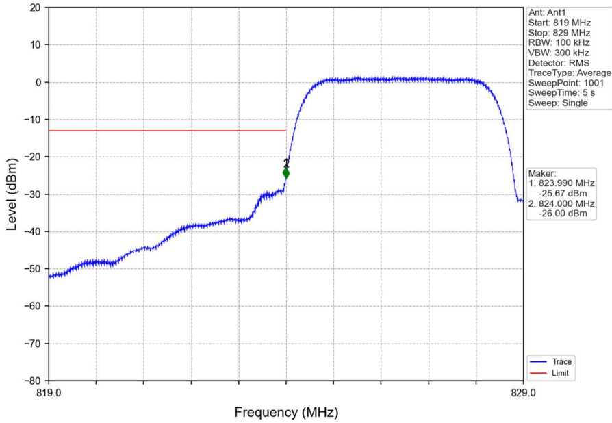
Band5_HSUPA_LCH_826.4MHz_Subtest 1_NTNV
