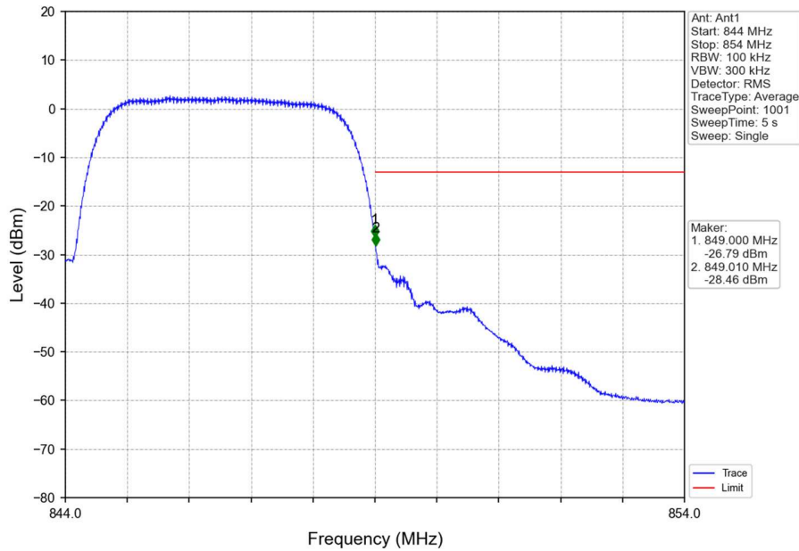
Band5_HSDPA_HCH_846.6MHz_Subtest 1_NTNV
