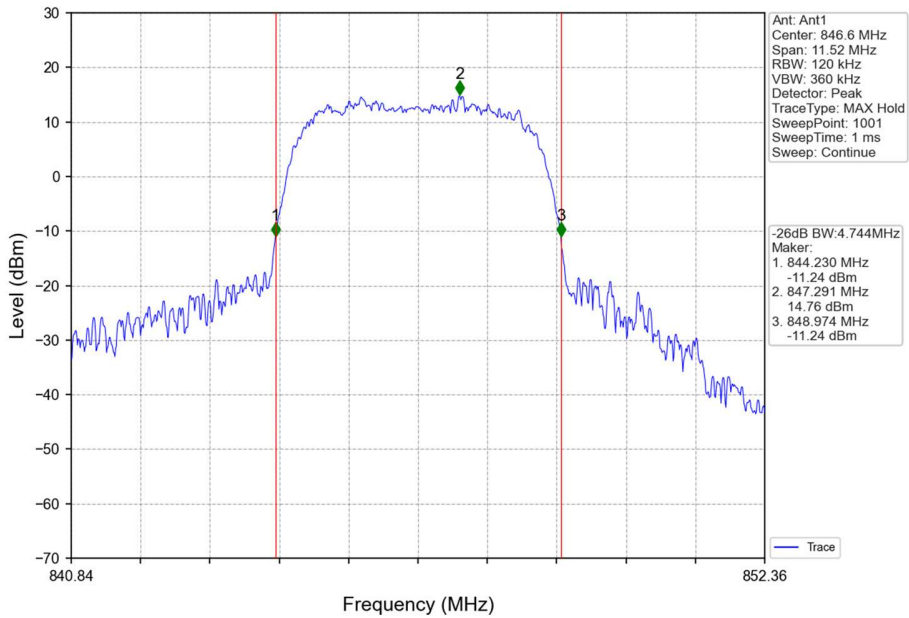
Band5_HSDPA_HCH_846.6MHz_Subtest 1_NTNV
