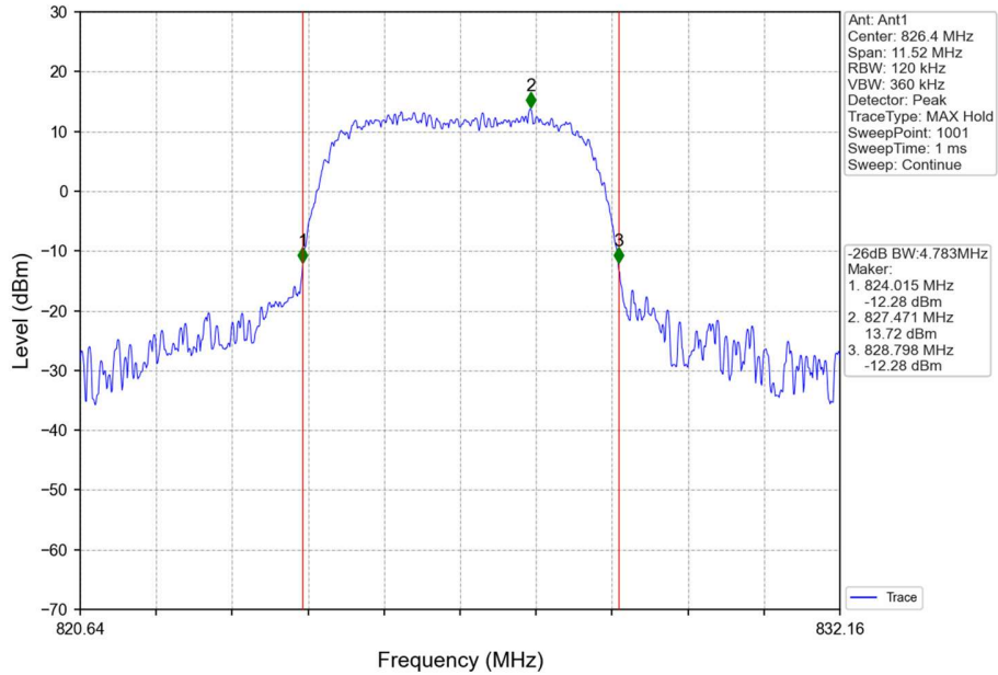
Band5_HSDPA_LCH_826.4MHz_Subtest 1_NTNV
