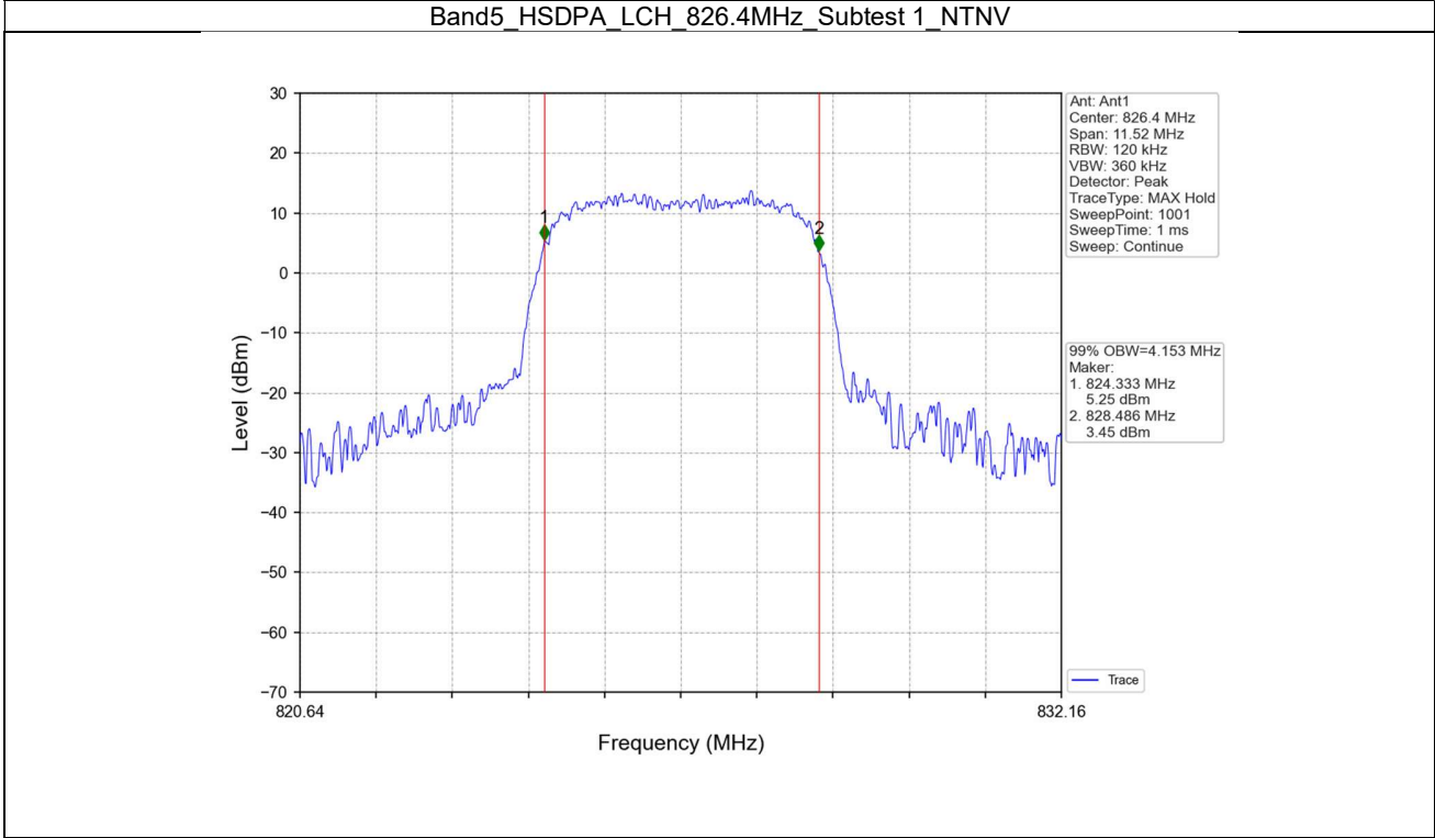
Band5_HSDPA_LCH_826.4MHz_Subtest 1_NTNV
