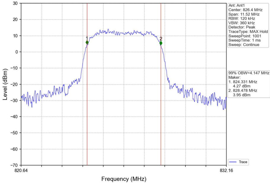
Band5_HSUPA_LCH_826.4MHz_Subtest 1_NTNV
