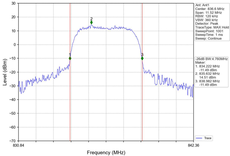
Band5_HSDPA_MCH_836.6MHz_Subtest 1_NTNV
