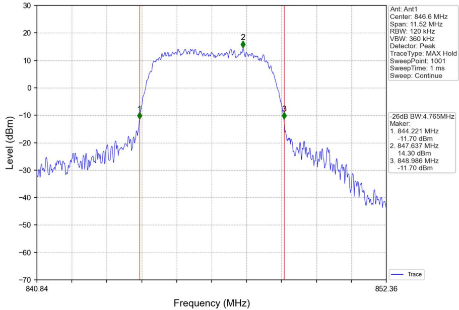
Band5_HSUPA_HCH_846.6MHz_Subtest 1_NTNV
