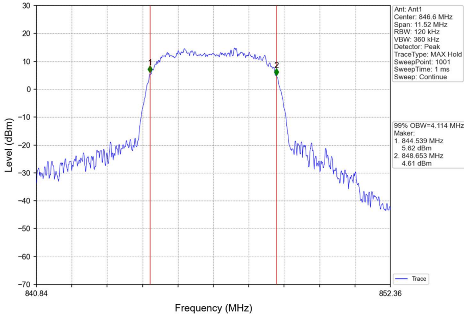
Band5_HSDPA_HCH_846.6MHz_Subtest 1_NTNV
