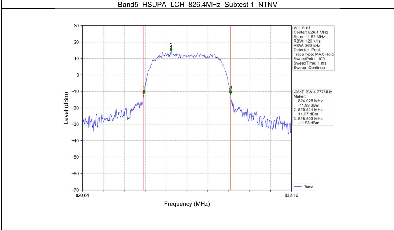
Band5_HSUPA_LCH_826.4MHz_Subtest 1_NTNV
