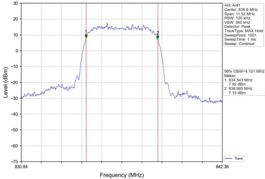
Band5_RMC_MCH_836.6MHz_12.2kbps RMC_NTNV
