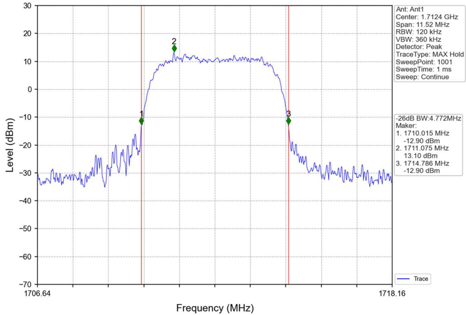
Band4_HSDPA_LCH_1712.4MHz_Subtest 1_NTNV
