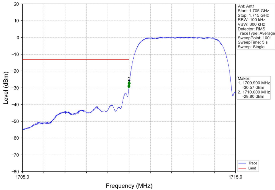
Band4_HSDPA_LCH_1712.4MHz_Subtest 1_NTNV
