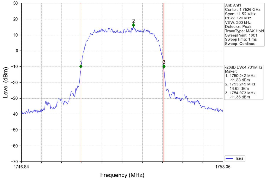
Band4_RMC_HCH_1752.6MHz_12.2kbps_RMC_NTNV
