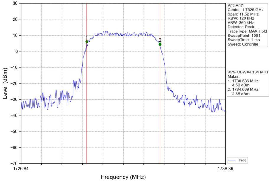
Band4_HSUPA_MCH_1732.6MHz_Subtest 1_NTNV
