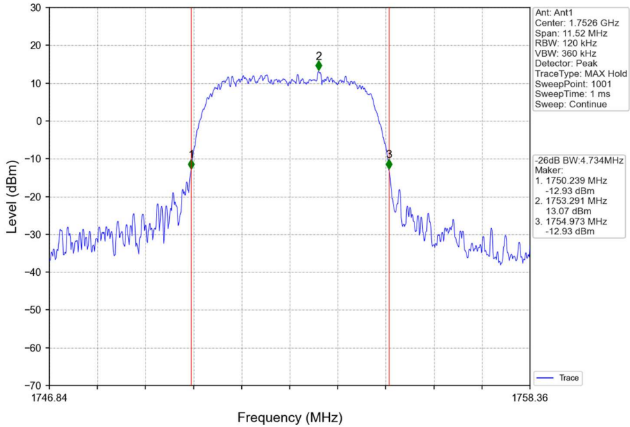
Band4_HSUPA_HCH_1752.6MHz_Substest 1_NTNV
