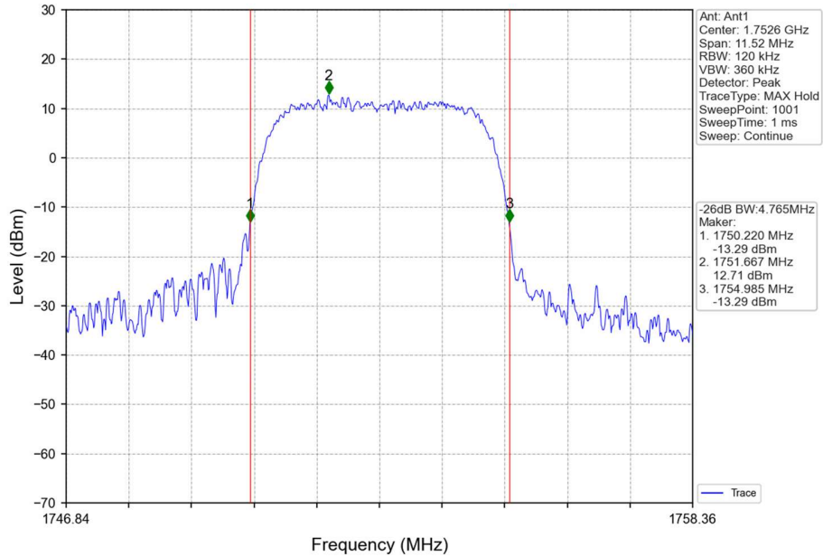
Band4_HSDPA_HCH_1752.6MHz_Subtest 1_NTNV
