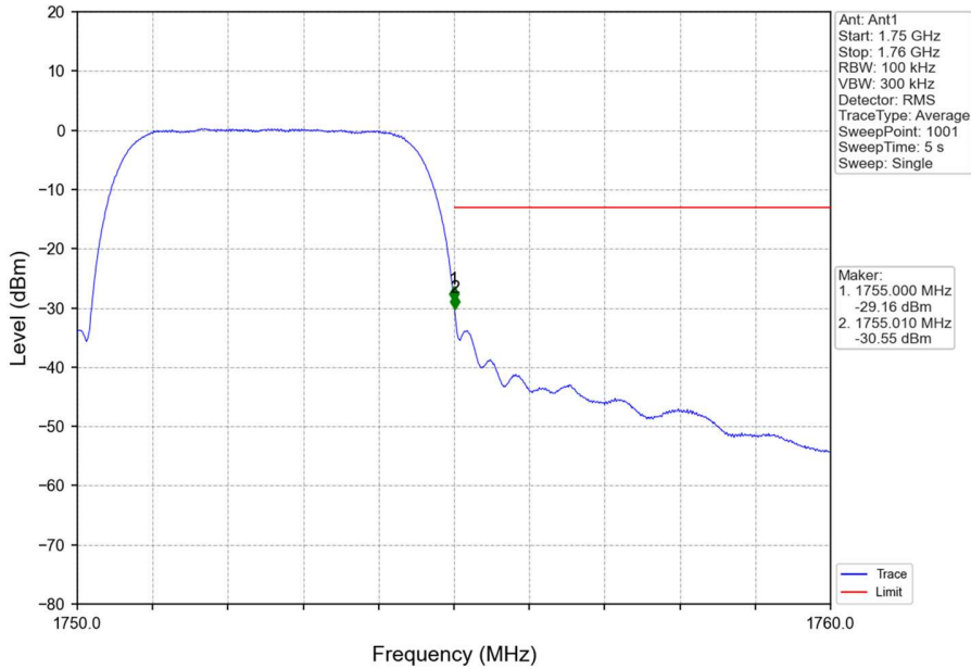
Band4_HSUPA_HCH_1752.6MHz_Subtest 1_NTNV
