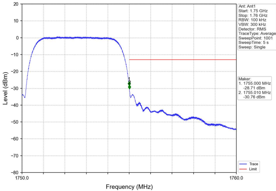
Band4_HSDPA_HCH_1752.6MHz_Subtest 1_NTNV
