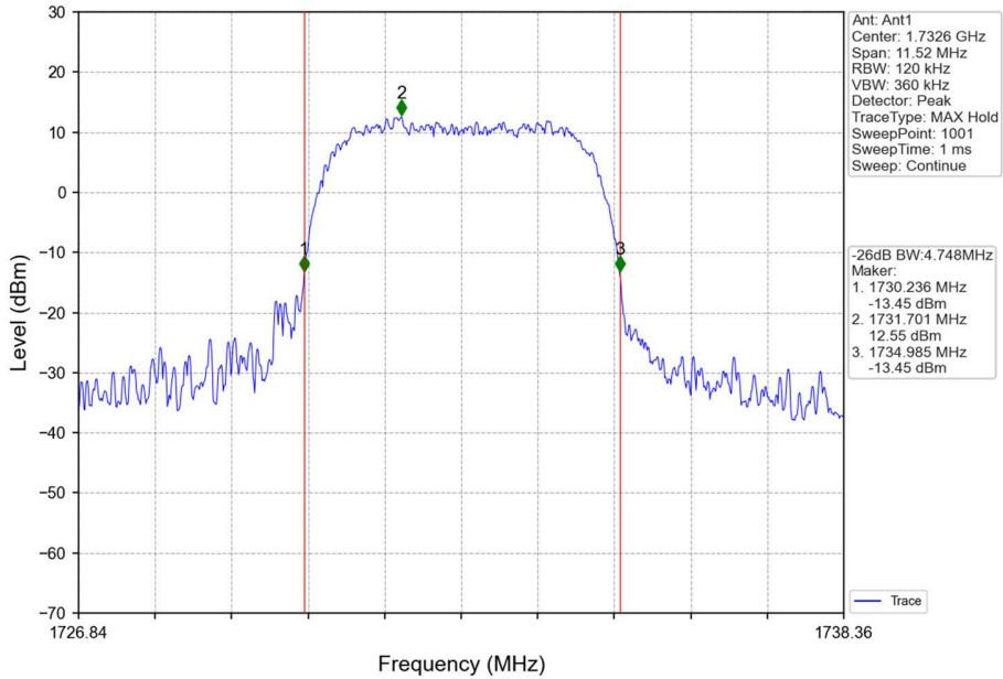
Band4_HSUPA_MCH_1732.6MHz_Subtest 1_NTNV
