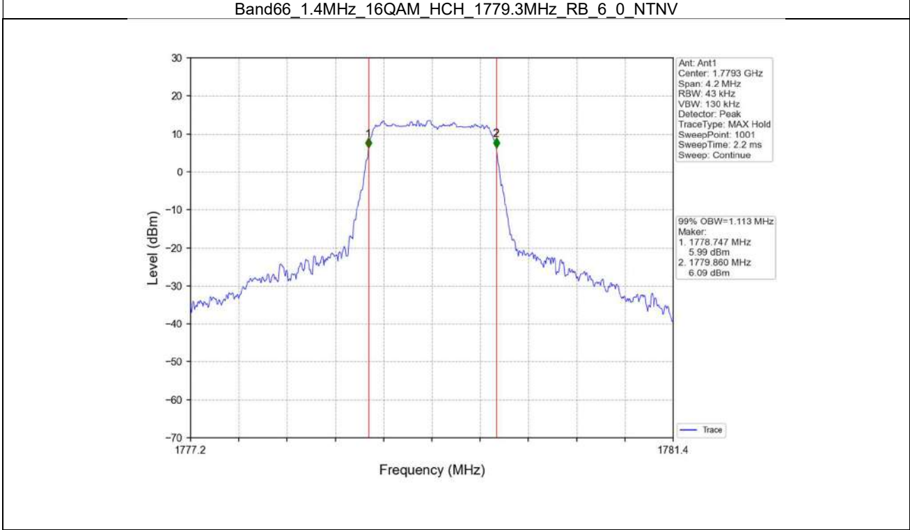
Band66_1.4MHz_16QAM_HCH_1779.3MHz_RB_6_0_NTNV
