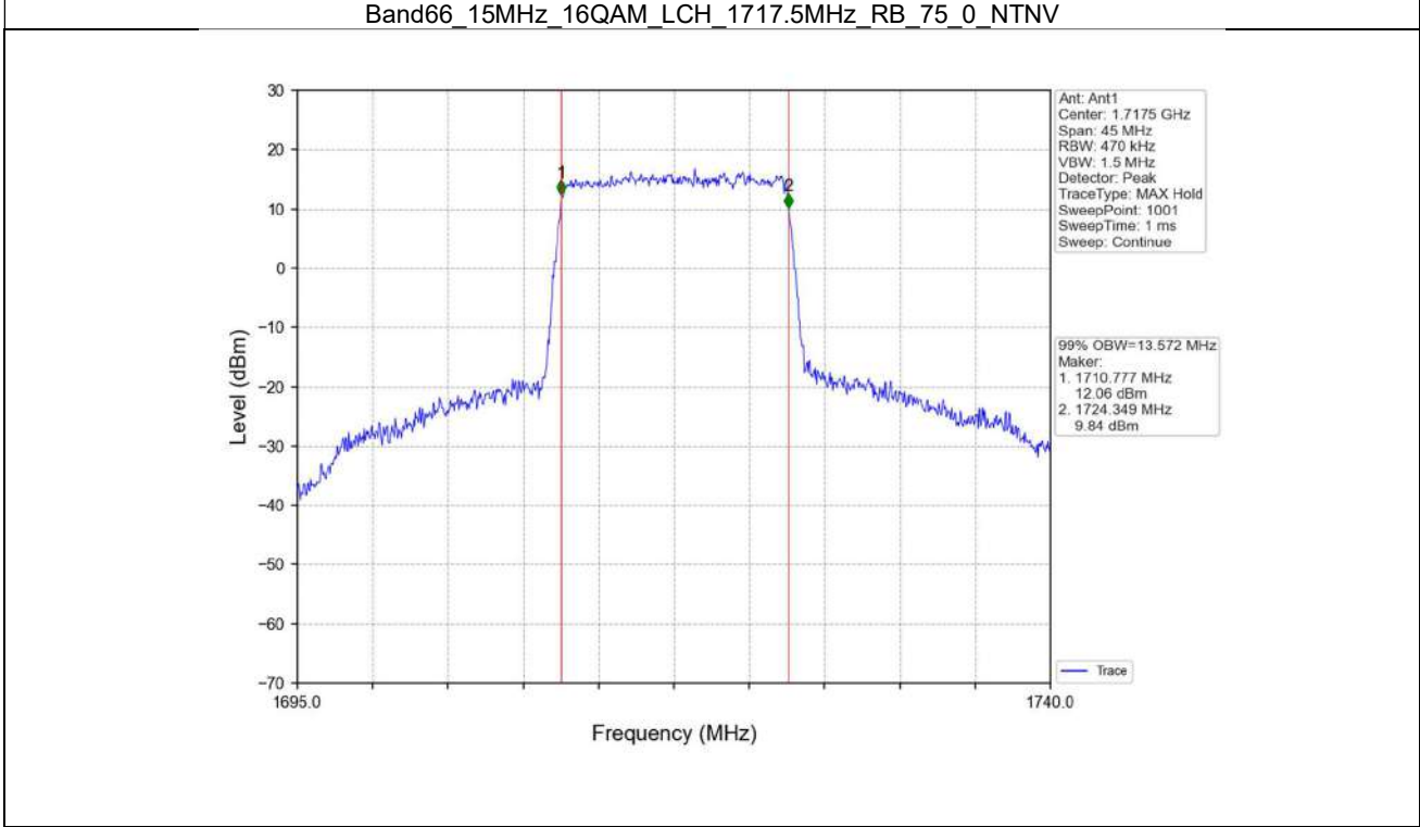
Band66_15MHz_16QAM_LCH_1717.5MHz_RB_75_0_NTNV
