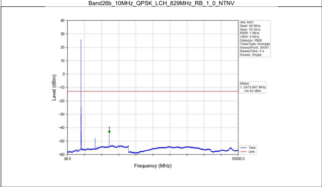
Band26b_10MHz_QPSK_LCH_829MHz_RB_1_0_NTNV
