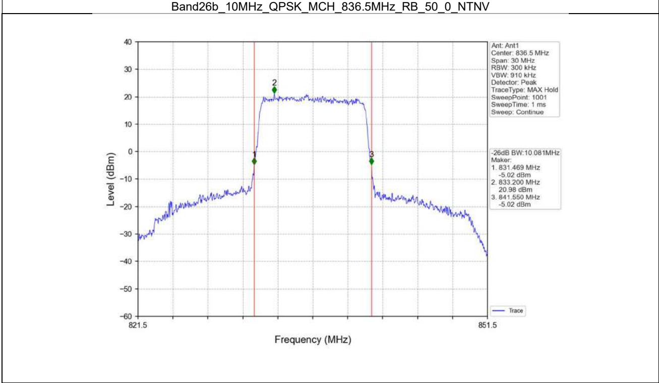
Band26b_10MHz_QPSK_MCH_836.5MHz_RB_50_0_NTNV
