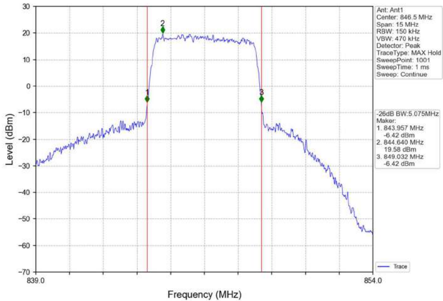
Band26b_5MHz_16QAM_HCH_846.5MHz_RB_25_0_NTNV
