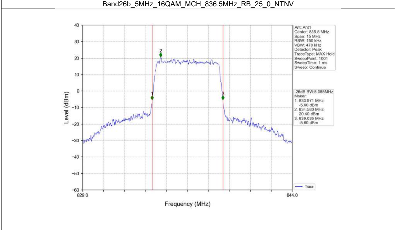
Band26b_5MHz_16QAM_MCH_836.5MHz_RB_25_0_NTNV
