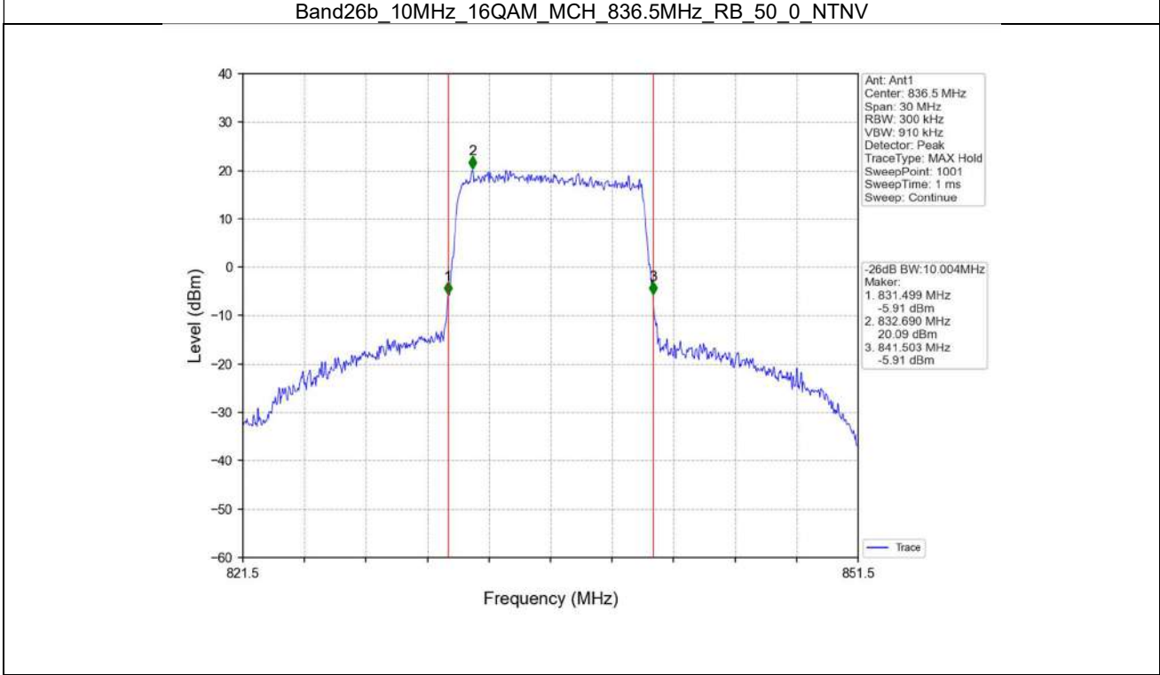
Band26b_10MHz_16QAM_MCH_836.5MHz_RB_50_0_NTNV
