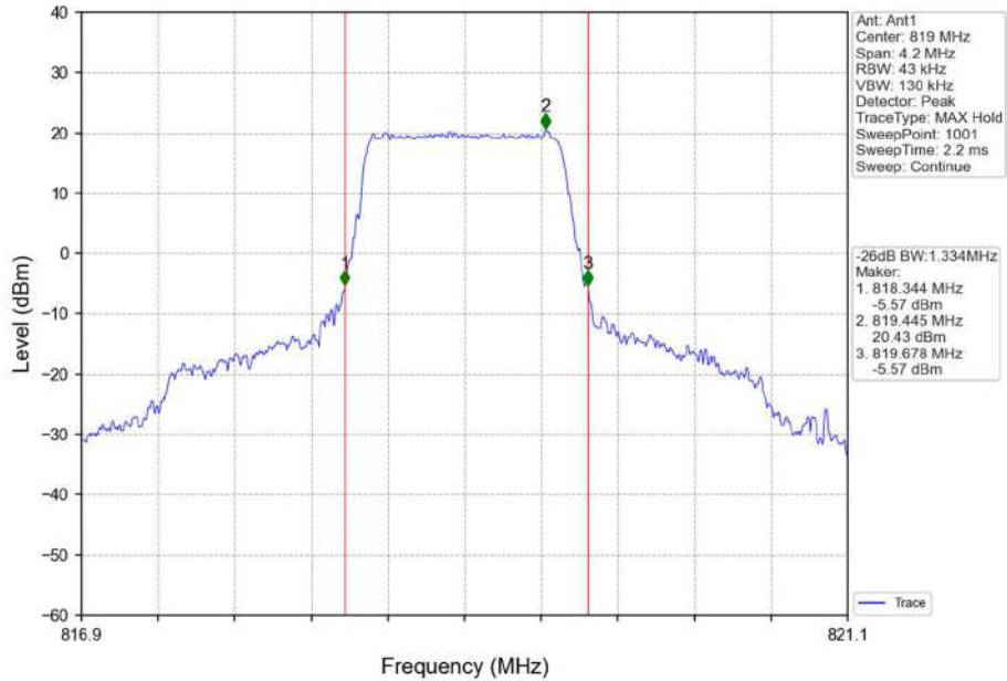
Band26a_1.4MHz_QPSK_MCH_819MHz_RB_6_0_NTNV
