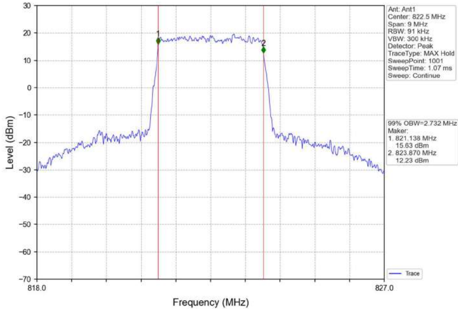
Band26a_3MHz_16QAM_HCH_822.5MHz_RB_15_0_NTNV
