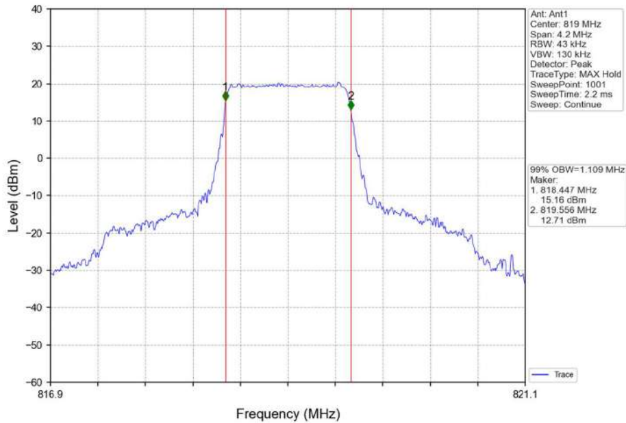
Band26a_1.4MHz_QPSK_MCH_819MHz_RB_6_0_NTNV
