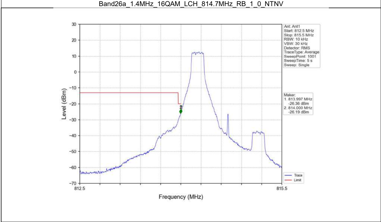
Band26a_1.4MHz_16QAM_LCH_814.7MHz_RB_1_0_NTNV
