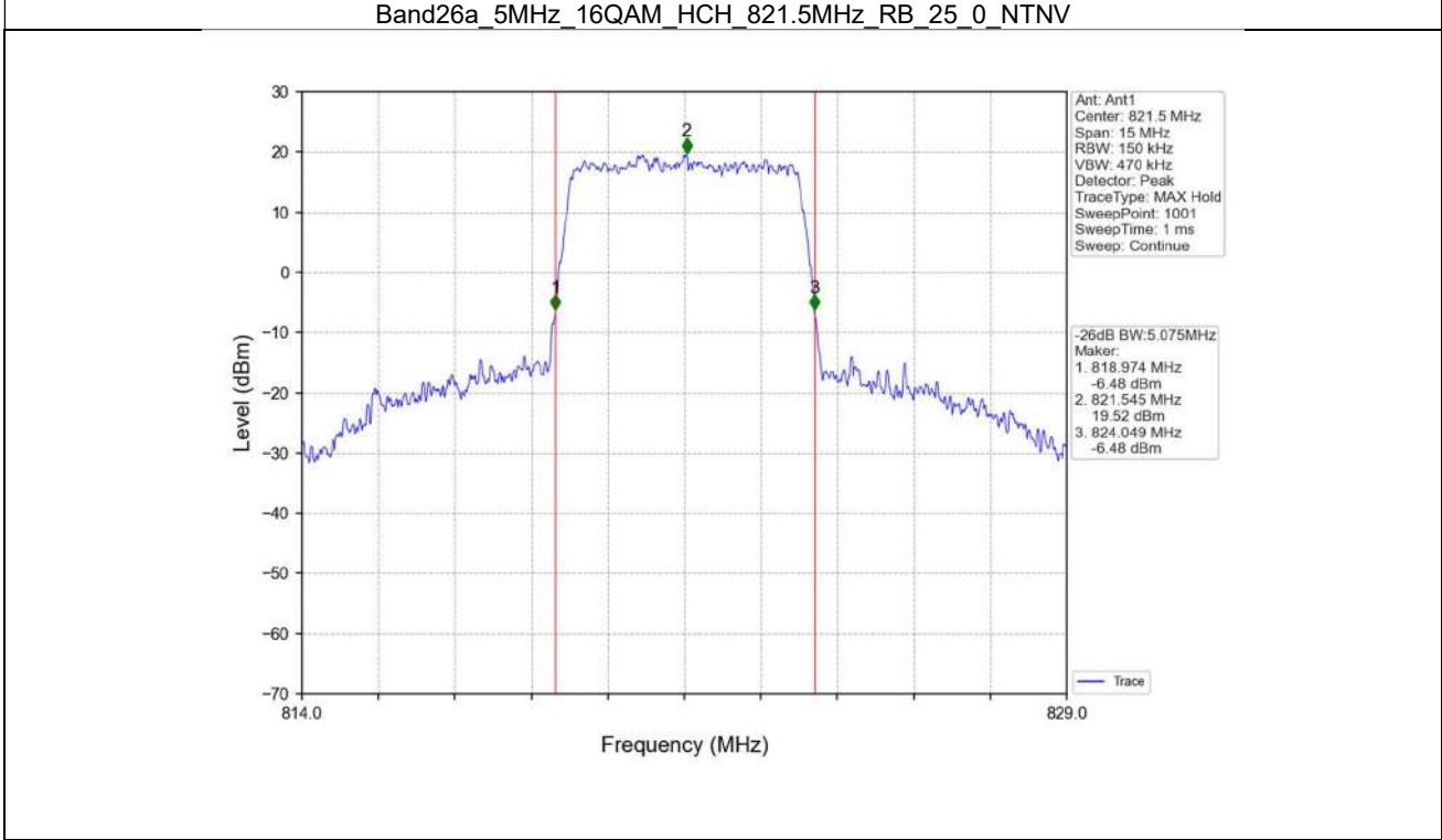
Band26a_5MHz_16QAM_HCH_821.5MHz_RB_25_0_NTNV
