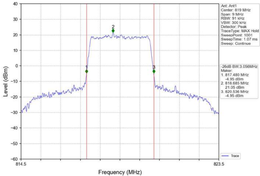
Band26a_3MHz_QPSK_MCH_819MHz_RB_15_0_NTNV
