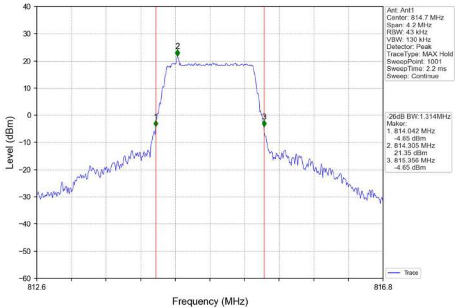
Band26a_1.4MHz_16QAM_LCH_814.7MHz_RB_6_0_NTNV
