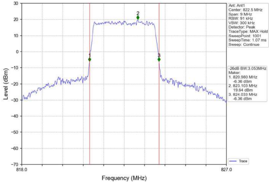
Band26a_3MHz_16QAM_HCH_822.5MHz_RB_15_0_NTNV
