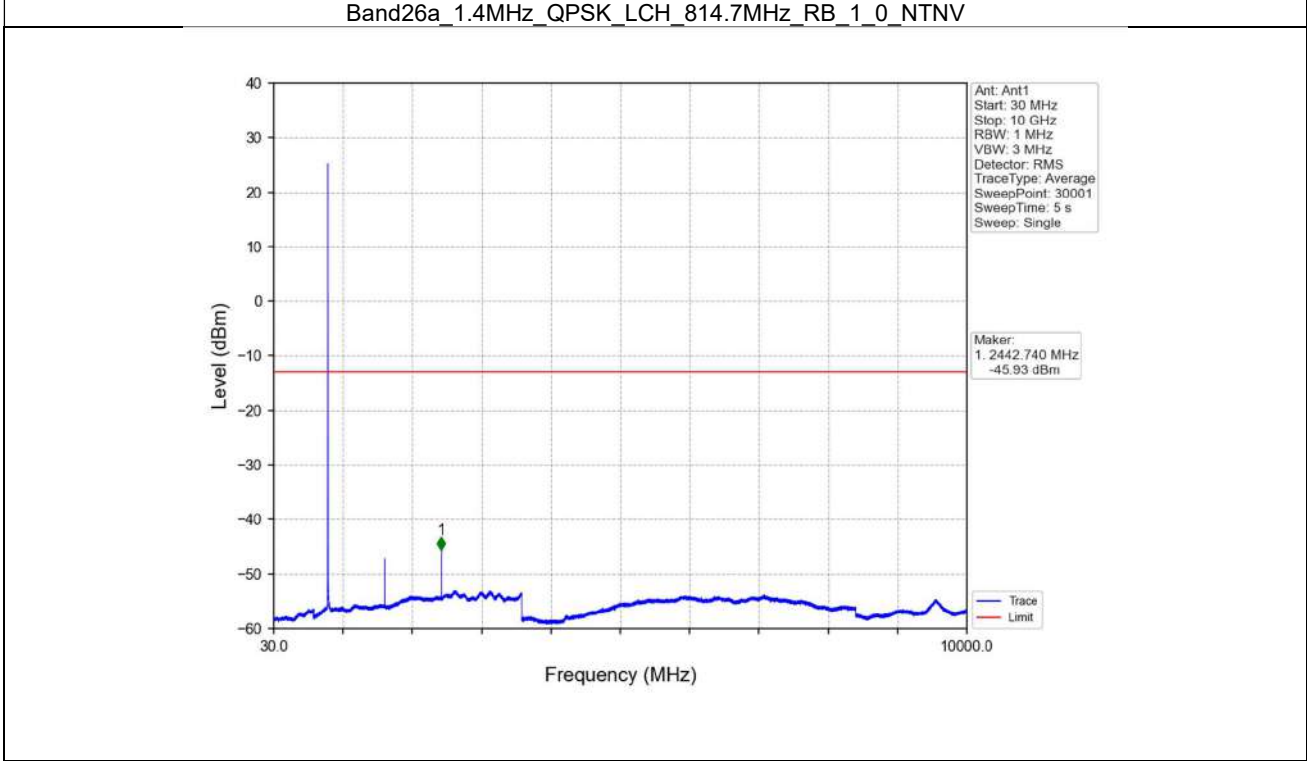
Band26a_1.4MHz_QPSK_LCH_814.7MHz_RB_1_0_NTNV
