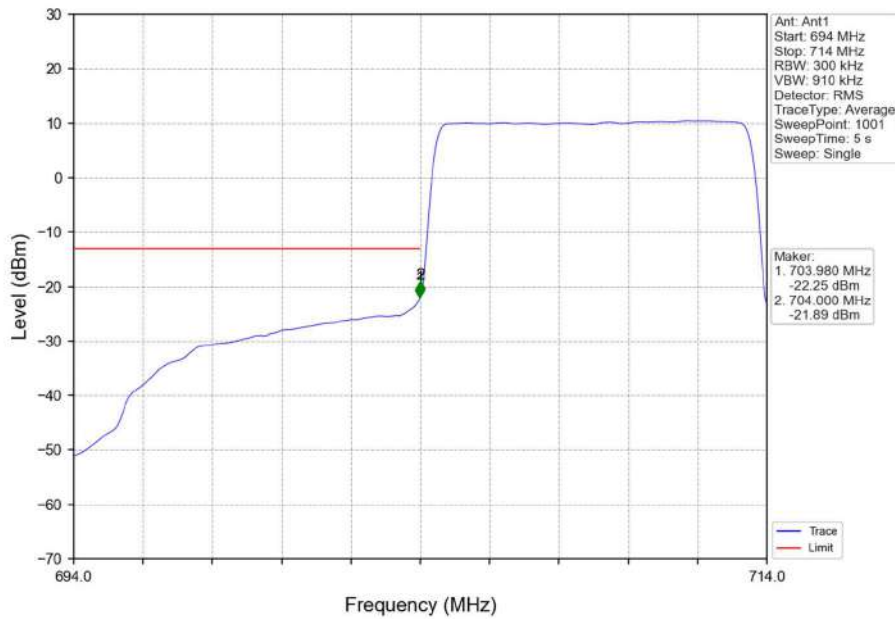
Band17 10MHz QPSK LCH 709MHz RB 50 0 NTN
