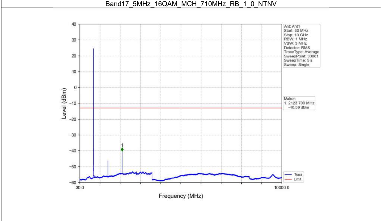
Band17_5MHz_16QAM_MCH_710MHz_RB_1_0_NTNV
