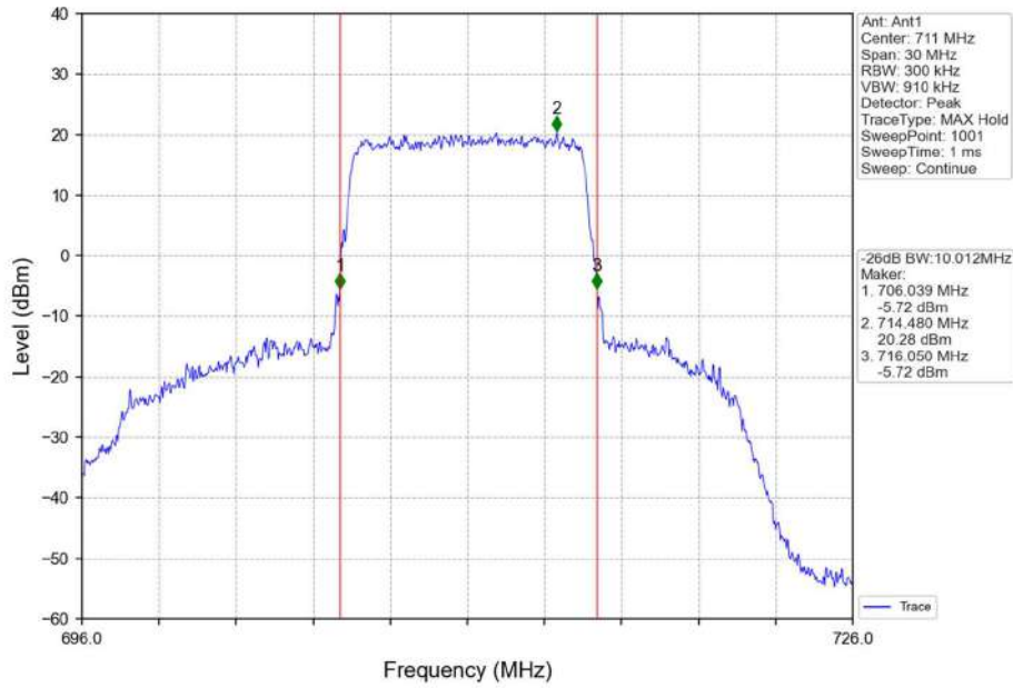
Band17 10MHz QPSK HCH 711MHz RB 50 0 NTN
