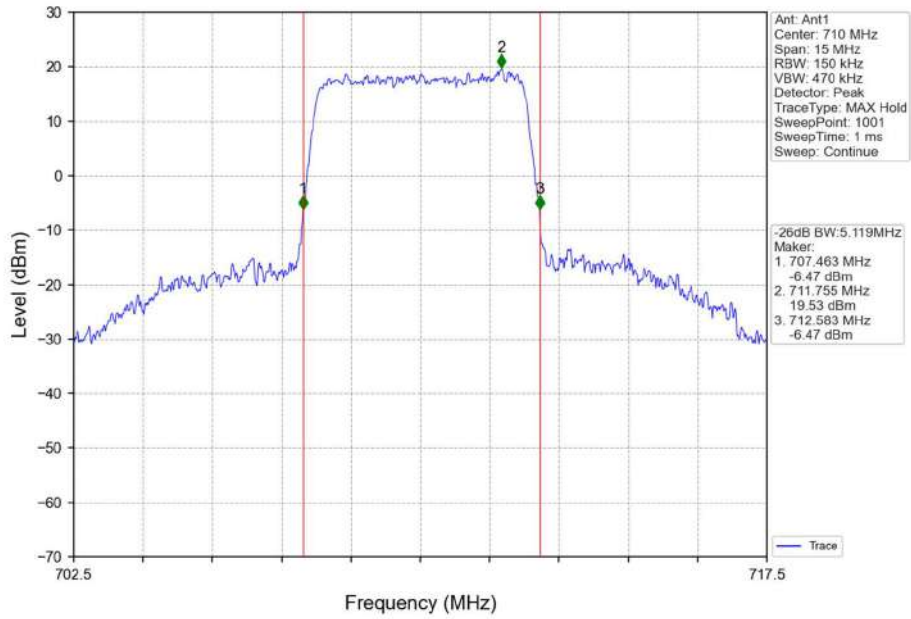
Band17 5MHz 16QAM MCH 710MHz RB 25 0 NTN
