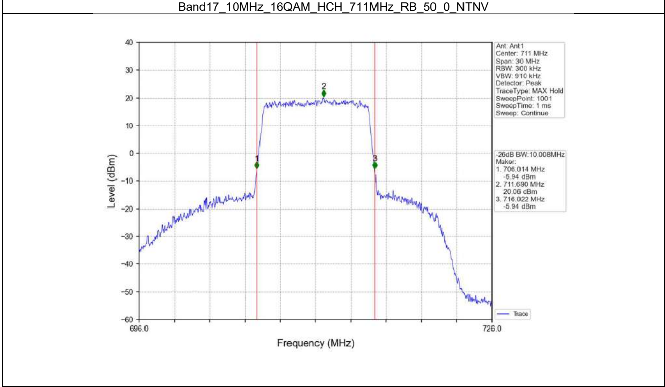
Band17_10MHz_16QAM_HCH_711MHz_RB_50_0_NTNV
