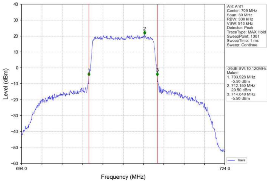
Band17 10MHz QPSK LCH 709MHz RB 50 0 NTN
