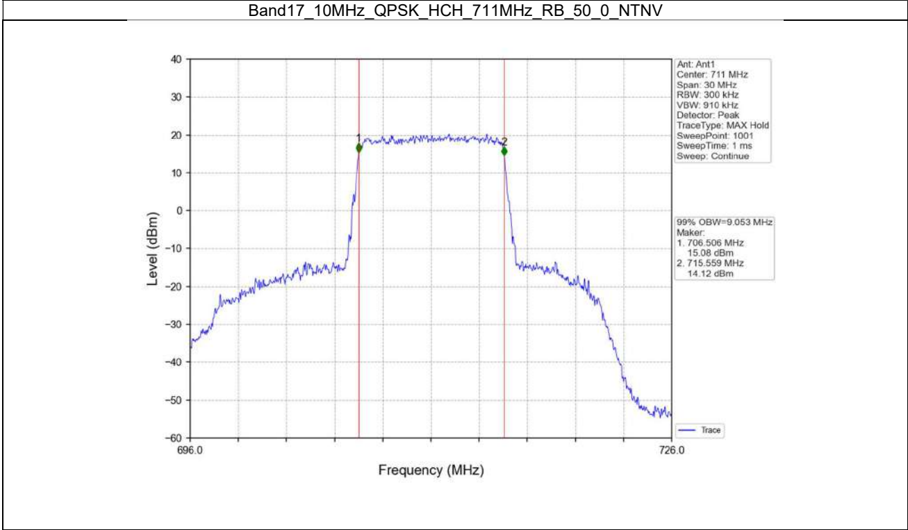
Band17_10MHz_QPSK_HCH_711MHz_RB_50_0_NTNV
