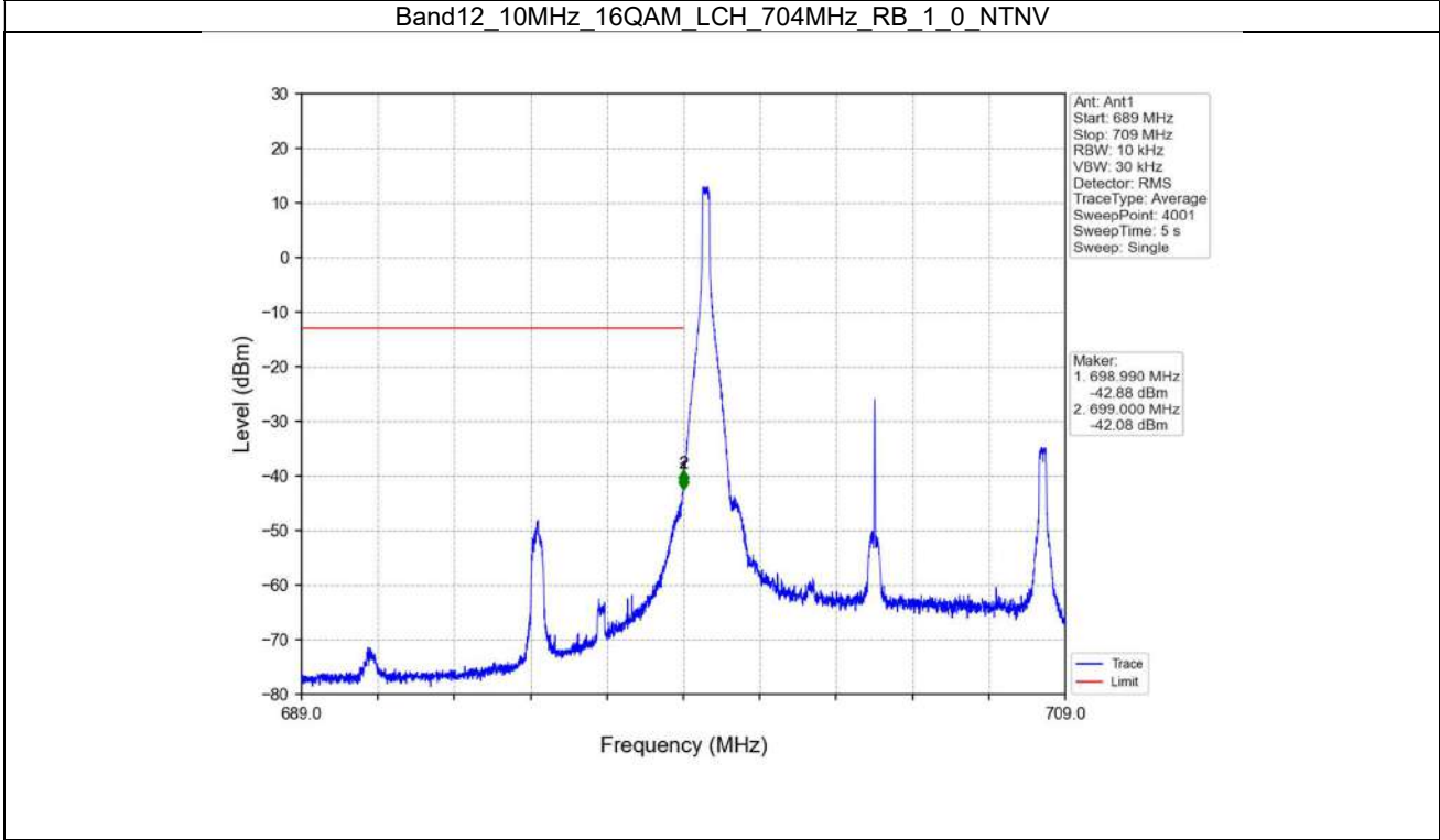
Band12_10MHz_16QAM_LCH_704MHz_RB_1_0_NTNV
