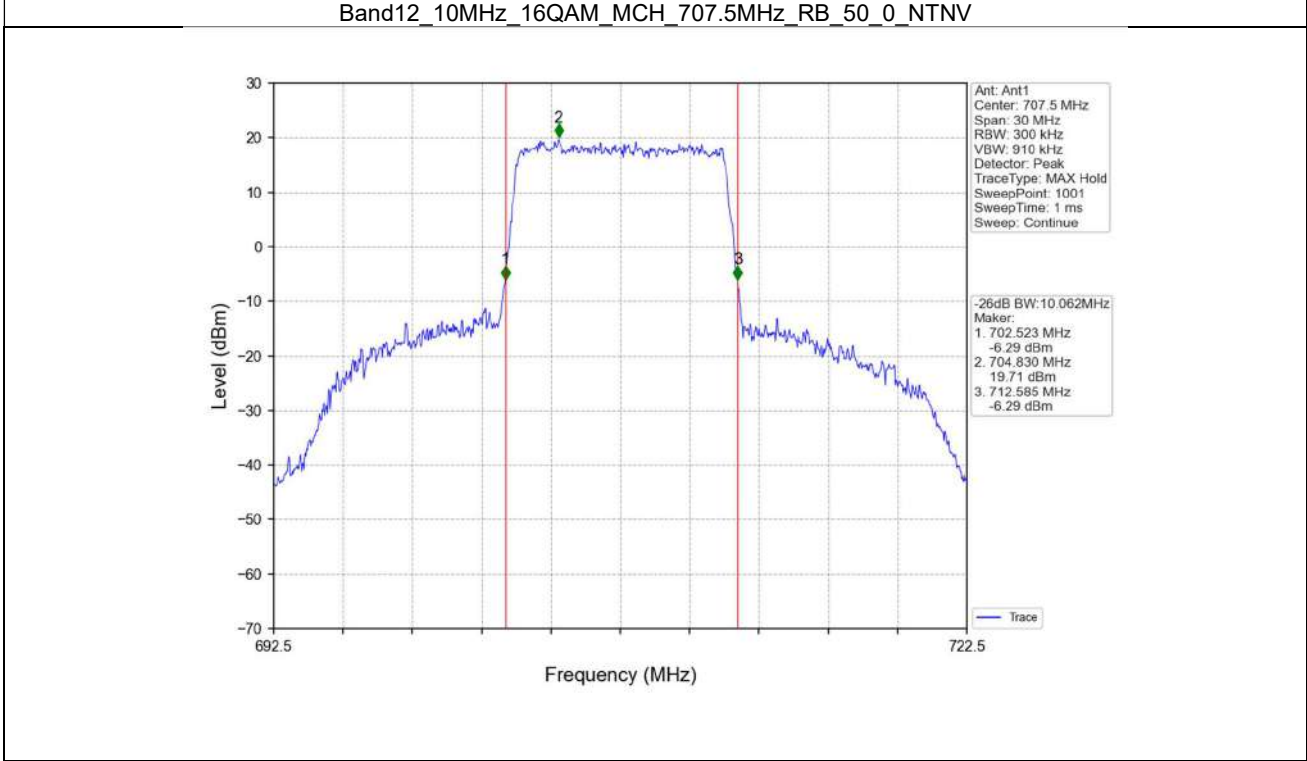
Band12_10MHz_16QAM_MCH_707.5MHz_RB_50_0_NTNV
