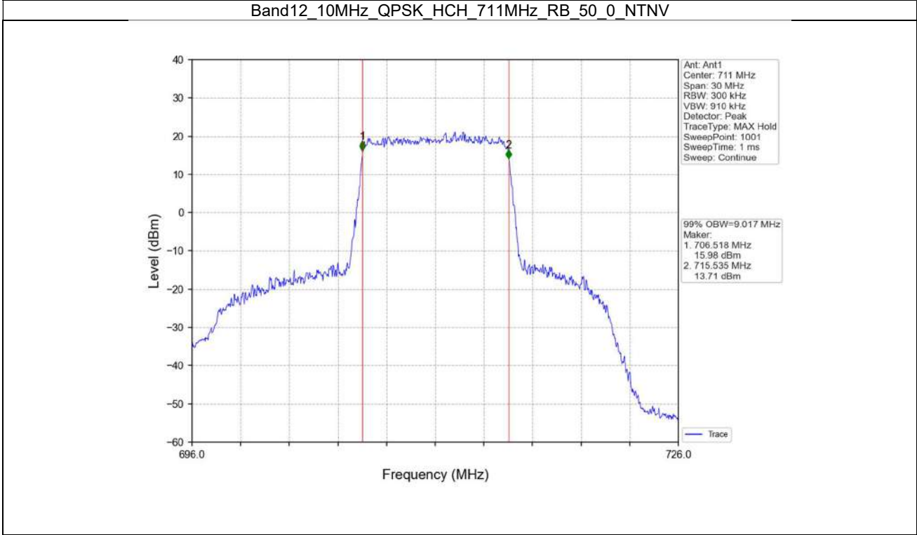
Band12_10MHz_QPSK_HCH_711MHz_RB_50_0_NTNV
