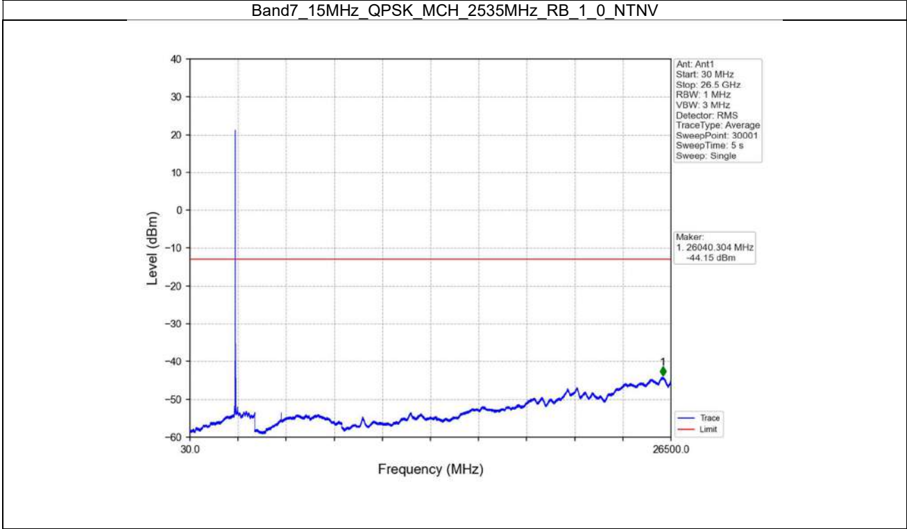
Band7_15MHz_QPSK_MCH_2535MHz_RB_1_0_NTNV
