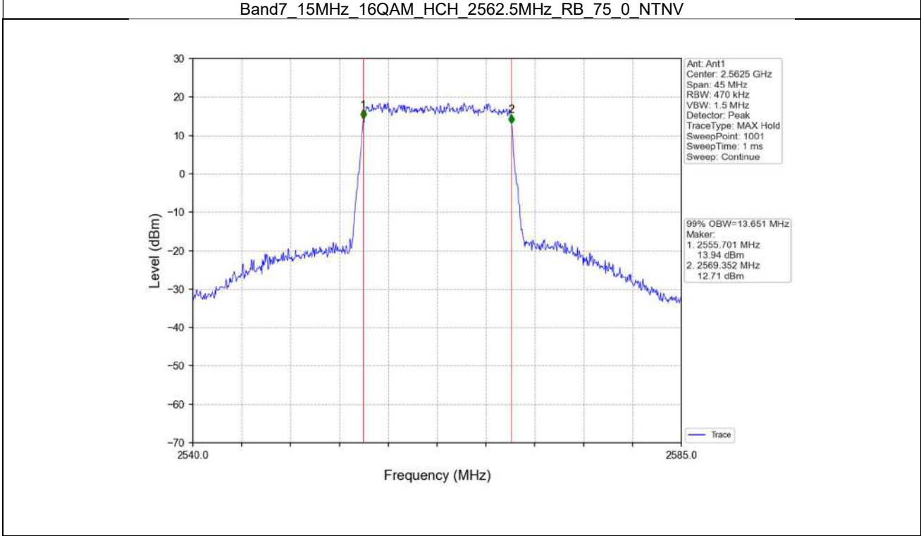
Band7_15MHz_16QAM_HCH_2562.5MHz_RB_75_0_NTNV
