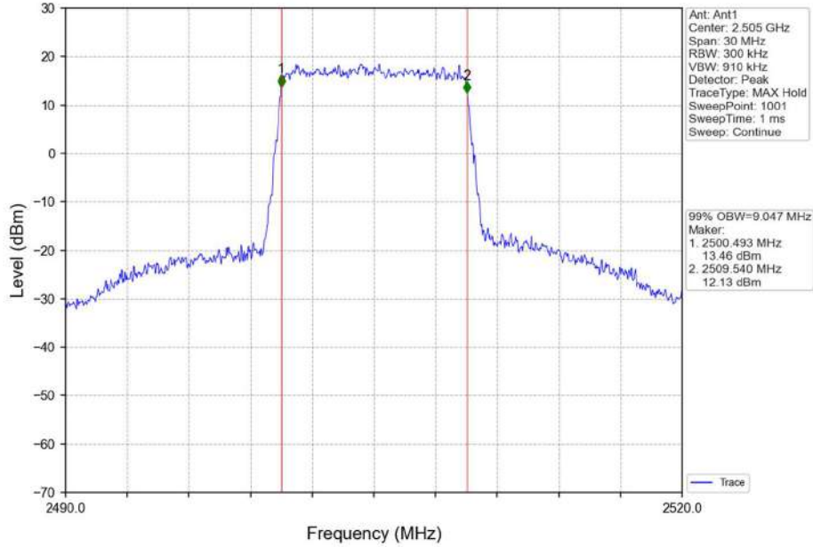
Band7_10MHz_16QAM_LCH_2505MHz_RB_50_0_NTNV
