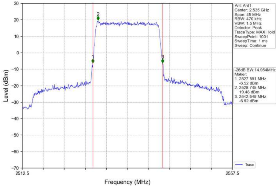
Band7_15MHz_QPSK_MCH_2535MHz_RB_75_0_NTNV
