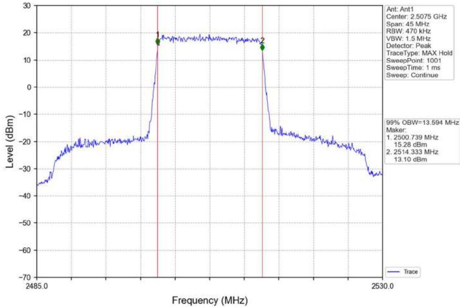
Band7_15MHz_QPSK_LCH_2507.5MHz_RB_75_0_NTNV
