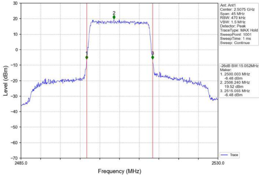
Band7_15MHz_QPSK_LCH_2507.5MHz_RB_75_0_NTNV
