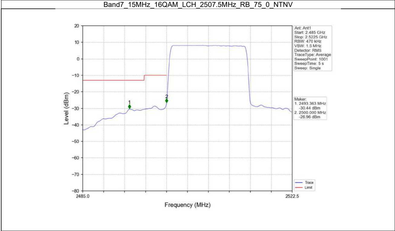
Band7_15MHz_16QAM_LCH_2507.5MHz_RB_75_0_NTNV
