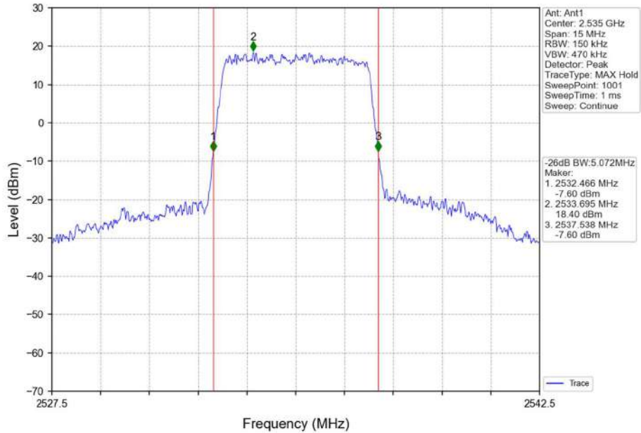
Band7_5MHz_16QAM_MCH_2535MHz_RB_25_0_NTNV
