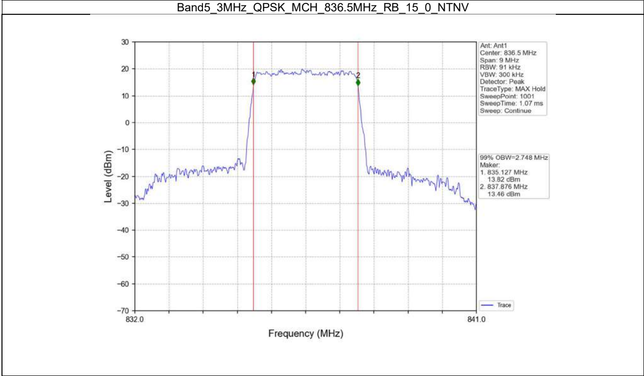
Band5_3MHz_QPSK_MCH_836.5MHz_RB_15_0_NTNV
