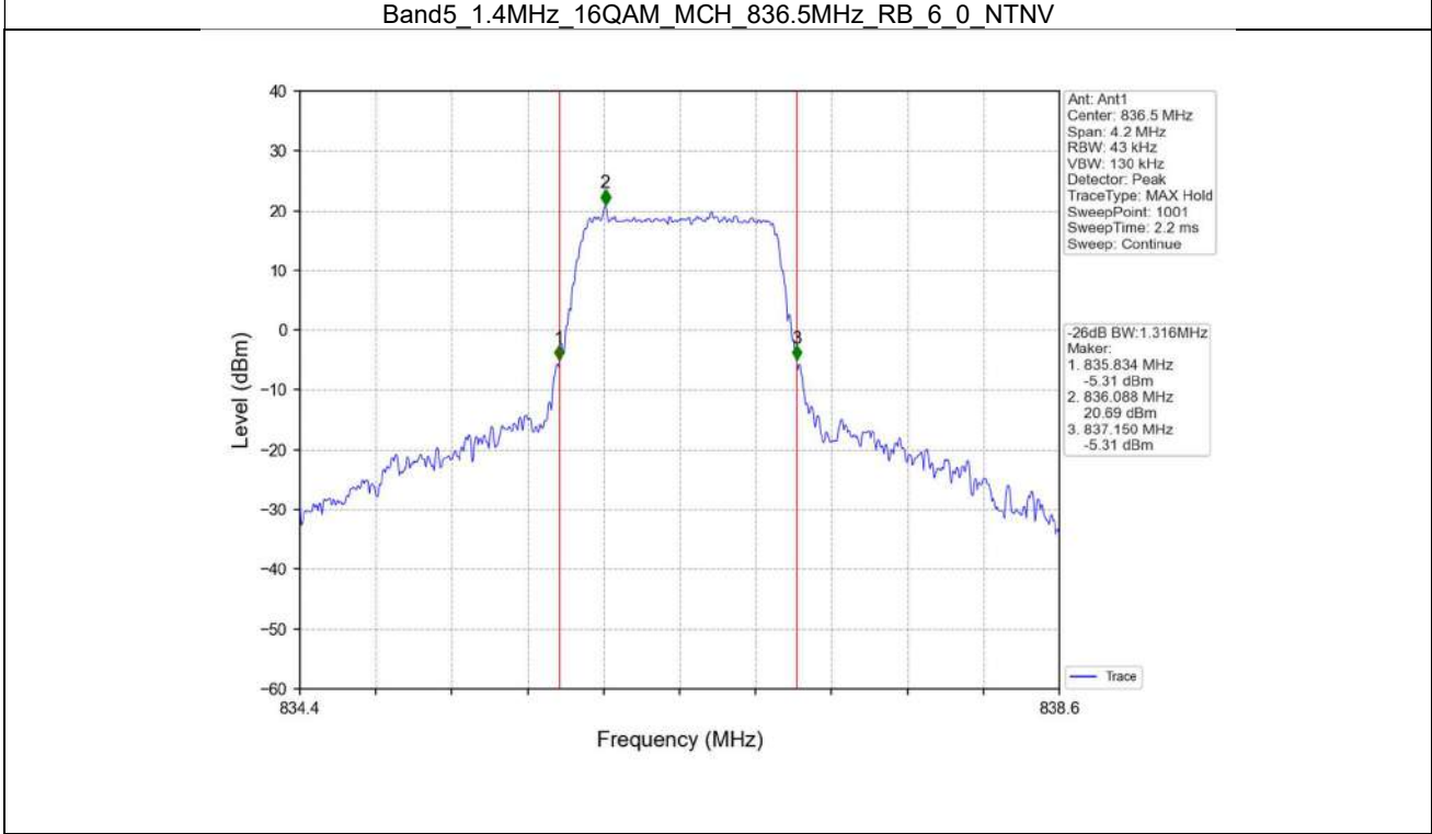
Band5_1.4MHz_16QAM_MCH_836.5MHz_RB_6_0_NTNV
