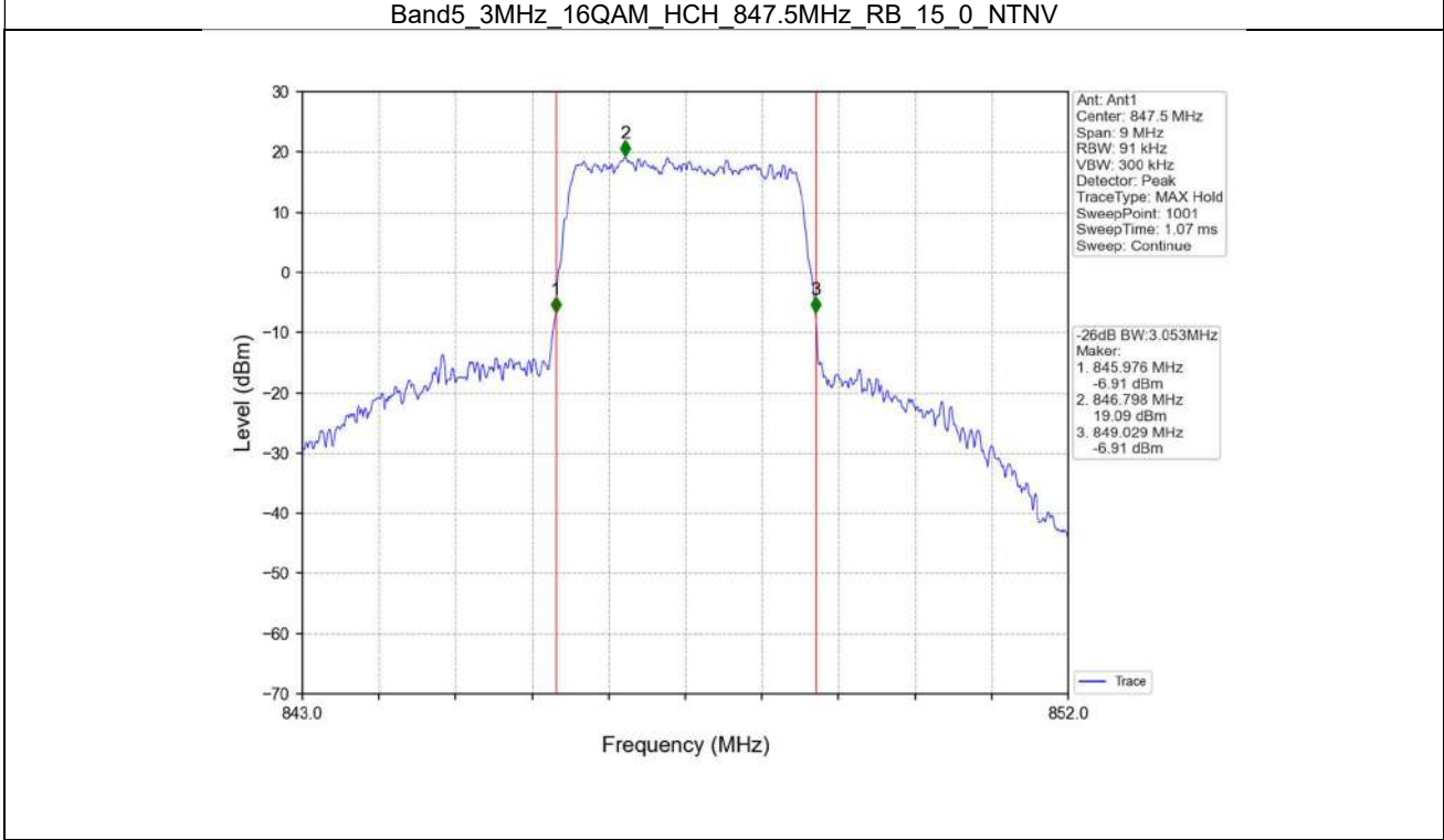
Band5_3MHz_16QAM_HCH_847.5MHz_RB_15_0_NTNV
