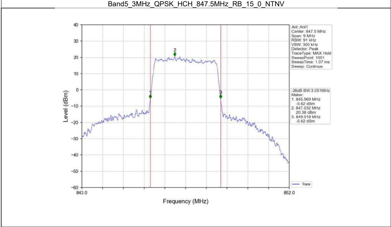
Band5_3MHz_QPSK_HCH_847.5MHz_RB_15_0_NTNV
